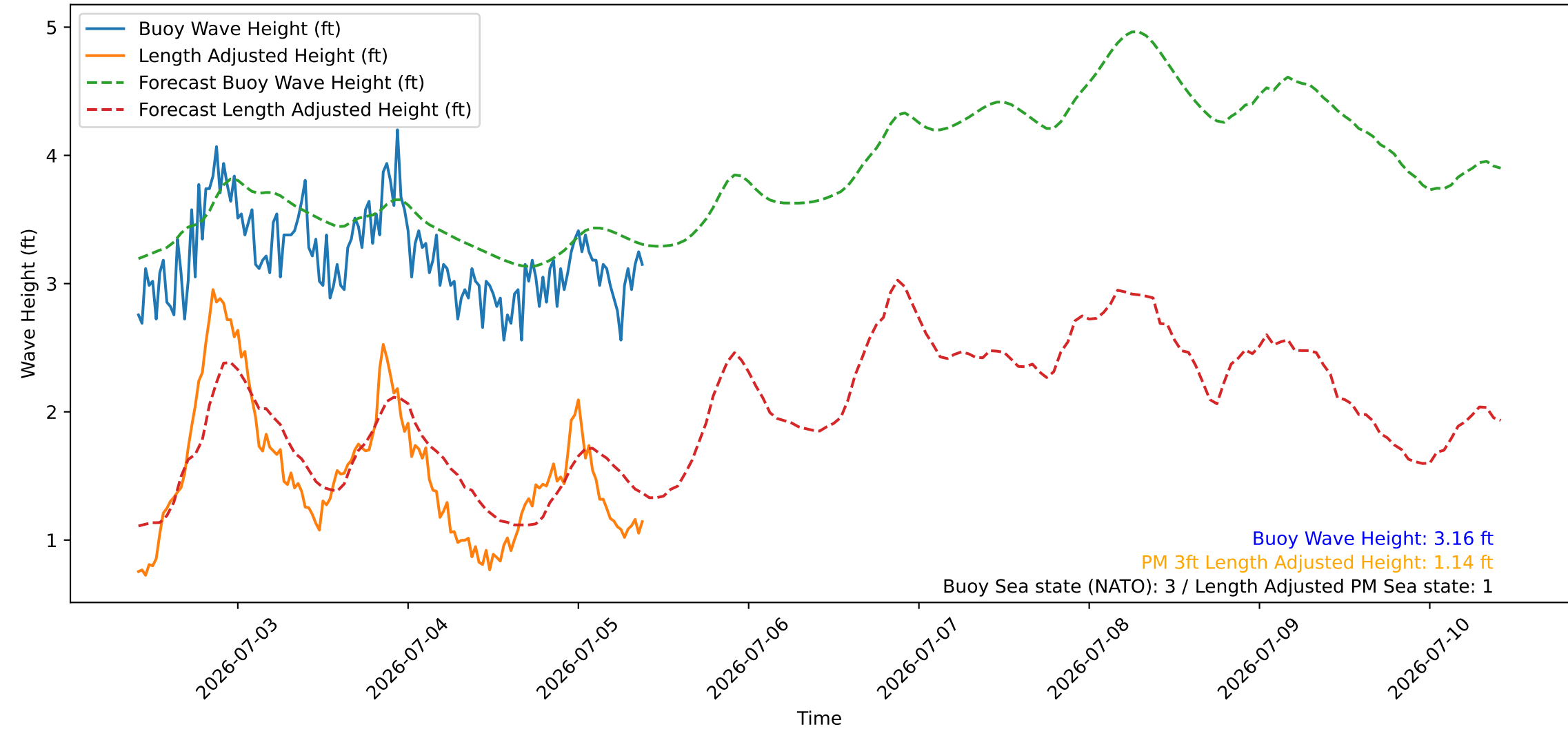
Wave Heights over Time for Green Beach at 2026-07-05 09:51:10
