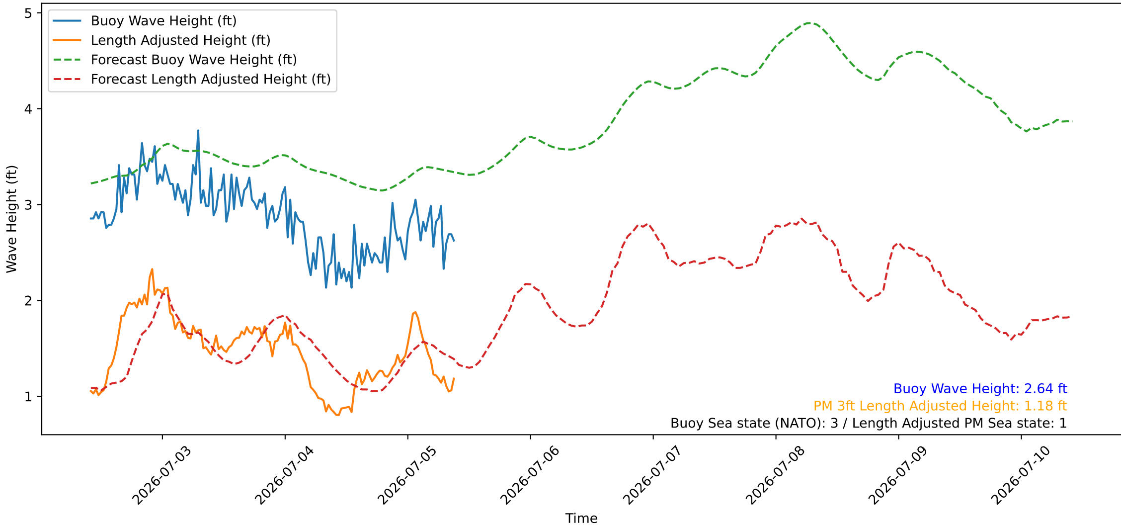
Wave Heights over Time for Oceanside Harbor at 2026-07-05 09:50:26
