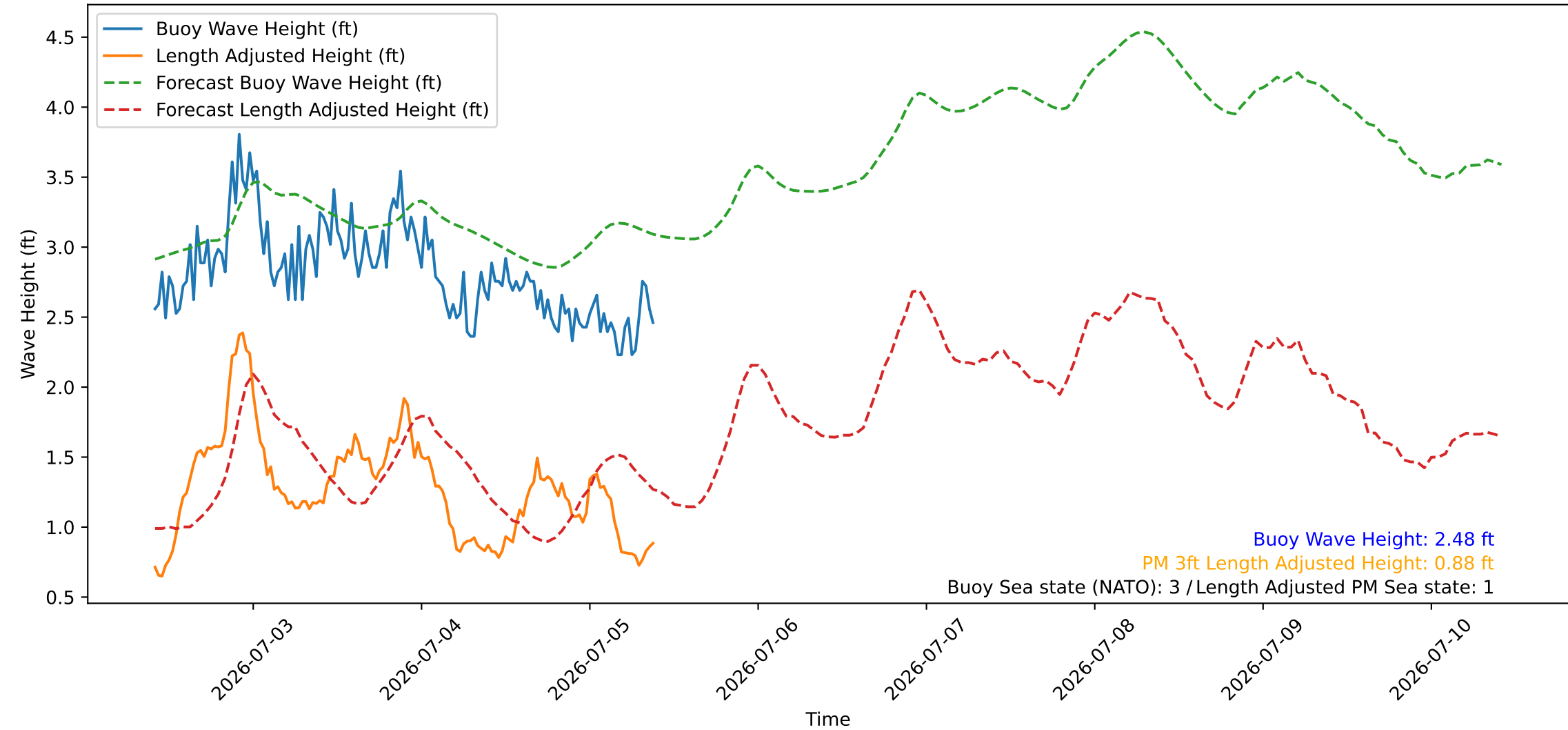
Wave Heights over Time for Red Beach at 2026-07-05 09:50:47
