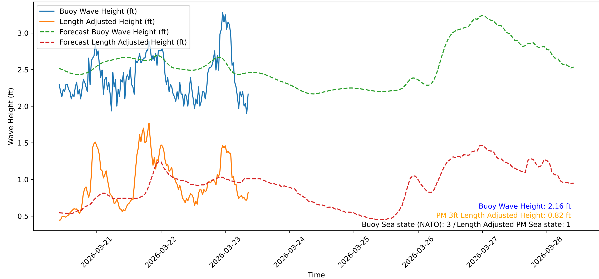
Wave Heights over Time for Green Beach at 2026-03-23 09:51:11
