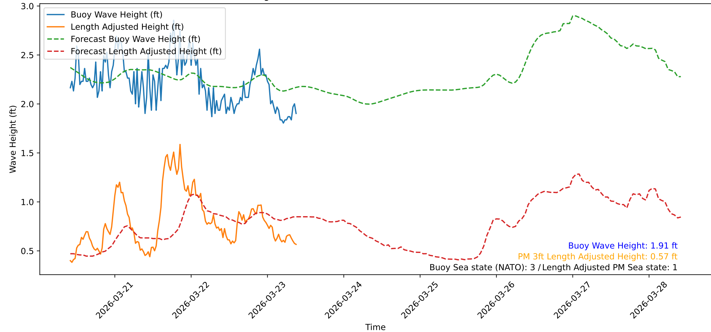
Wave Heights over Time for Red Beach at 2026-03-23 09:50:49
