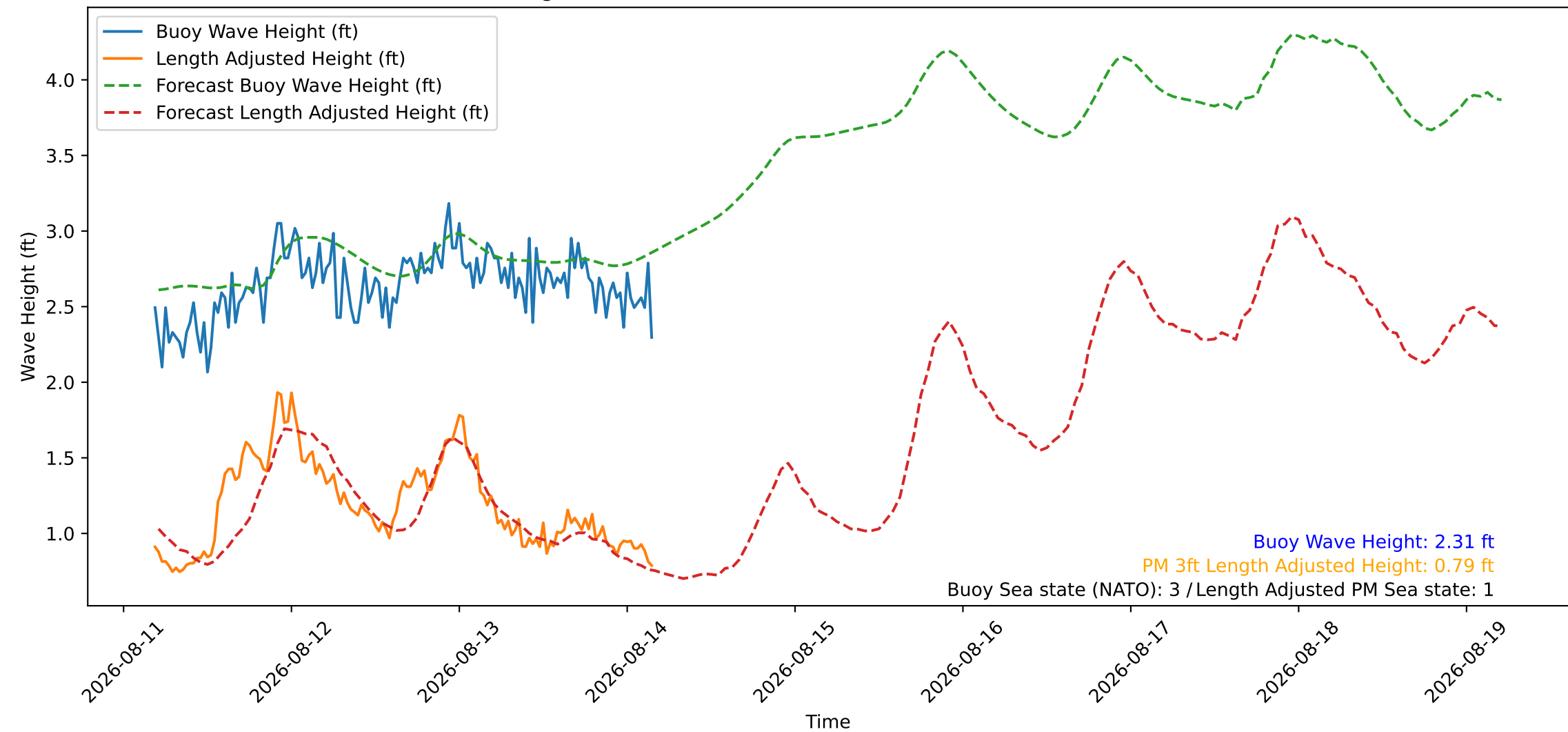
Wave Heights over Time for Oceanside Harbor at 2026-08-14 04:30:27
