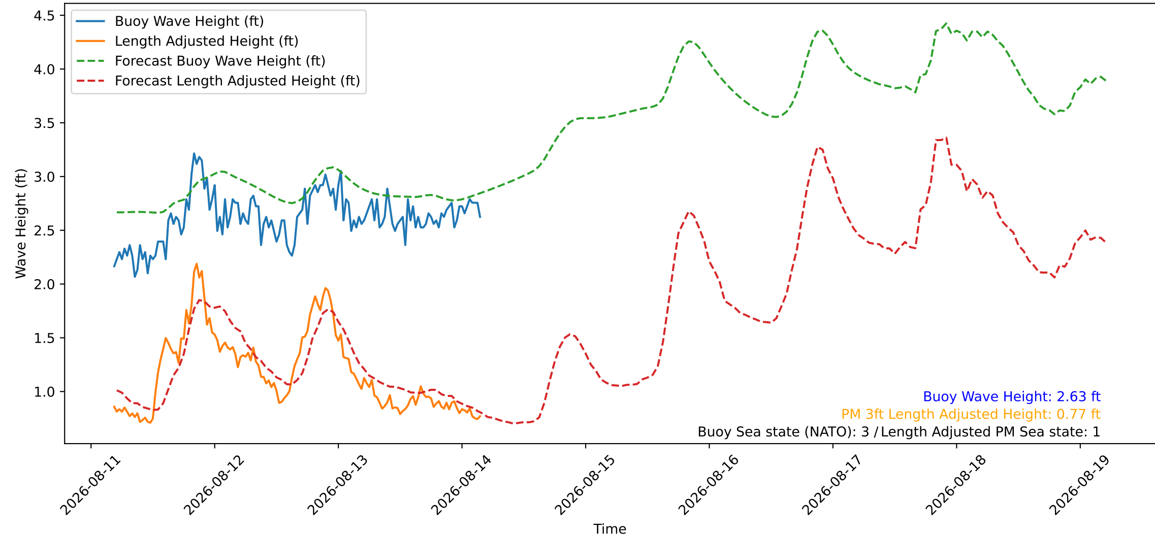
Wave Heights over Time for Green Beach at 2026-08-14 04:31:08
