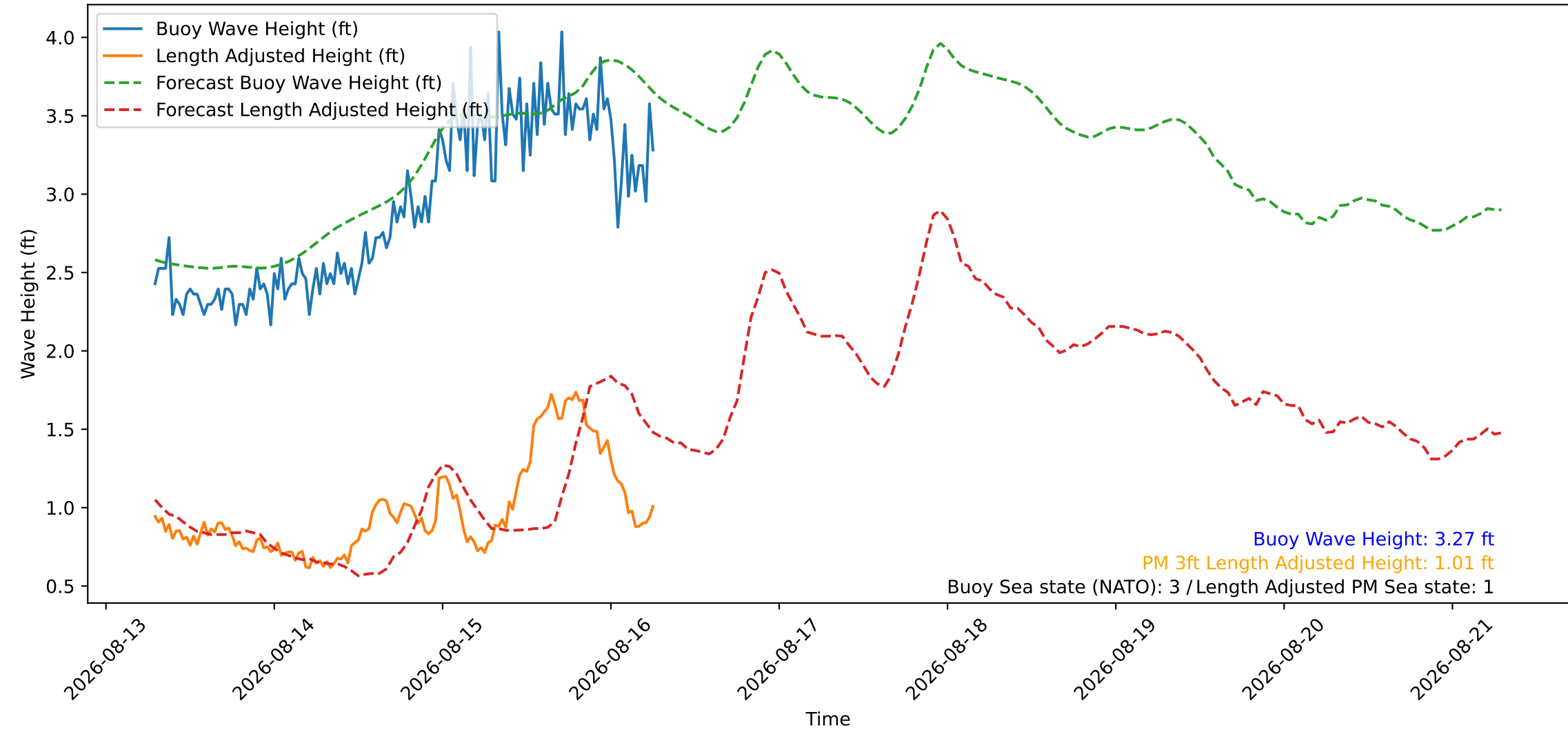
Wave Heights over Time for Red Beach at 2026-08-16 06:40:46
