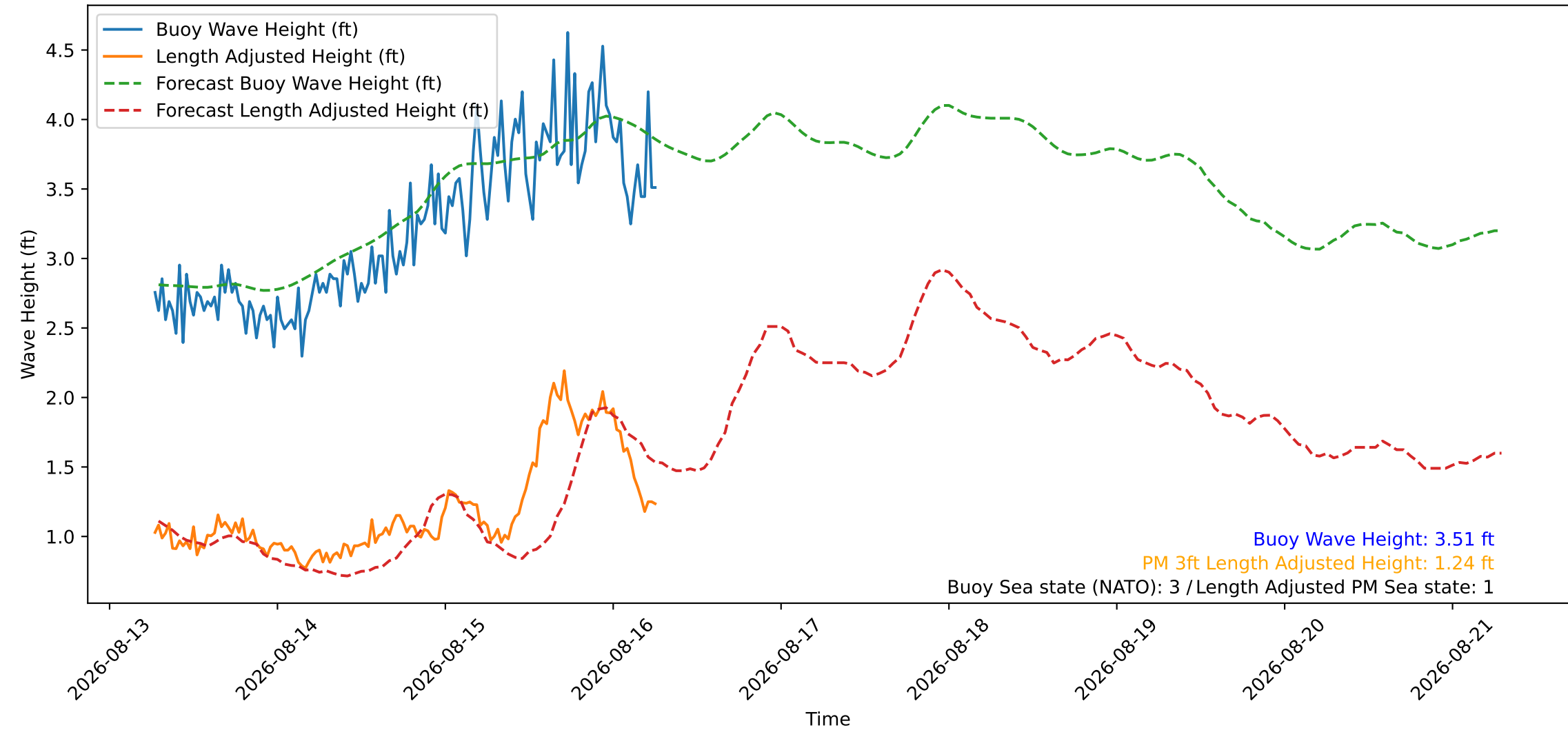
Wave Heights over Time for Oceanside Harbor at 2026-08-16 06:40:26
