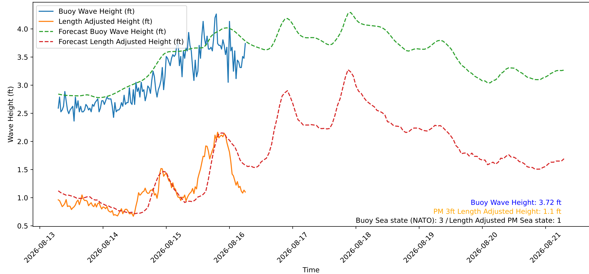
Wave Heights over Time for Green Beach at 2026-08-16 06:41:08
