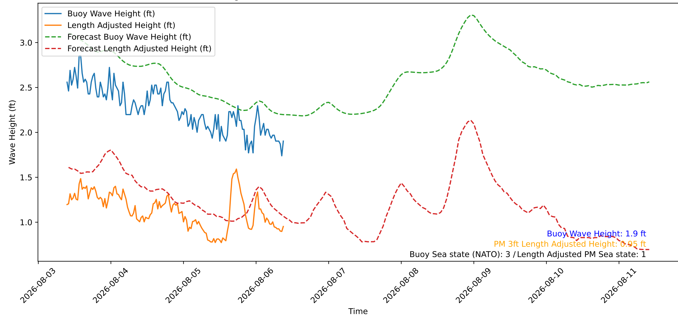
Wave Heights over Time for Oceanside Harbor at 2026-08-06 09:40:26
