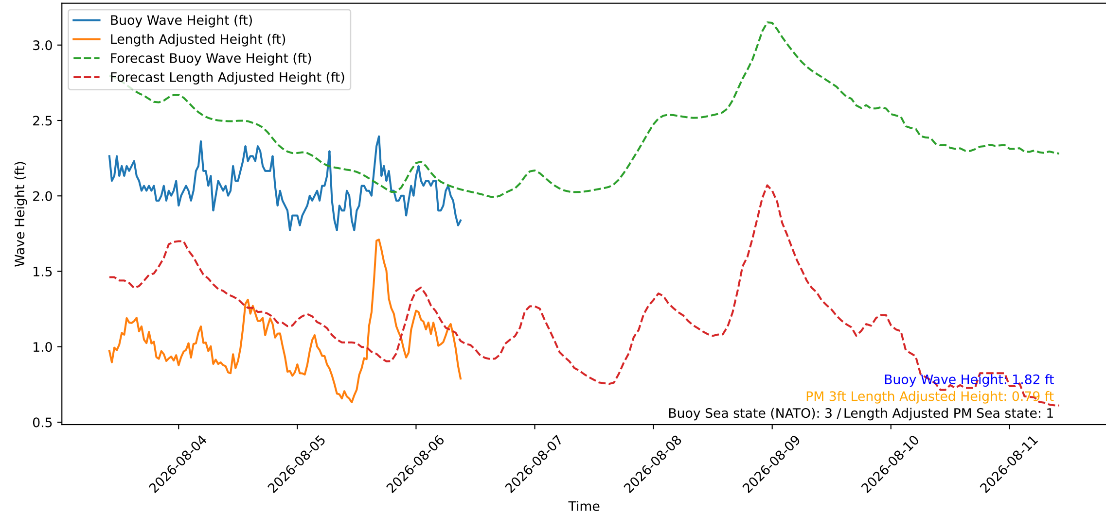
Wave Heights over Time for Red Beach at 2026-08-06 09:40:46
