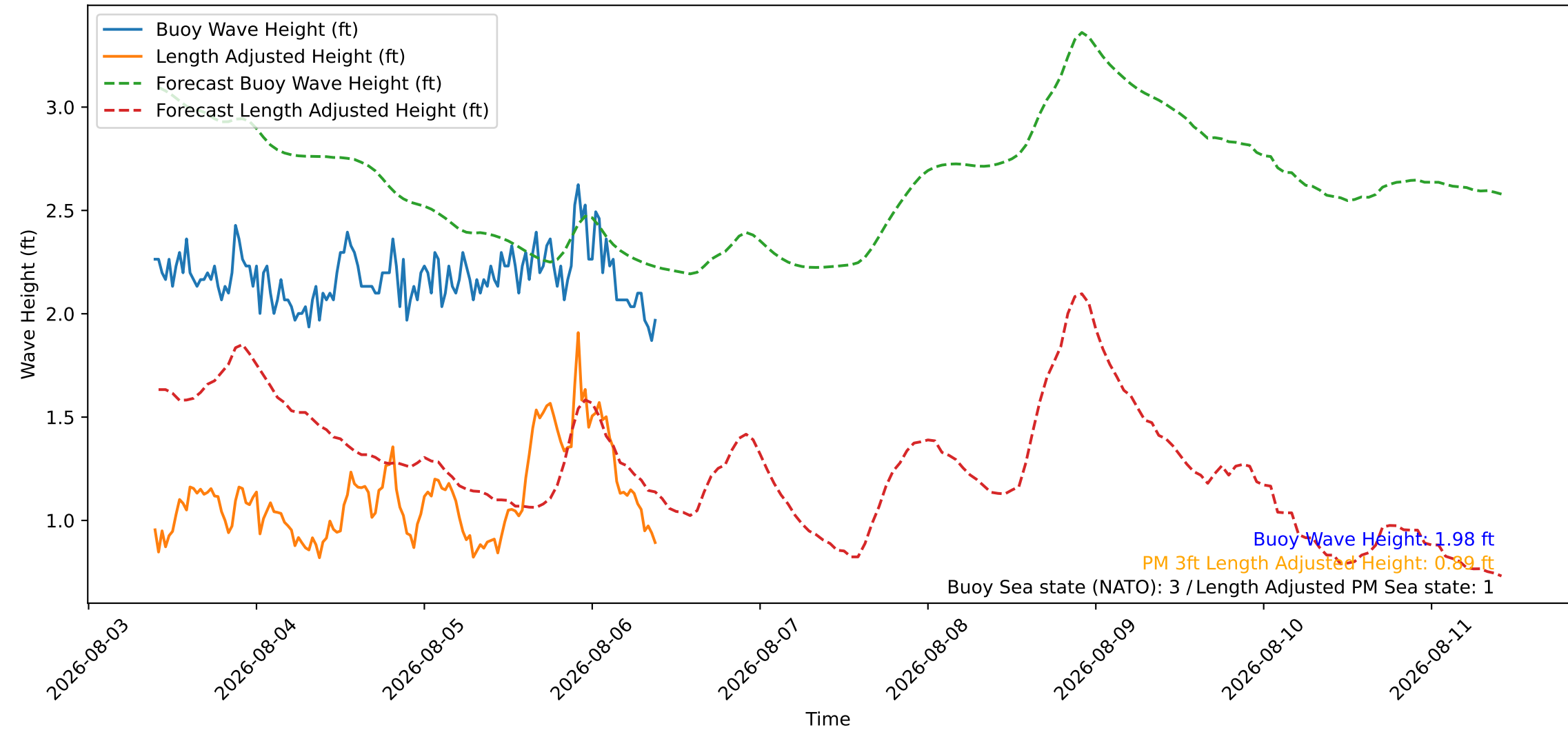
Wave Heights over Time for Green Beach at 2026-08-06 09:41:09
