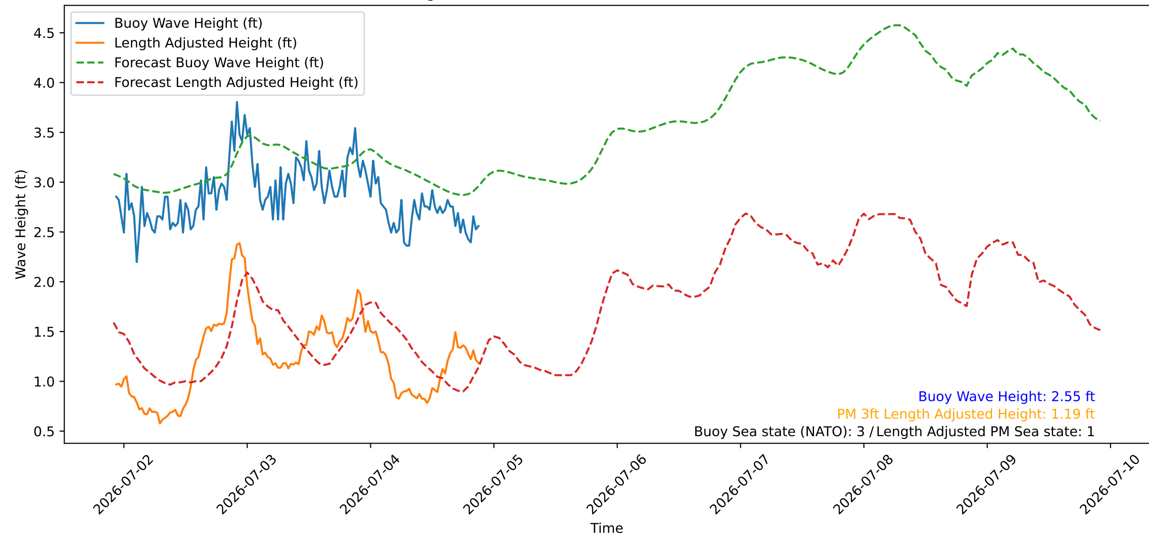
Wave Heights over Time for Red Beach at 2026-07-04 22:00:45
