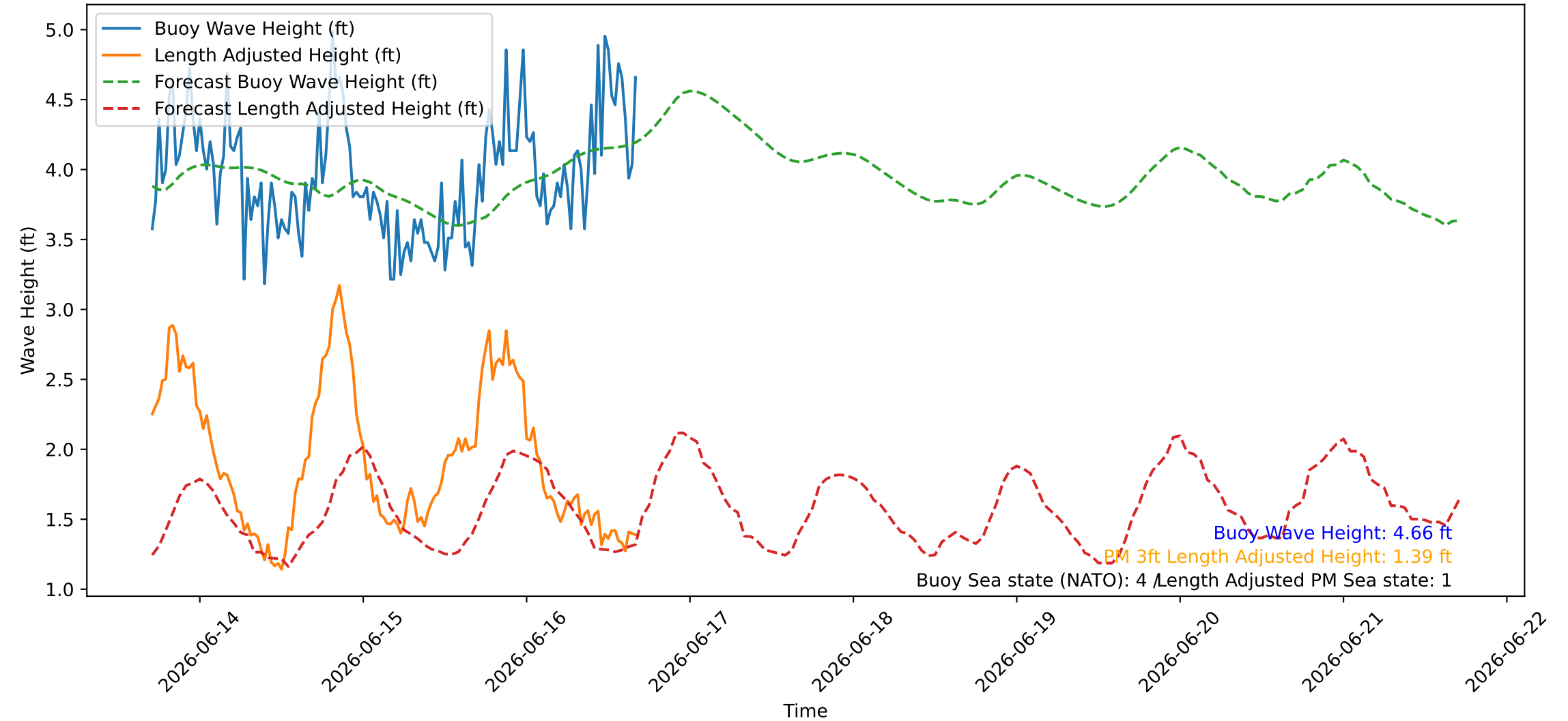
Wave Heights over Time for Oceanside Harbor at 2026-06-16 16:50:27
