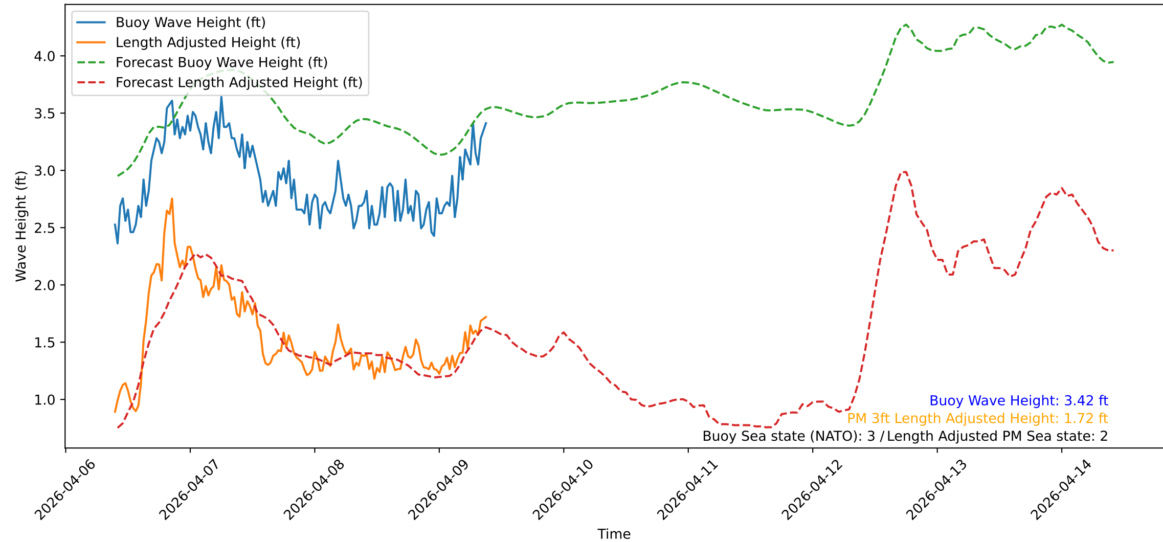
Wave Heights over Time for Oceanside Harbor at 2026-04-09 09:40:31
