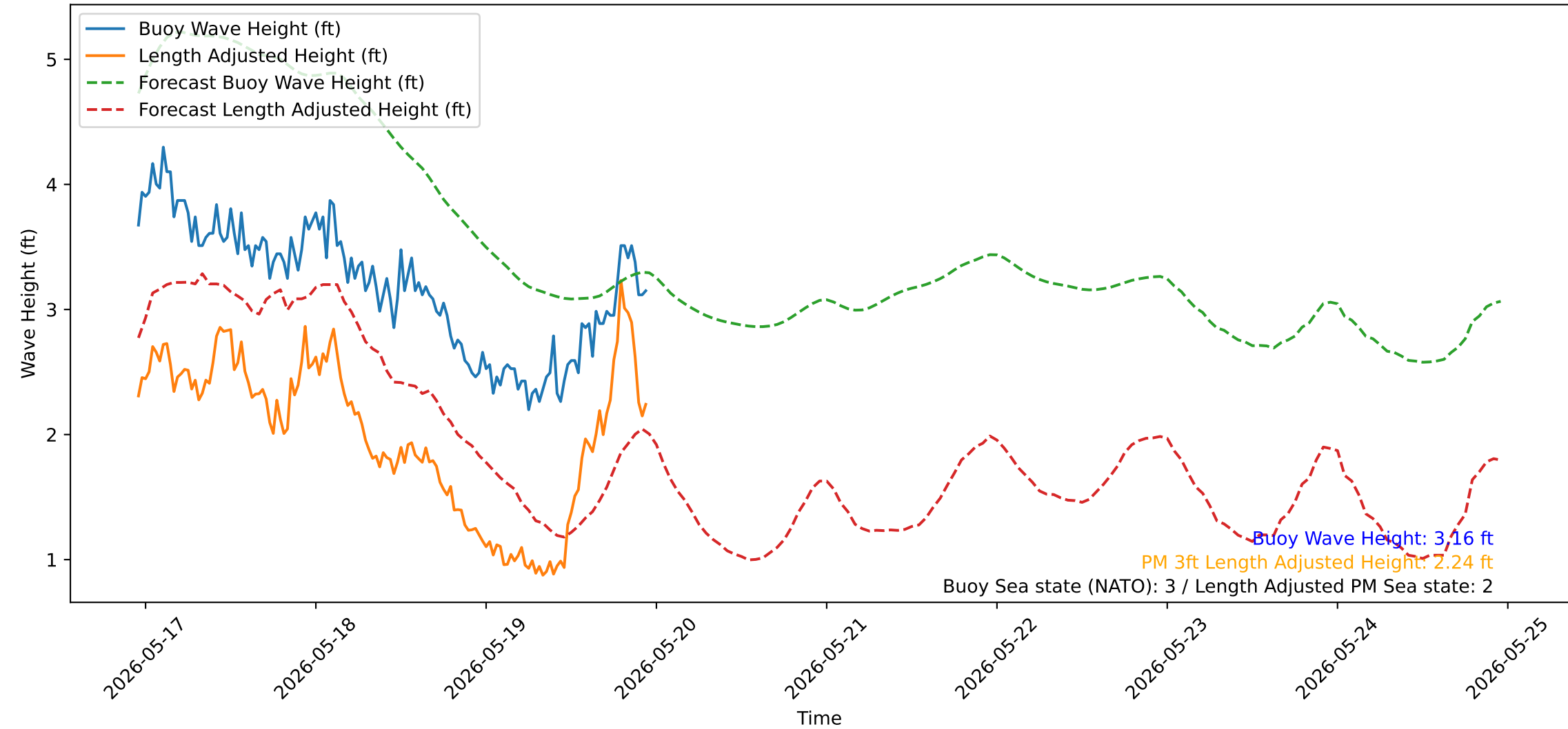
Wave Heights over Time for Oceanside Harbor at 2026-05-19 23:00:32
