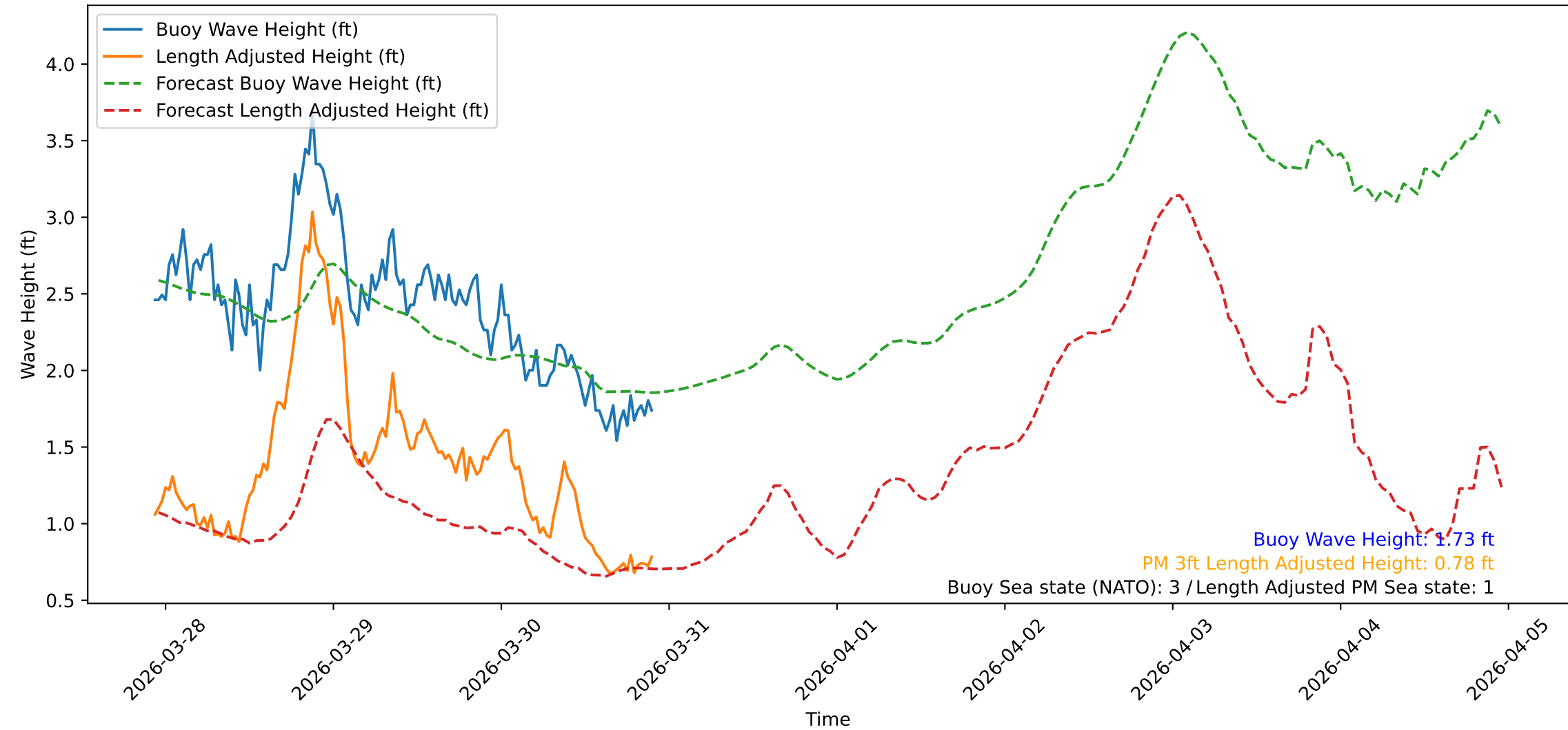
Wave Heights over Time for Green Beach at 2026-03-30 22:31:10
