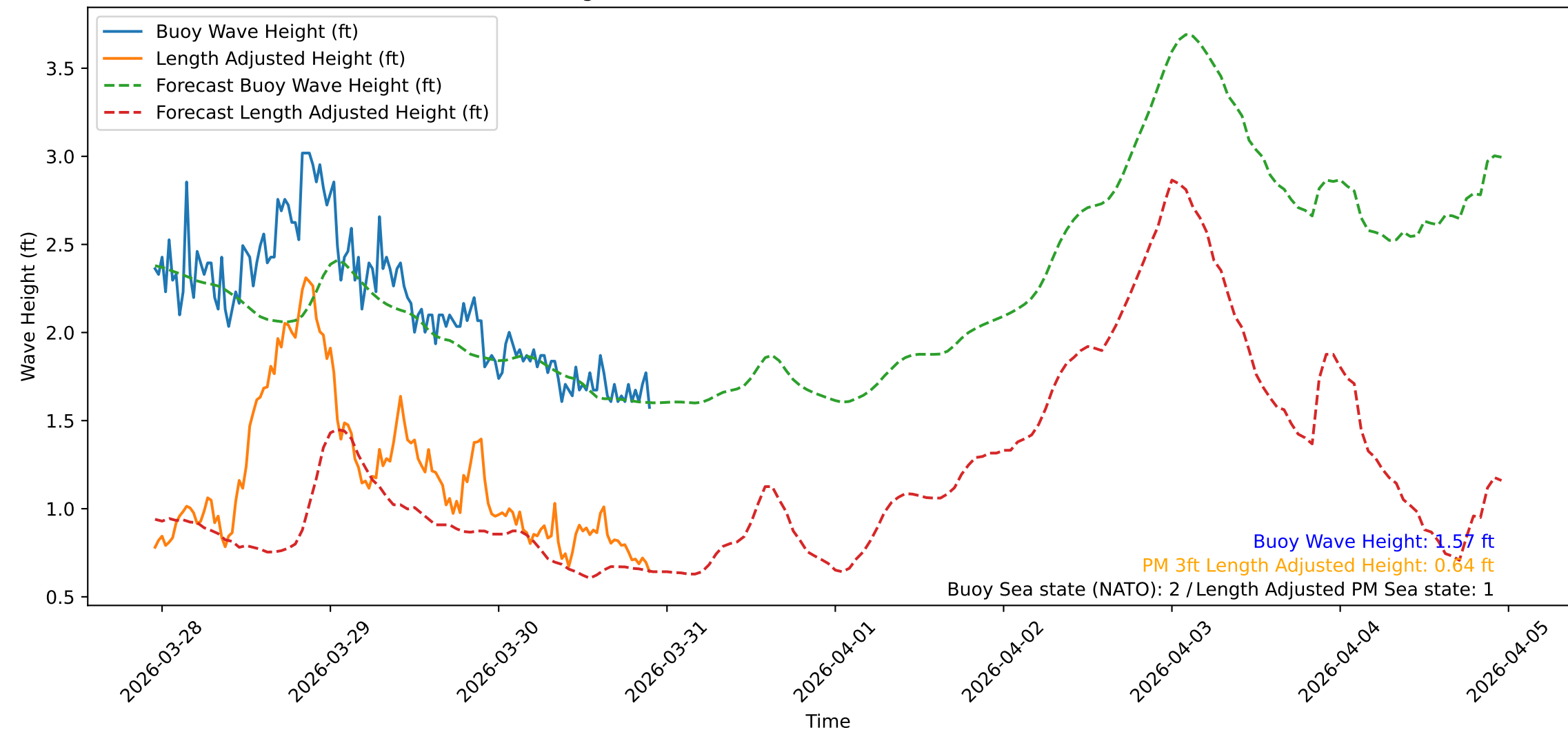
Wave Heights over Time for Red Beach at 2026-03-30 22:30:48
