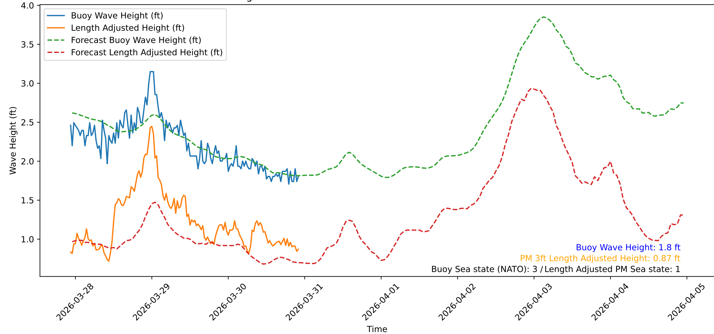
Wave Heights over Time for Oceanside Harbor at 2026-03-30 22:30:32
