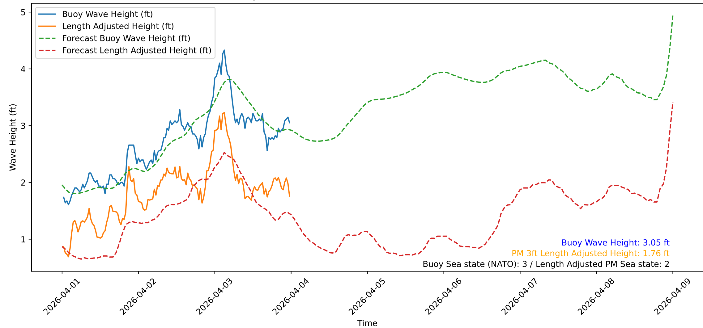
Wave Heights over Time for Green Beach at 2026-04-04 00:21:15
