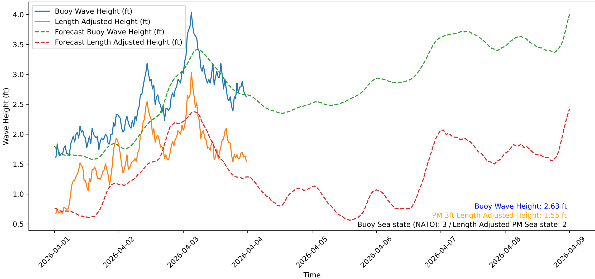
Wave Heights over Time for Oceanside Harbor at 2026-04-04 00:20:33
