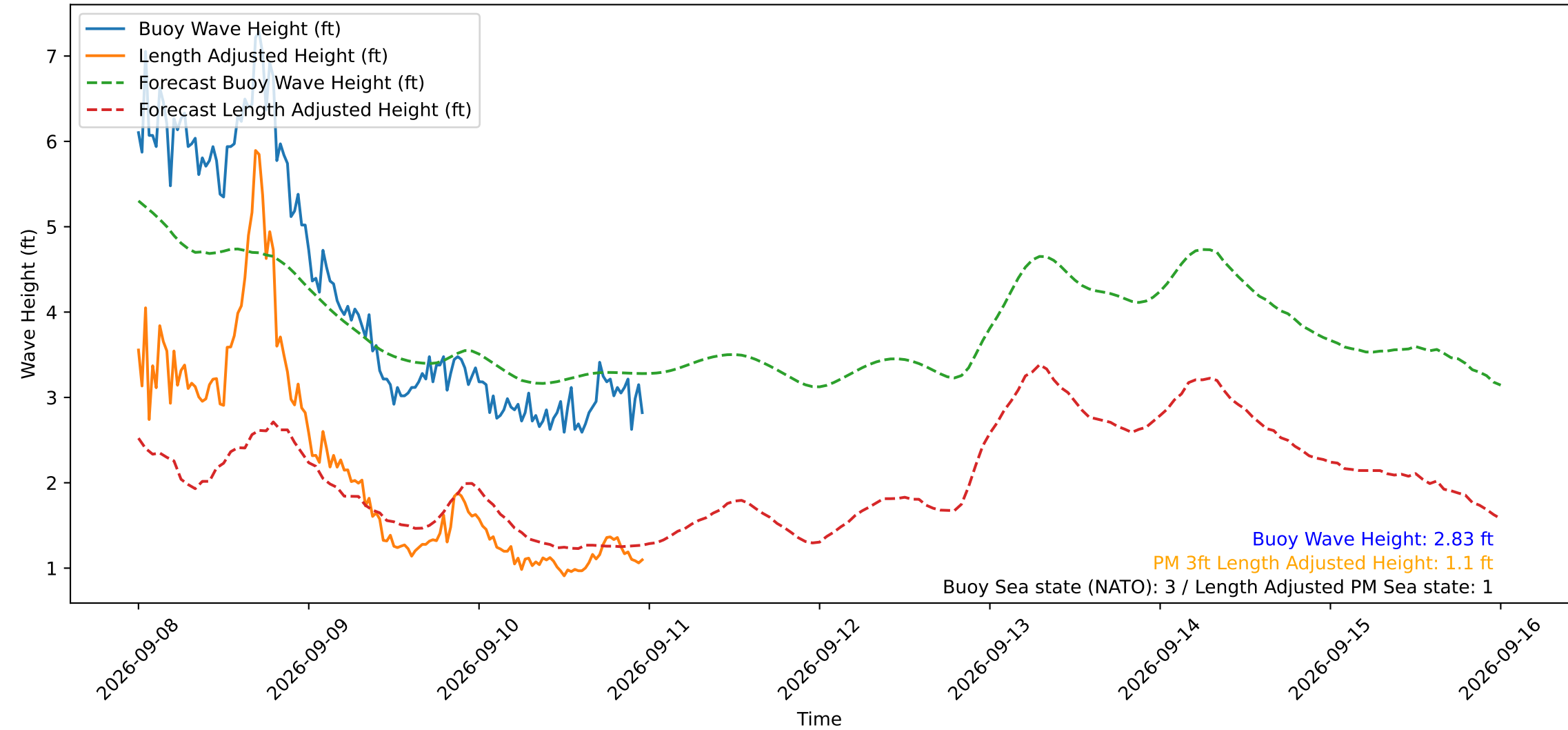
Wave Heights over Time for Green Beach at 2026-09-10 23:51:15
