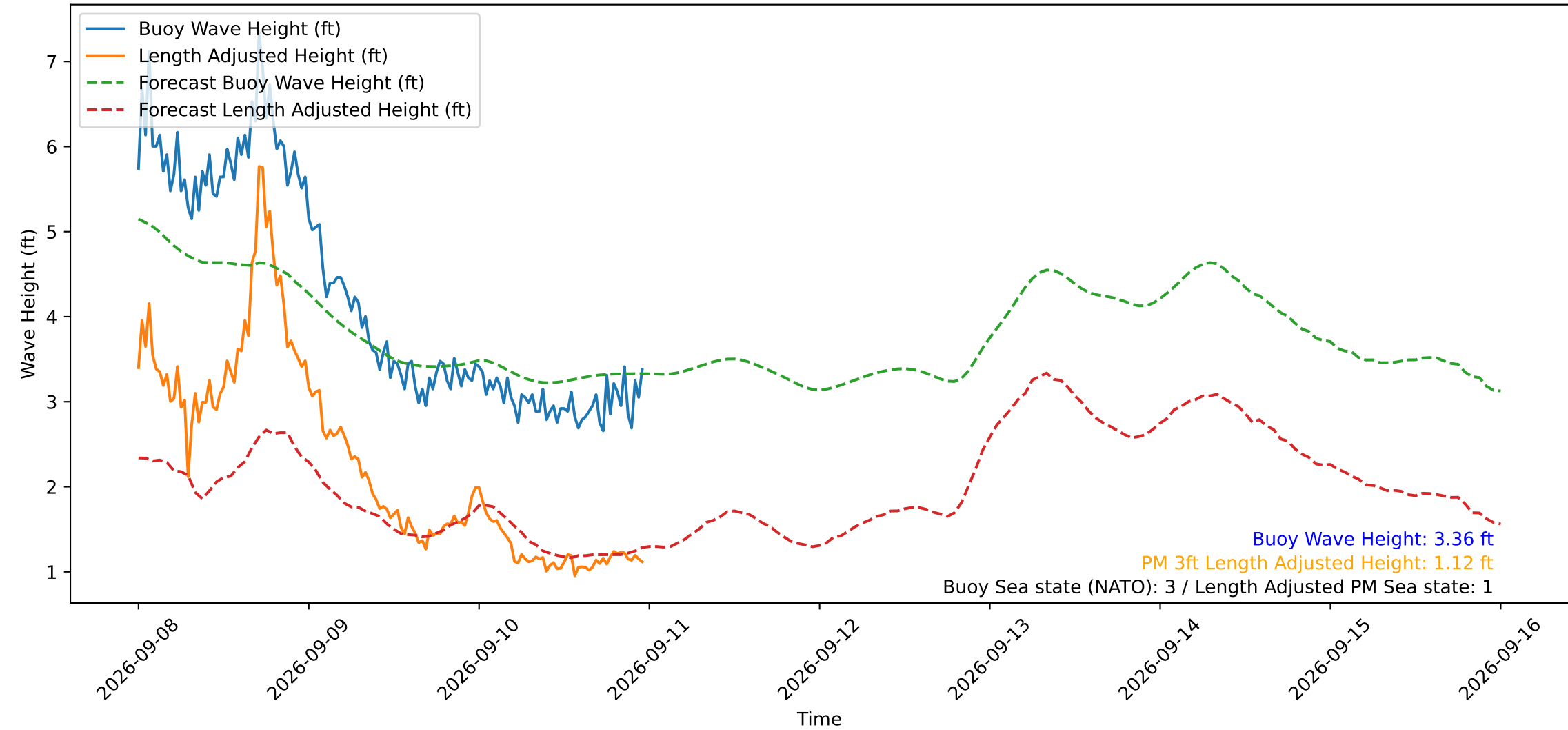
Wave Heights over Time for Oceanside Harbor at 2026-09-10 23:50:29
