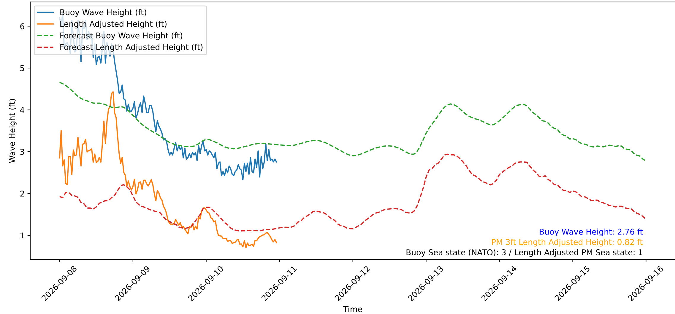
Wave Heights over Time for Red Beach at 2026-09-10 23:50:50
