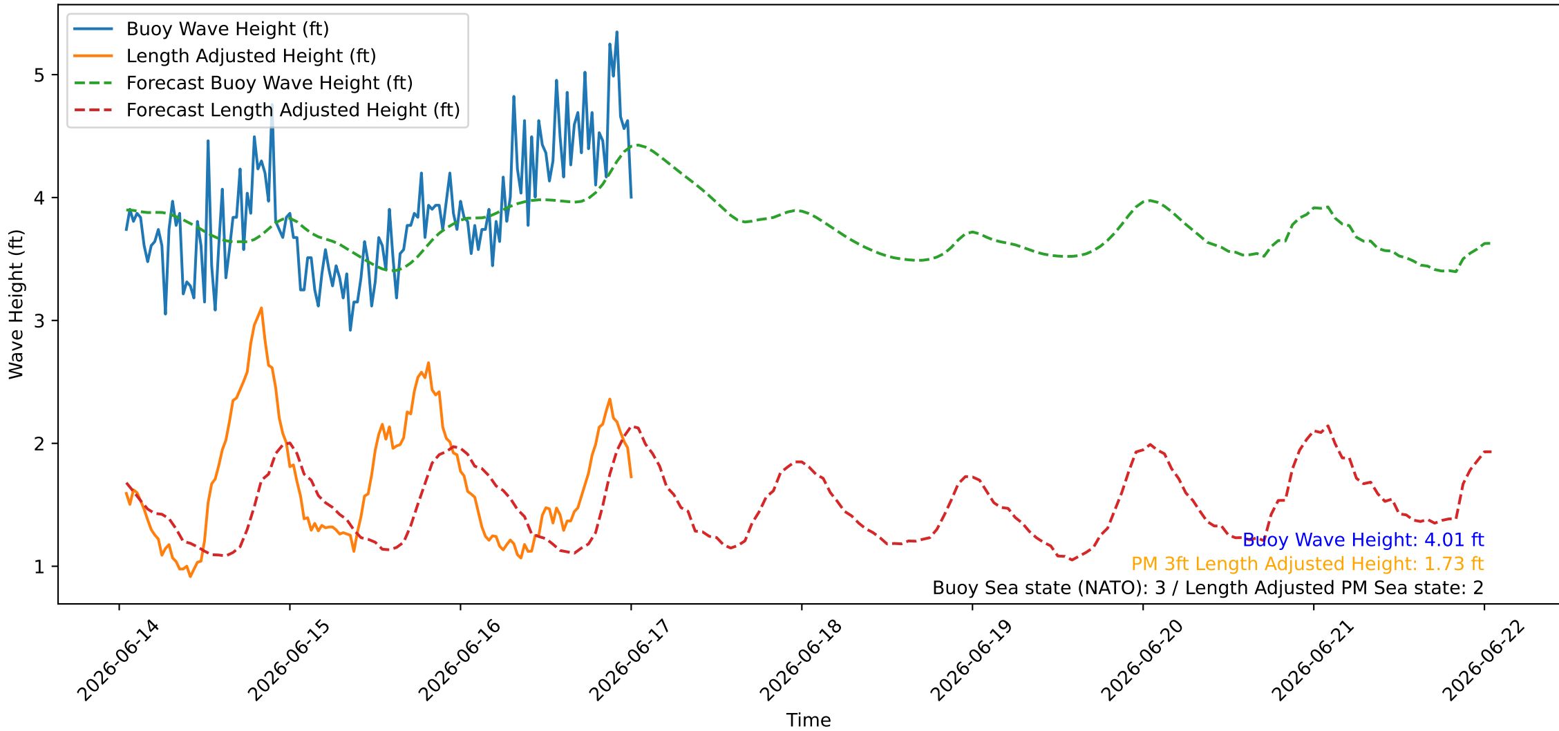
Wave Heights over Time for Red Beach at 2026-06-17 00:50:46
