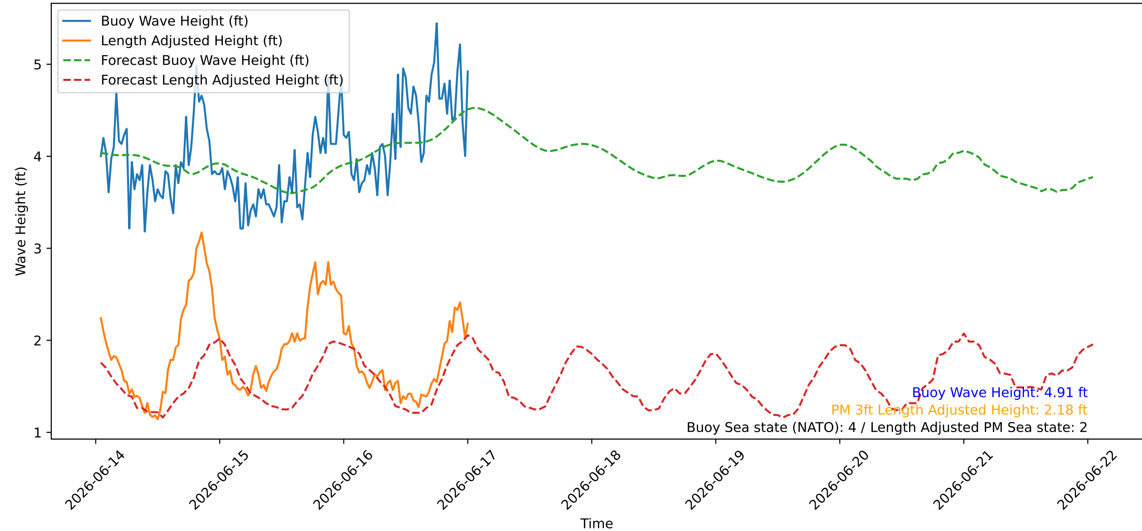
Wave Heights over Time for Oceanside Harbor at 2026-06-17 00:50:26
