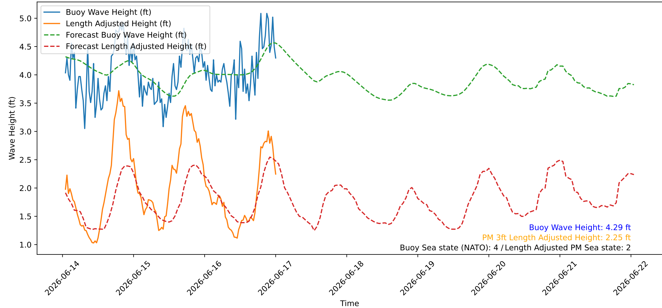
Wave Heights over Time for Green Beach at 2026-06-17 00:51:09
