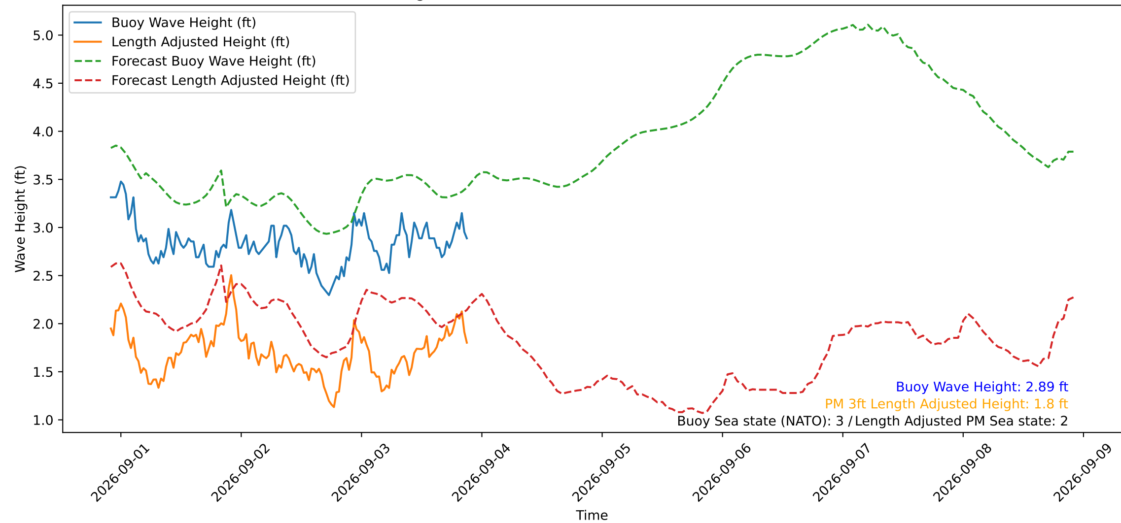
Wave Heights over Time for Red Beach at 2026-09-03 21:40:49
