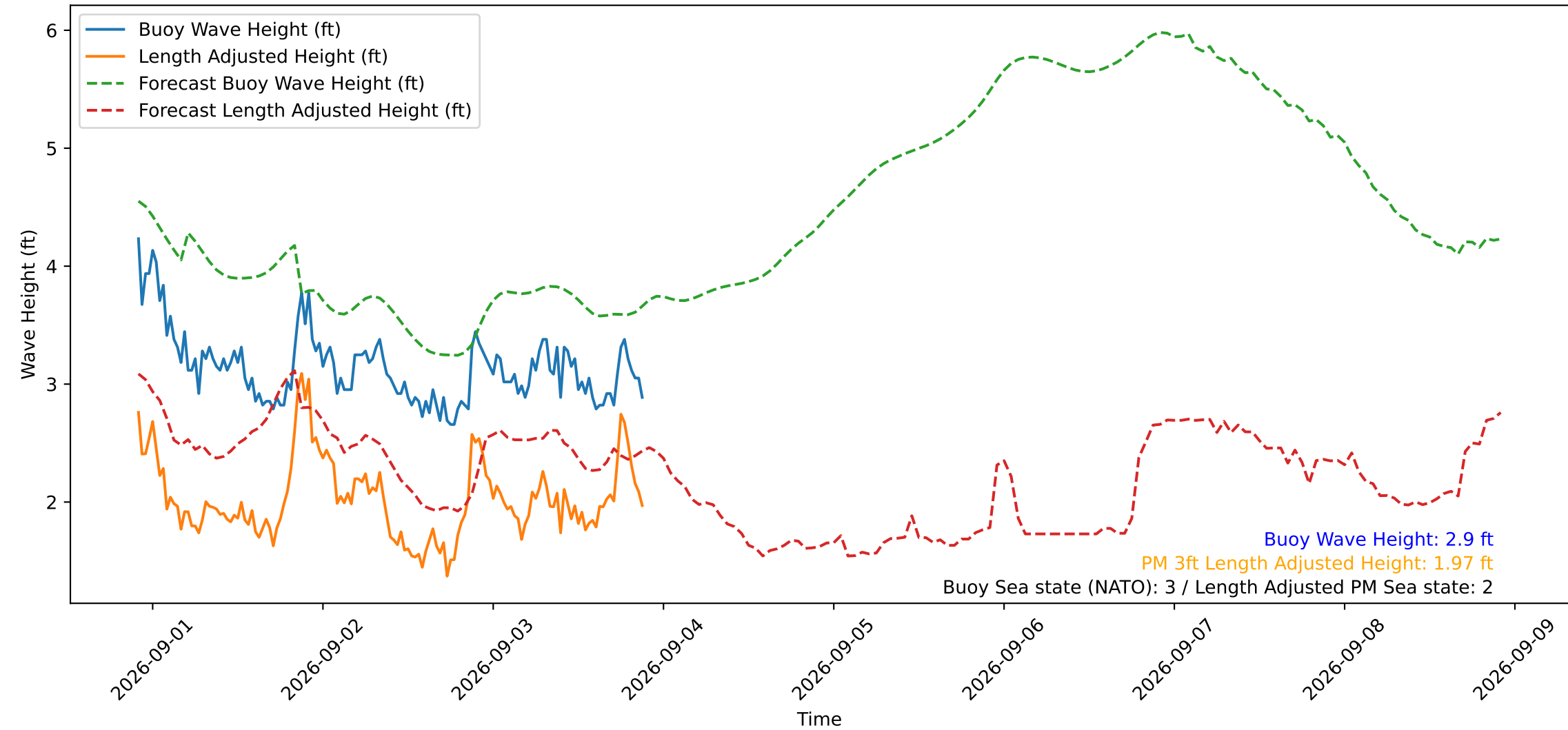
Wave Heights over Time for Green Beach at 2026-09-03 21:41:13
