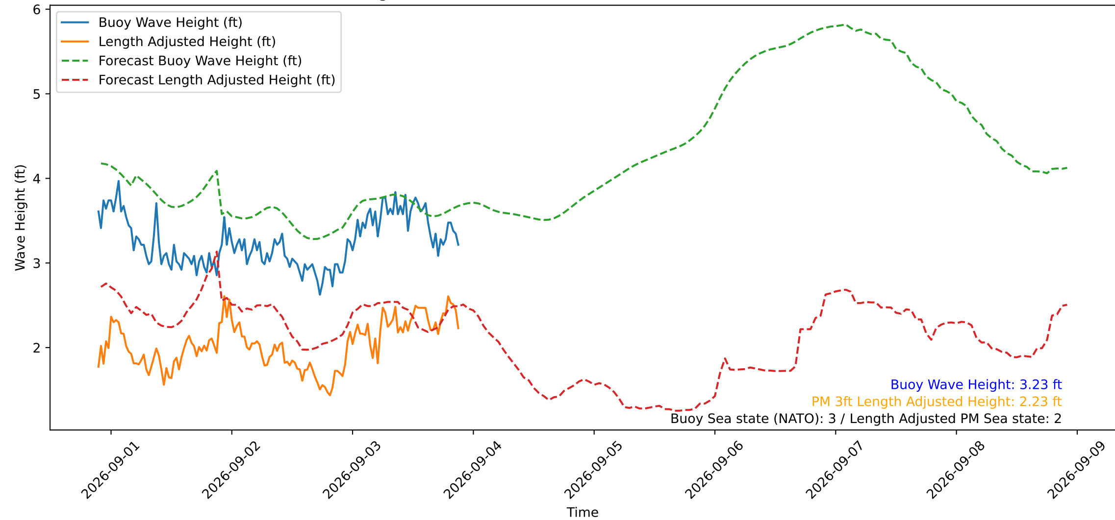
Wave Heights over Time for Oceanside Harbor at 2026-09-03 21:40:29
