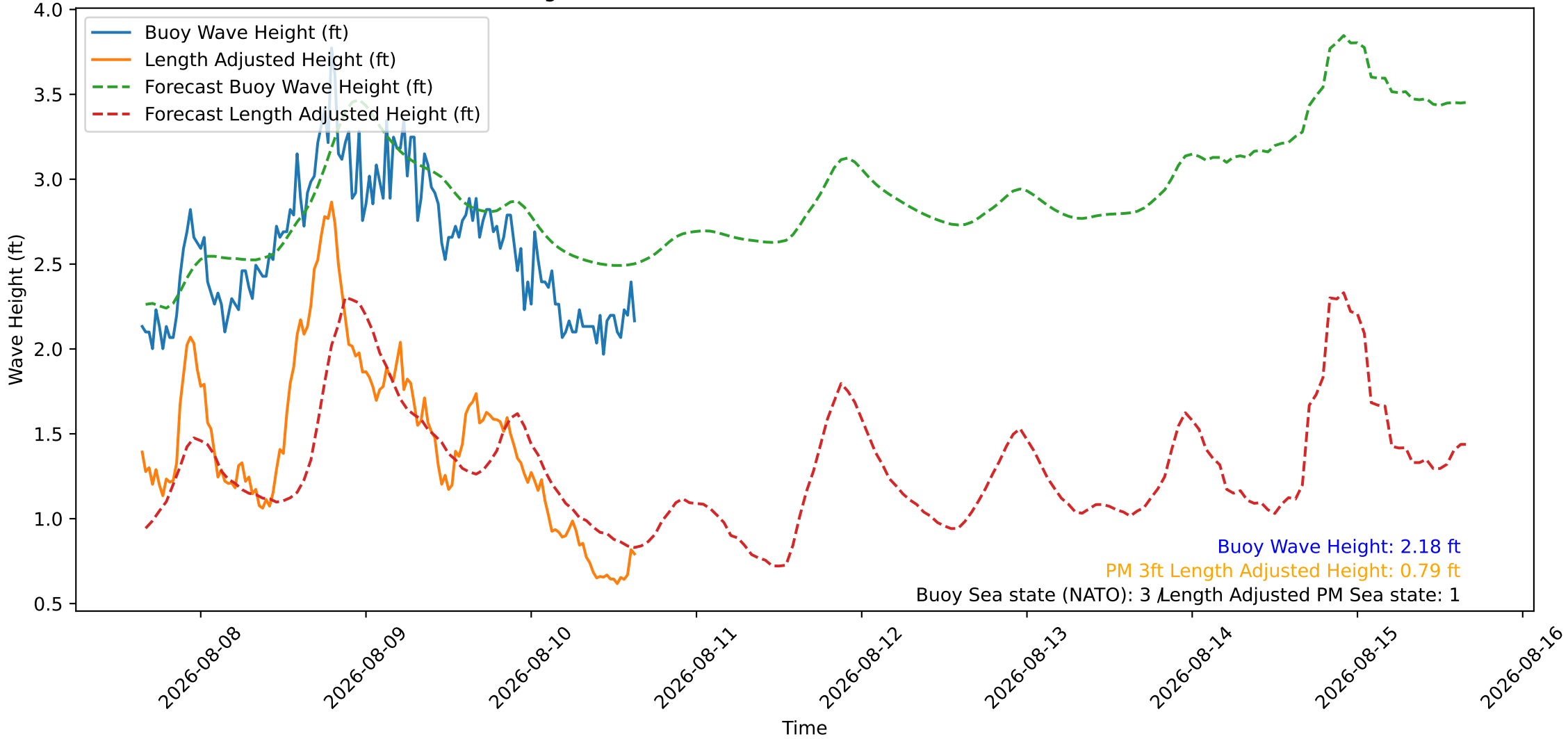
Wave Heights over Time for Green Beach at 2026-08-10 15:41:08
