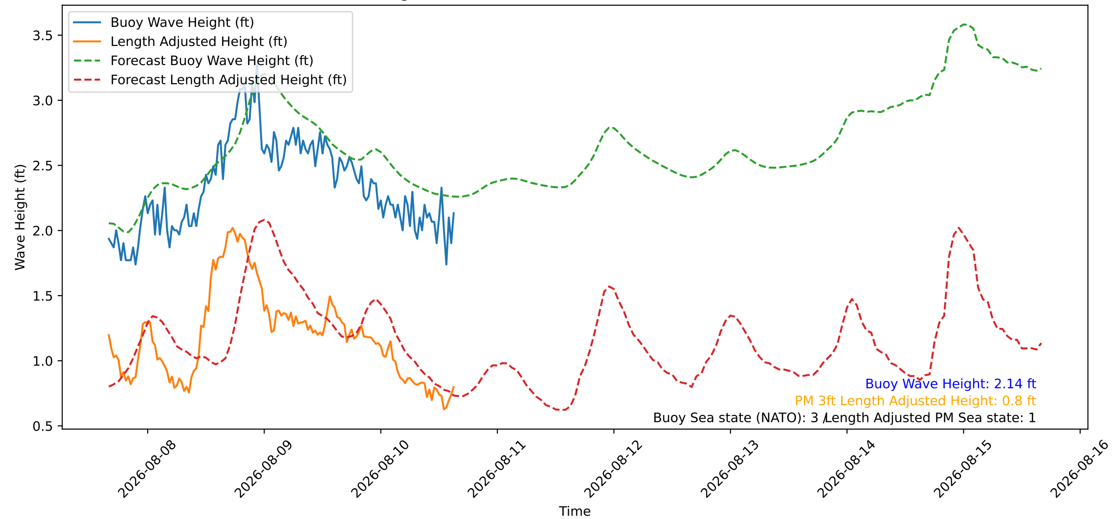
Wave Heights over Time for Red Beach at 2026-08-10 15:40:46
