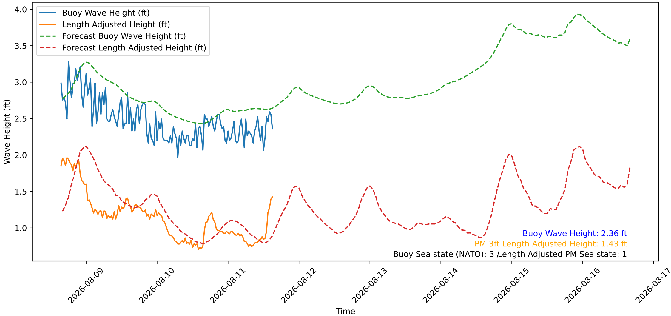
Wave Heights over Time for Oceanside Harbor at 2026-08-11 15:40:26
