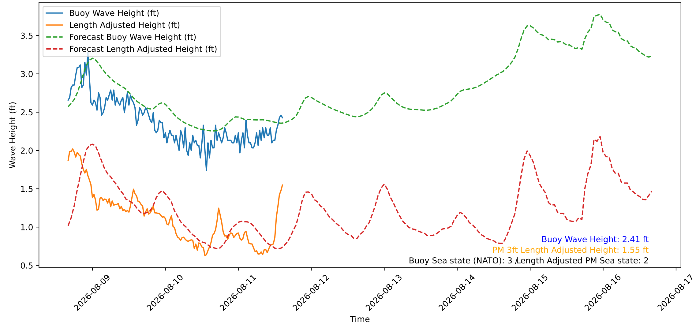
Wave Heights over Time for Red Beach at 2026-08-11 15:40:45
