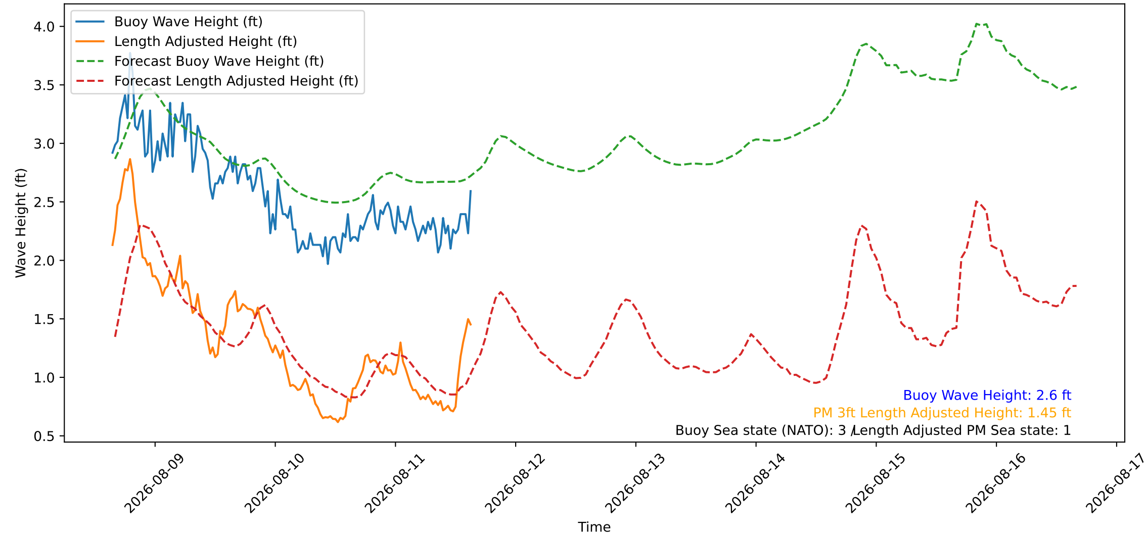
Wave Heights over Time for Green Beach at 2026-08-11 15:41:08
