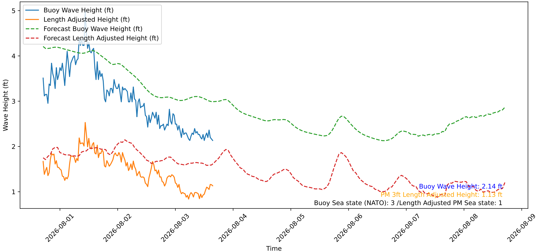
Wave Heights over Time for Green Beach at 2026-08-03 17:01:08
