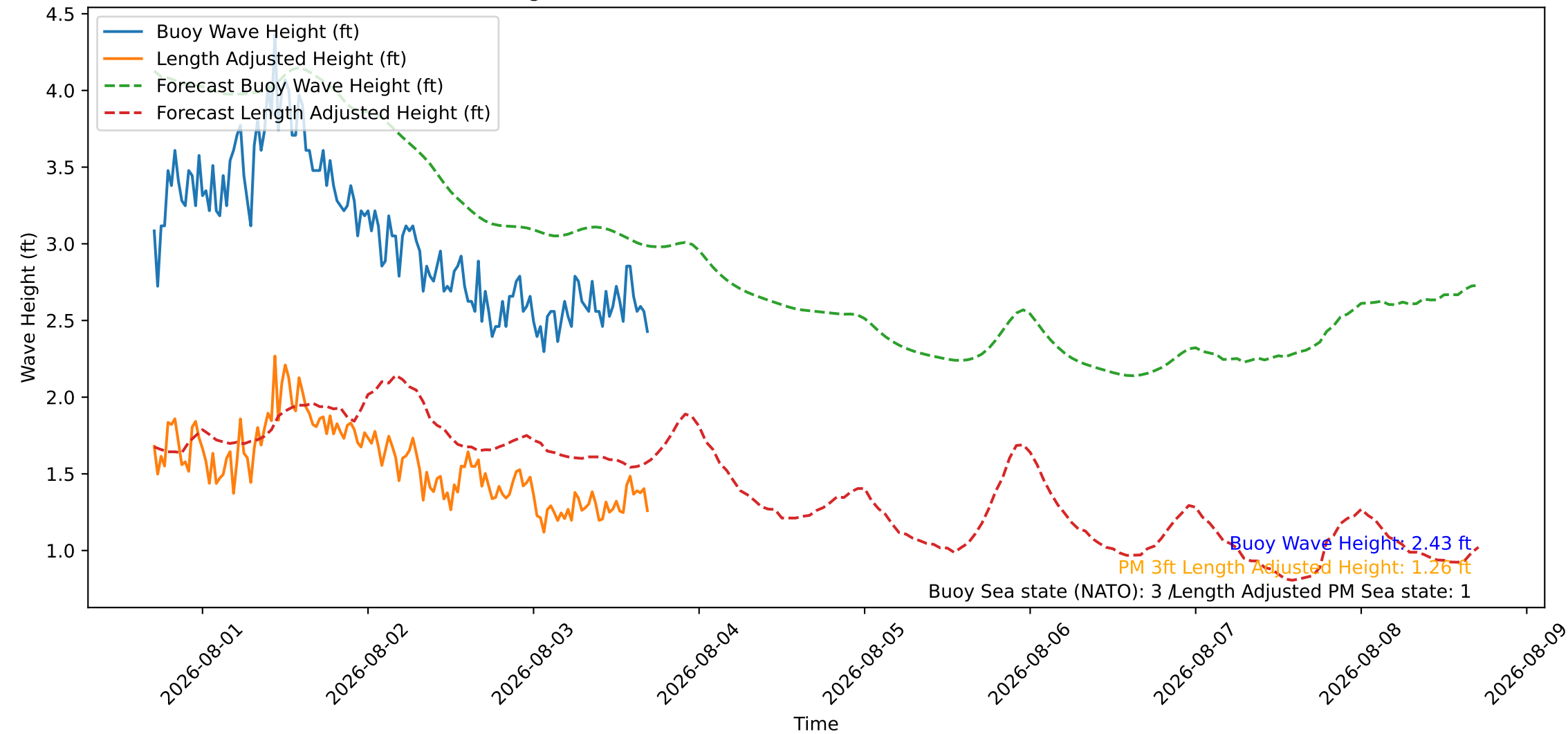
Wave Heights over Time for Oceanside Harbor at 2026-08-03 17:00:27
