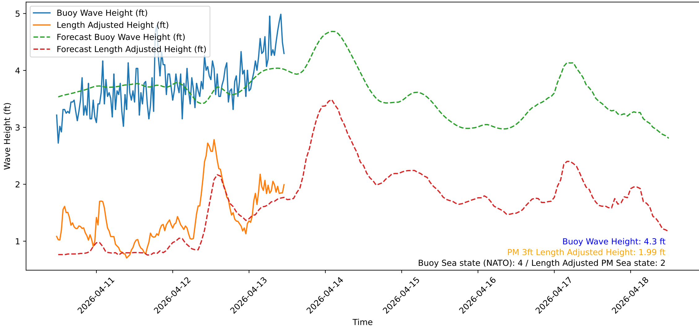
Wave Heights over Time for Oceanside Harbor at 2026-04-13 11:40:31
