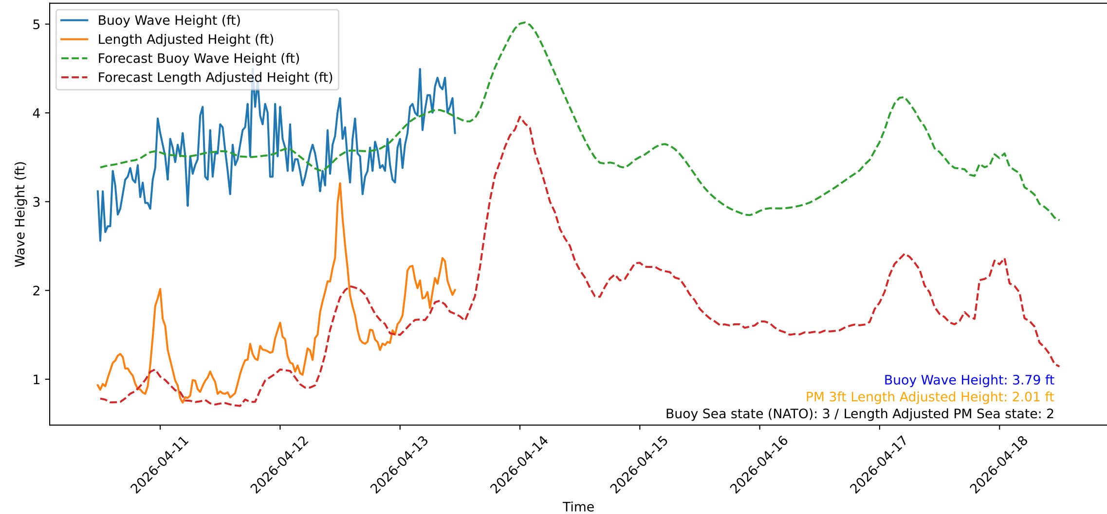
Wave Heights over Time for Green Beach at 2026-04-13 11:41:13
