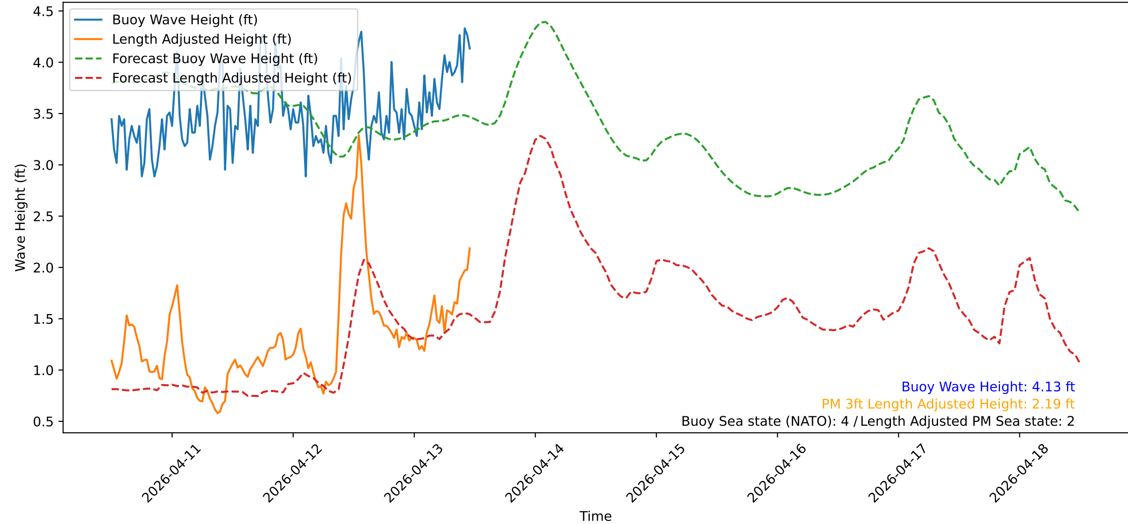
Wave Heights over Time for Red Beach at 2026-04-13 11:40:50
