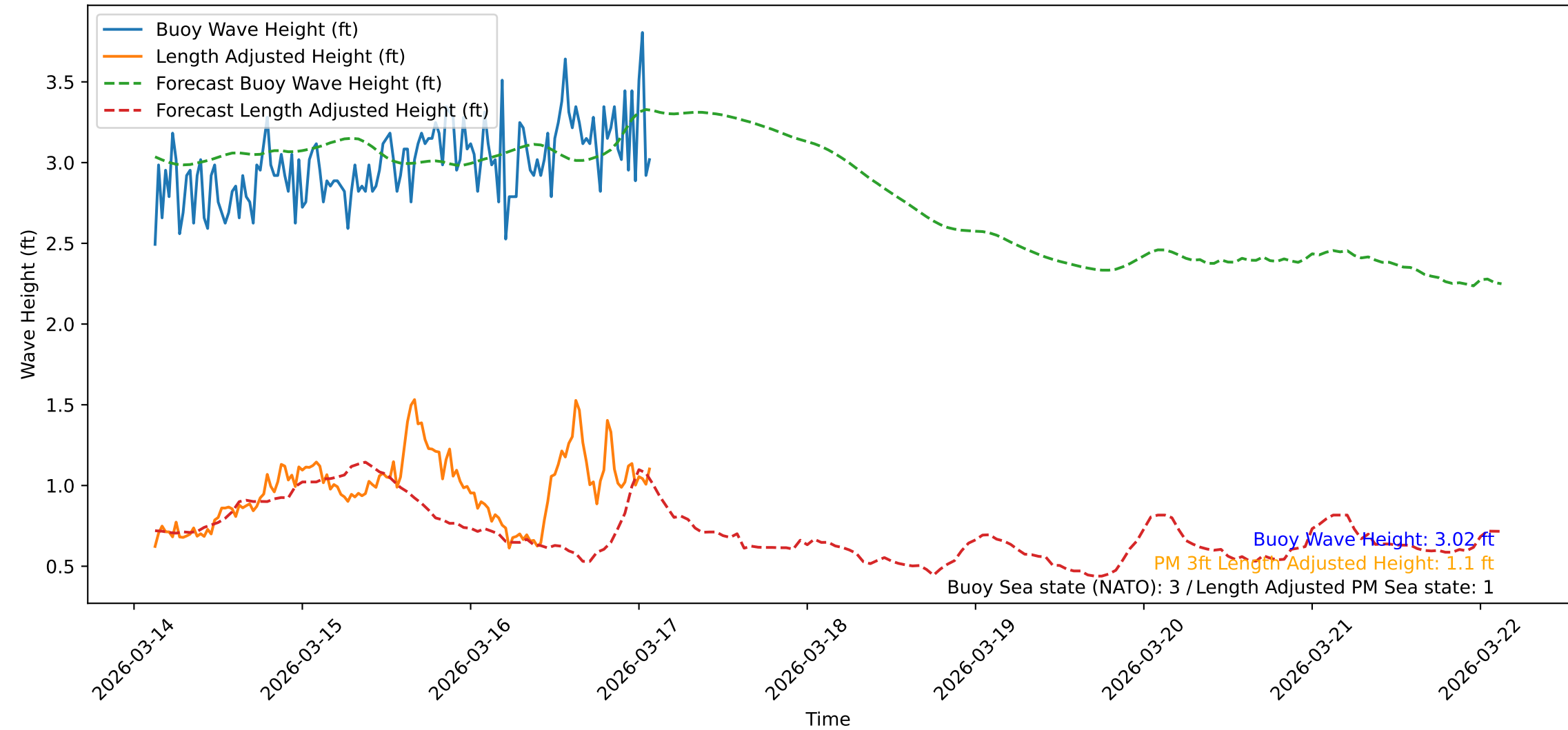
Wave Heights over Time for Red Beach at 2026-03-17 02:31:07
