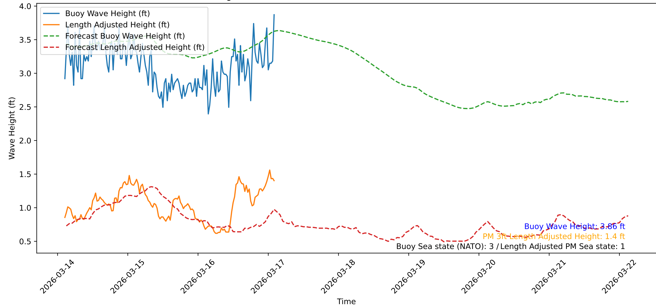
Wave Heights over Time for Oceanside Harbor at 2026-03-17 02:30:45
