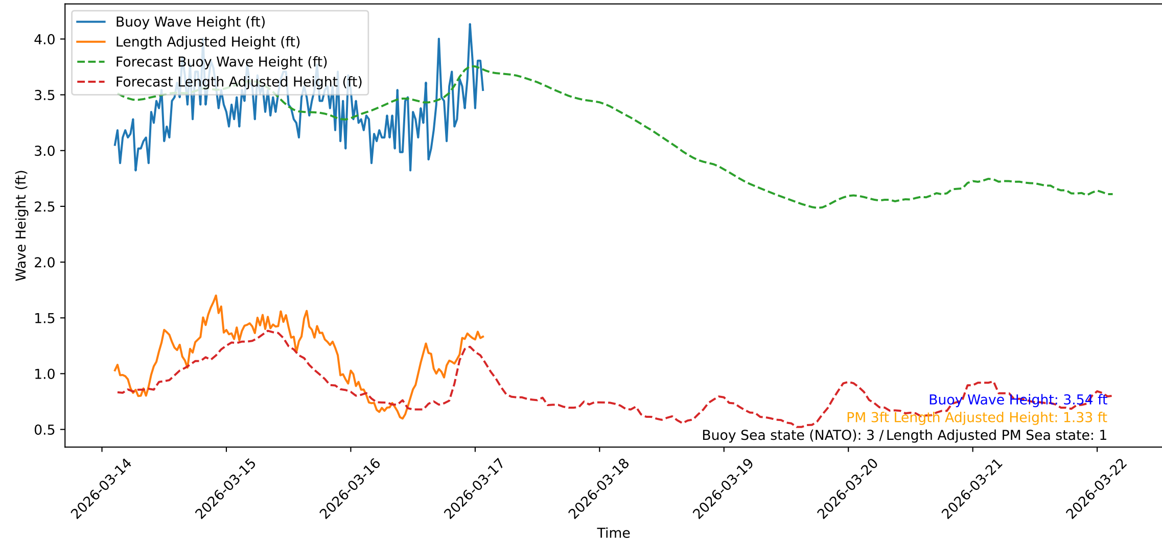
Wave Heights over Time for Green Beach at 2026-03-17 02:31:44
