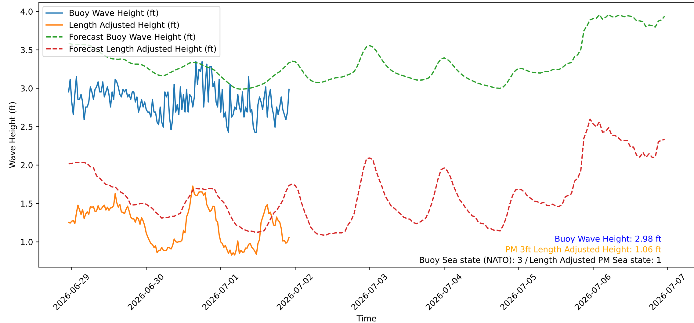
Wave Heights over Time for Red Beach at 2026-07-01 22:40:46
