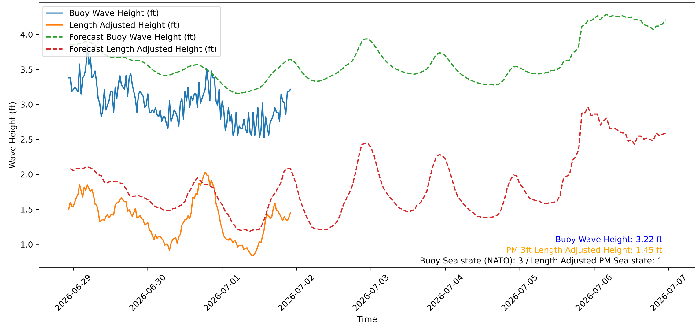
Wave Heights over Time for Green Beach at 2026-07-01 22:41:09
