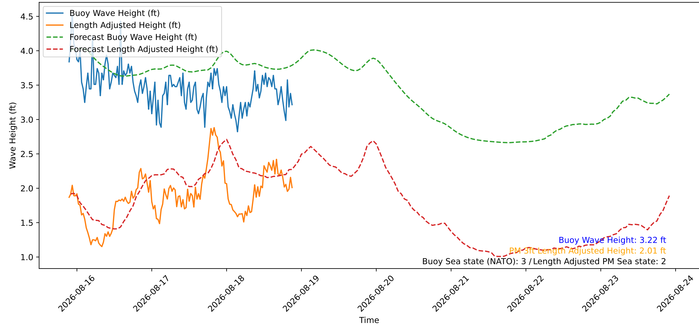
Wave Heights over Time for Oceanside Harbor at 2026-08-18 21:40:27
