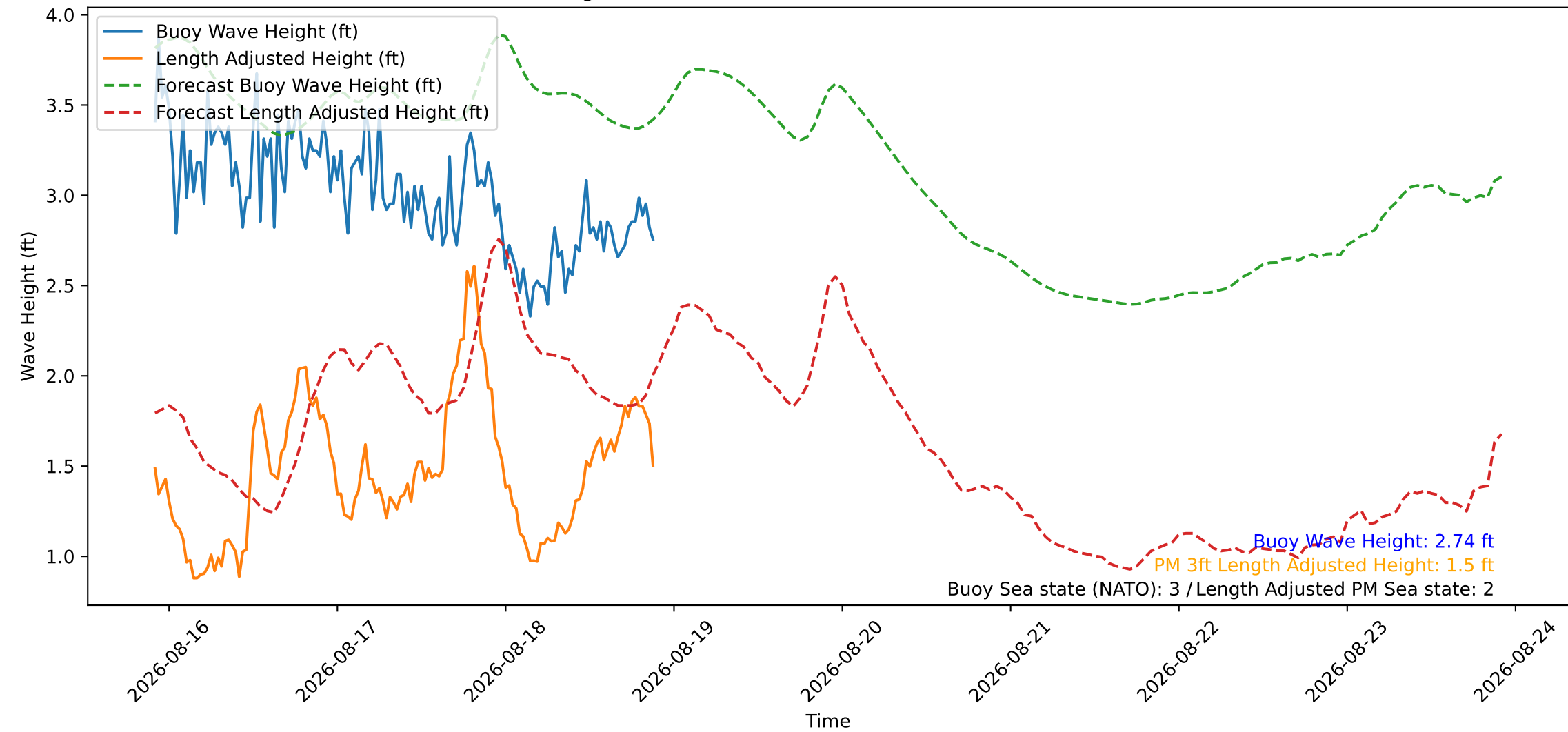
Wave Heights over Time for Red Beach at 2026-08-18 21:40:46
