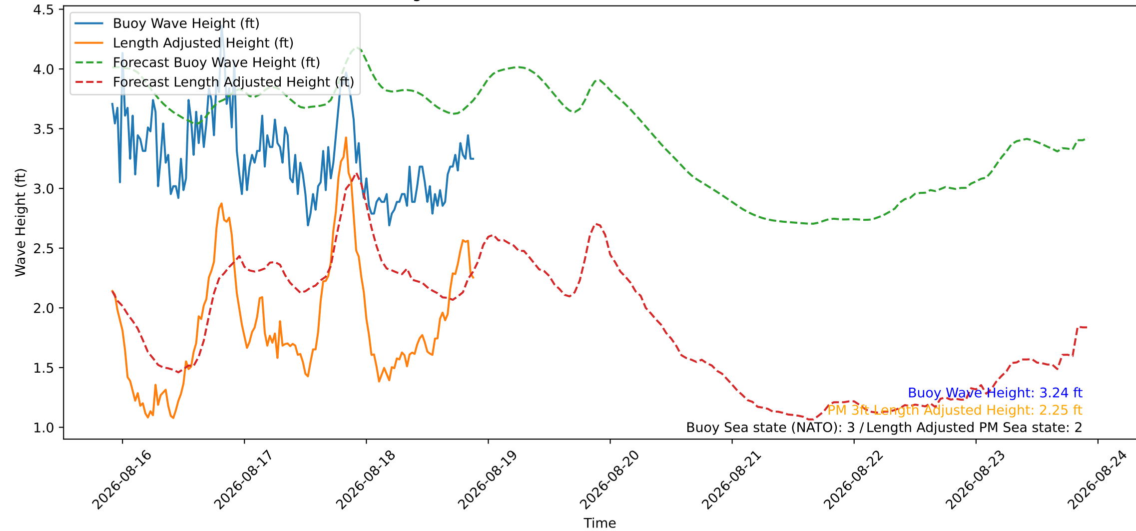
Wave Heights over Time for Green Beach at 2026-08-18 21:41:09
