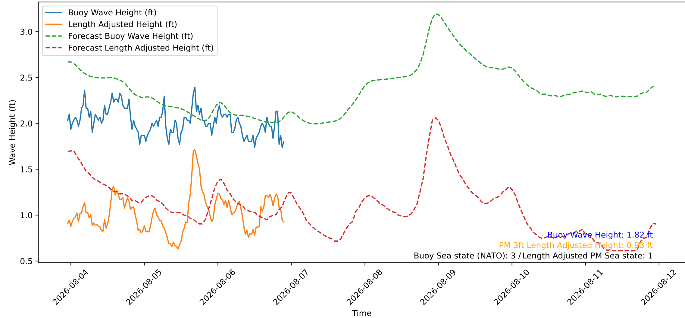
Wave Heights over Time for Red Beach at 2026-08-06 22:30:46
