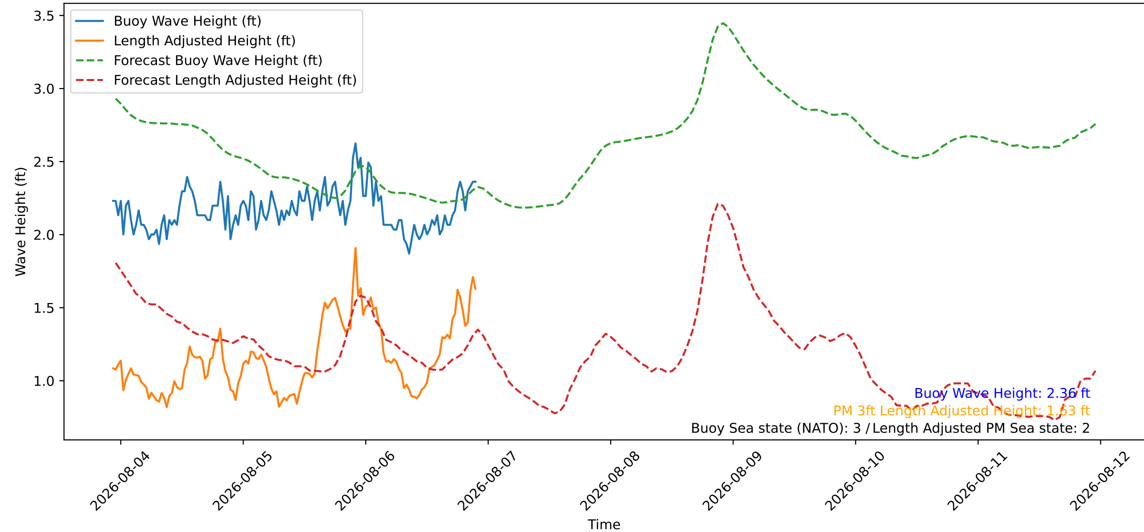
Wave Heights over Time for Green Beach at 2026-08-06 22:31:08
