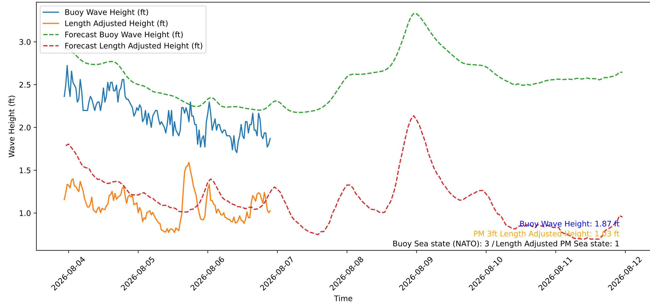
Wave Heights over Time for Oceanside Harbor at 2026-08-06 22:30:27
