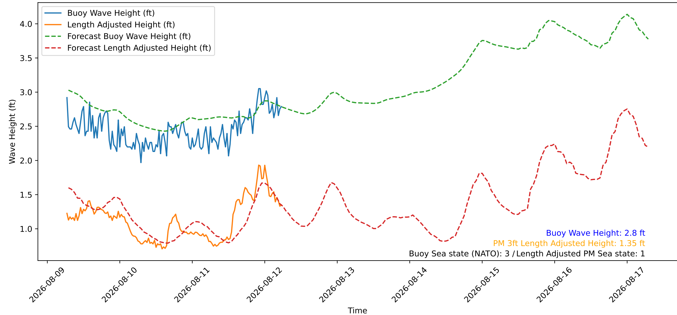
Wave Heights over Time for Oceanside Harbor at 2026-08-12 06:30:27
