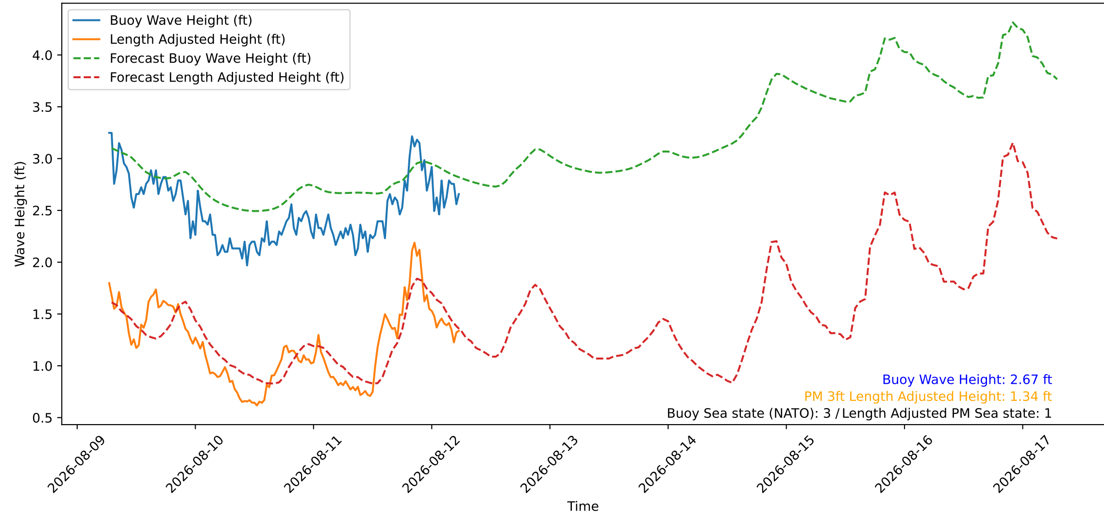
Wave Heights over Time for Green Beach at 2026-08-12 06:31:09
