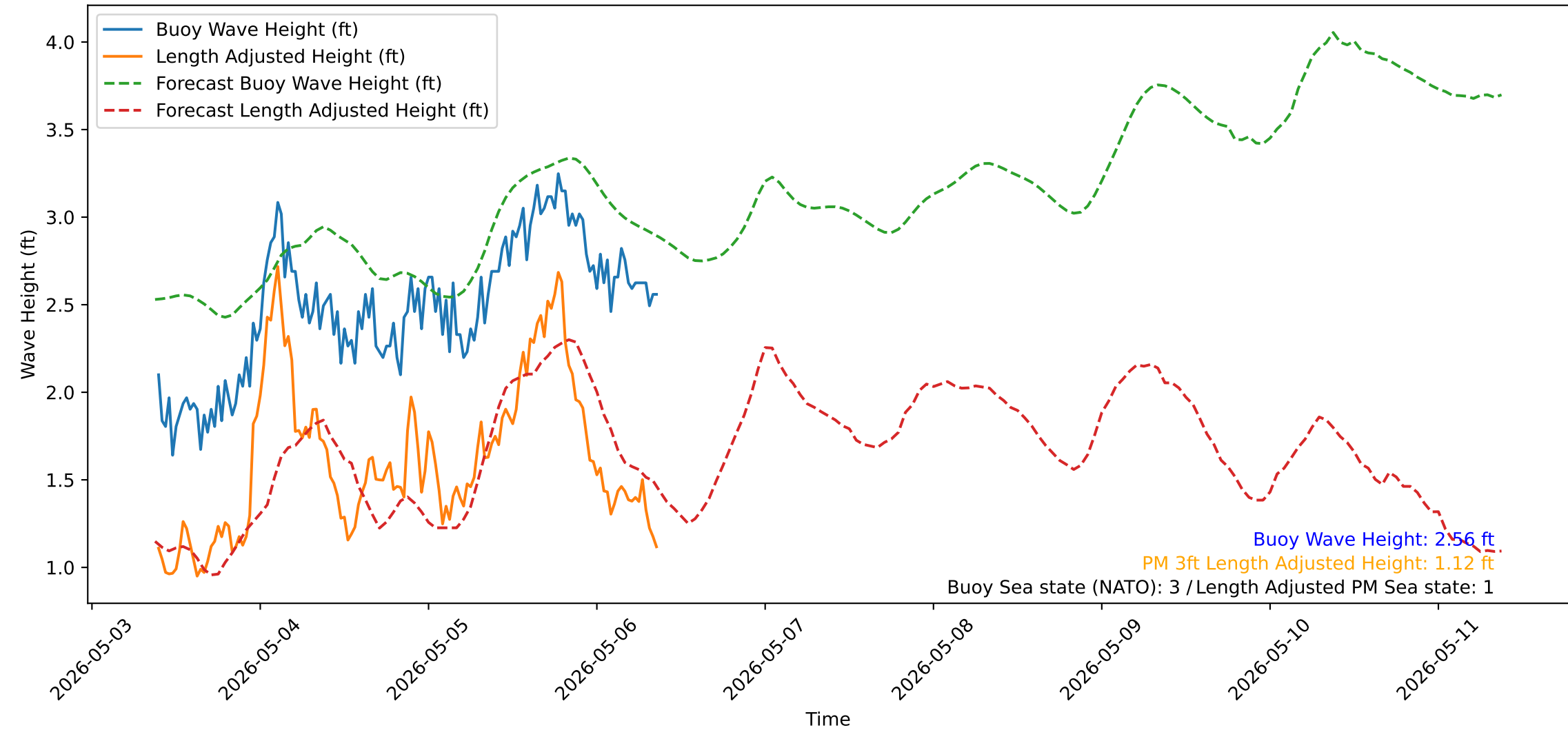
Wave Heights over Time for Oceanside Harbor at 2026-05-06 09:20:30
