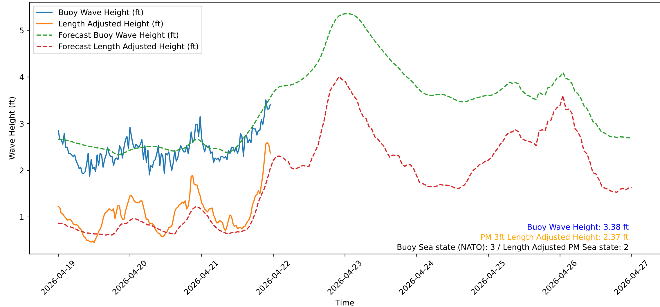
Wave Heights over Time for Green Beach at 2026-04-22 00:01:12
