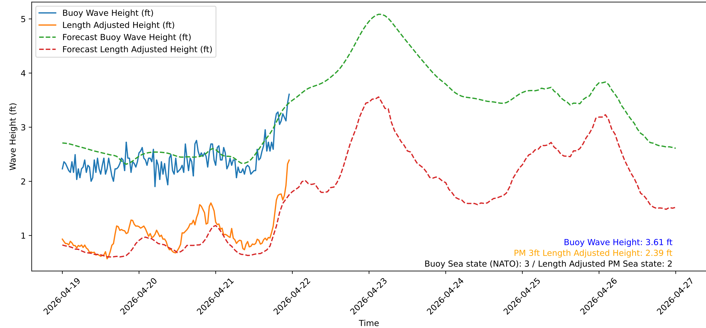
Wave Heights over Time for Oceanside Harbor at 2026-04-22 00:00:31
