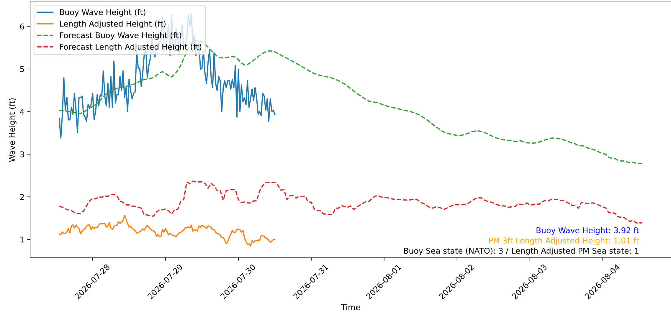
Wave Heights over Time for Green Beach at 2026-07-30 13:01:09
