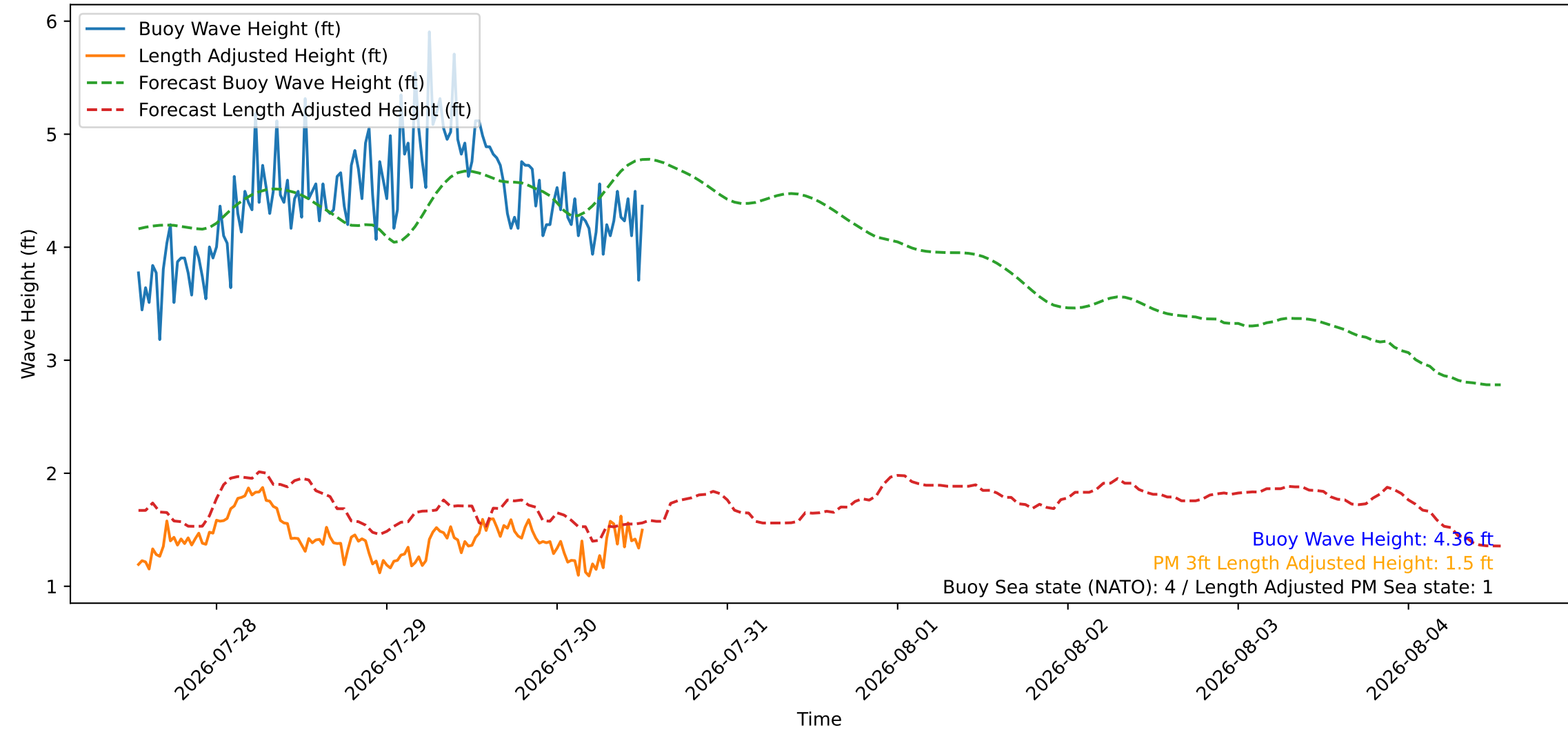
Wave Heights over Time for Oceanside Harbor at 2026-07-30 13:00:27
