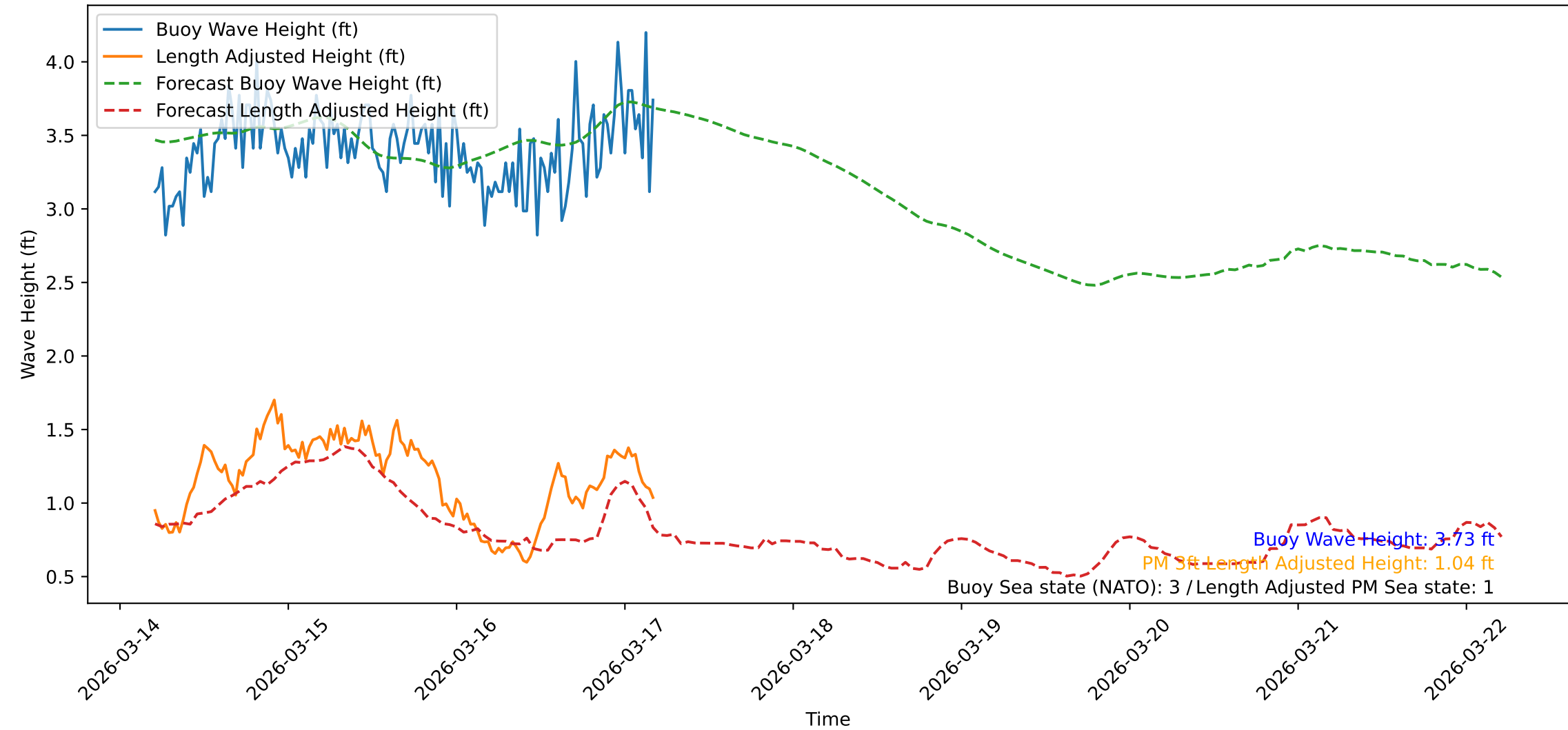
Wave Heights over Time for Green Beach at 2026-03-17 04:51:48
