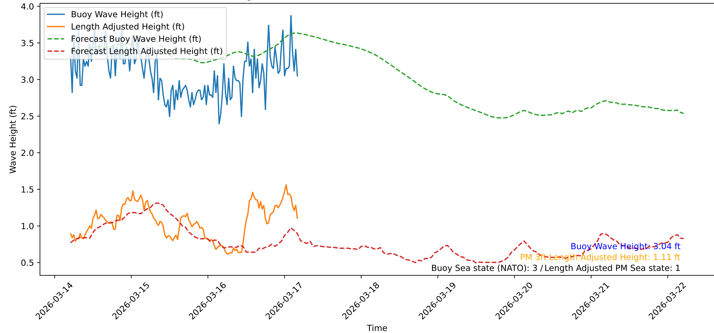
Wave Heights over Time for Oceanside Harbor at 2026-03-17 04:50:45
