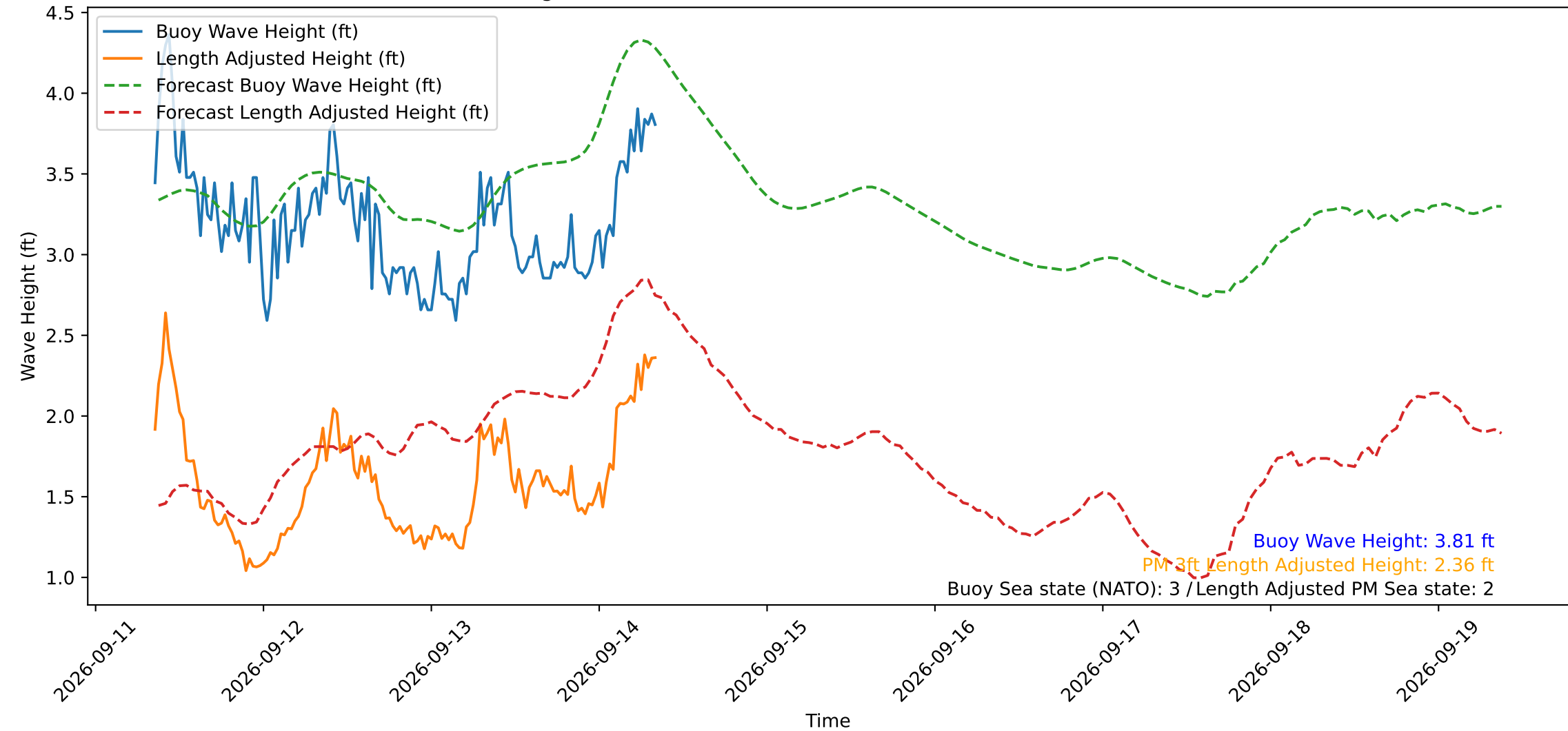
Wave Heights over Time for Oceanside Harbor at 2026-09-14 08:30:30
