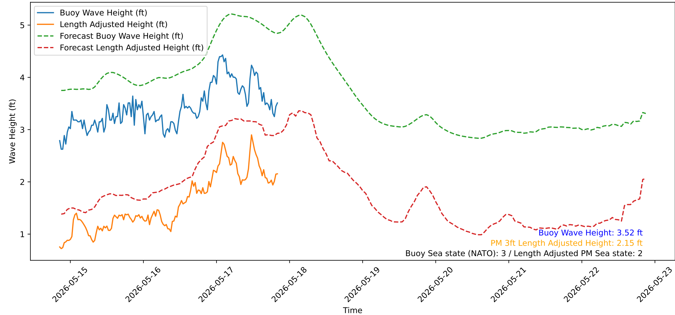
Wave Heights over Time for Green Beach at 2026-05-17 20:41:14
