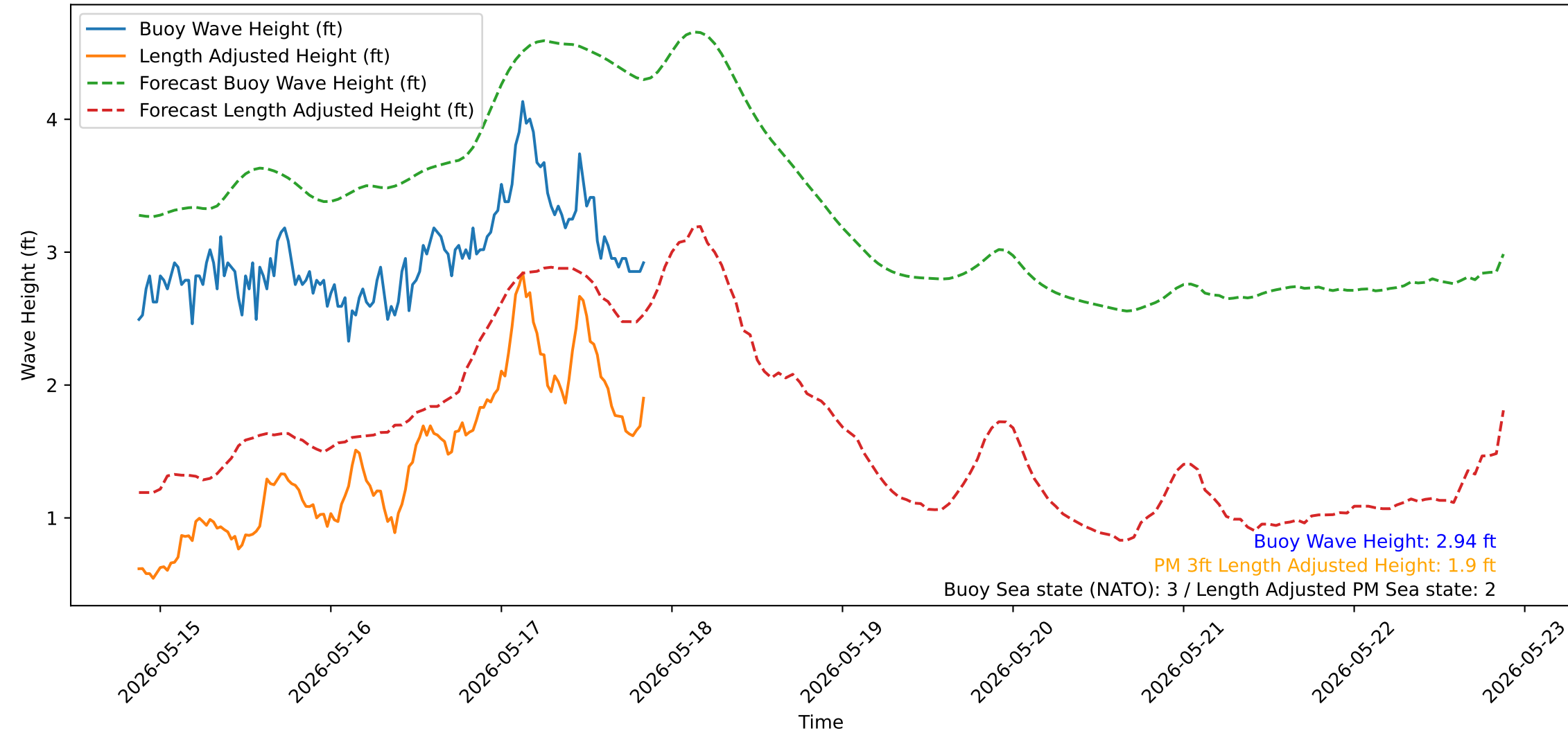
Wave Heights over Time for Red Beach at 2026-05-17 20:40:51
