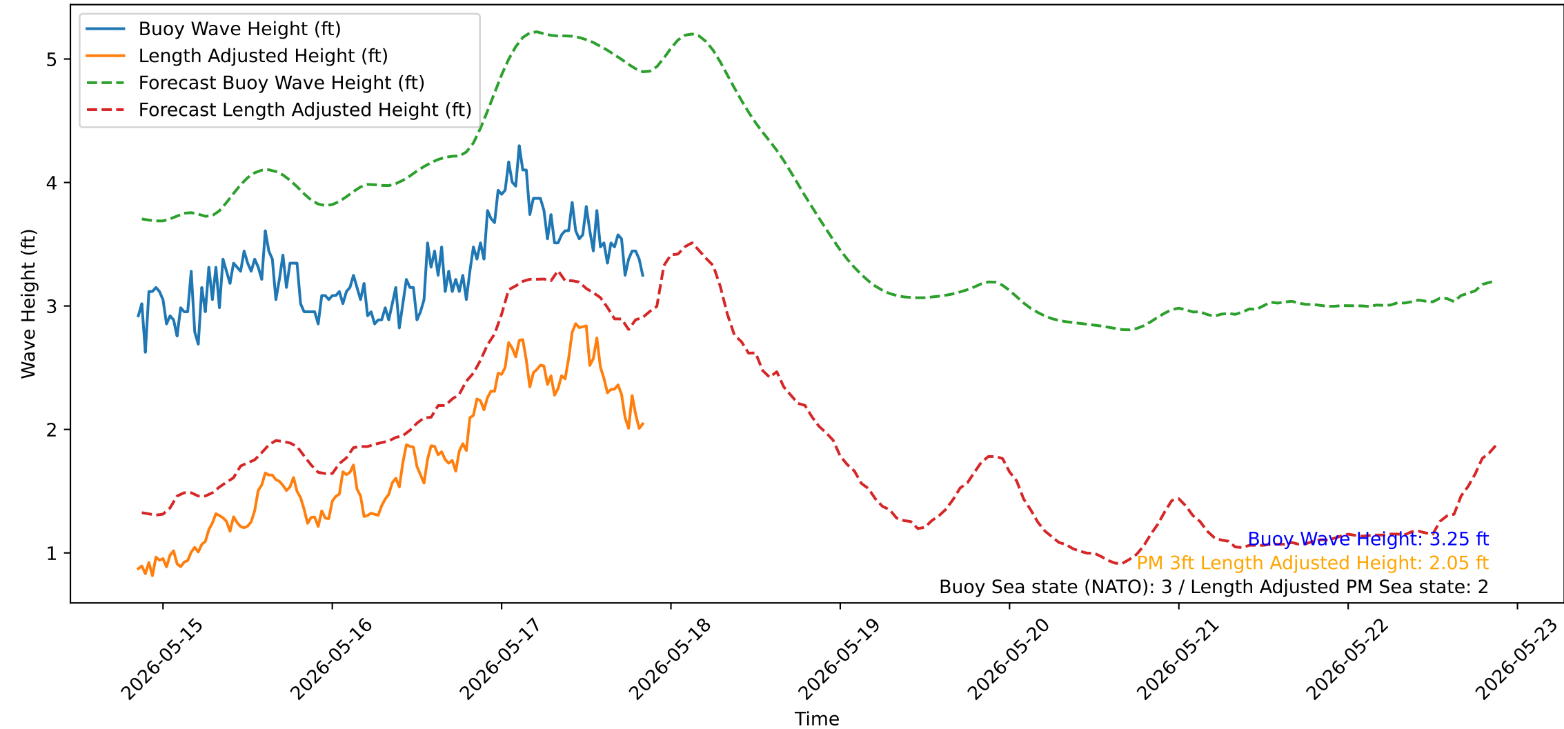
Wave Heights over Time for Oceanside Harbor at 2026-05-17 20:40:32
