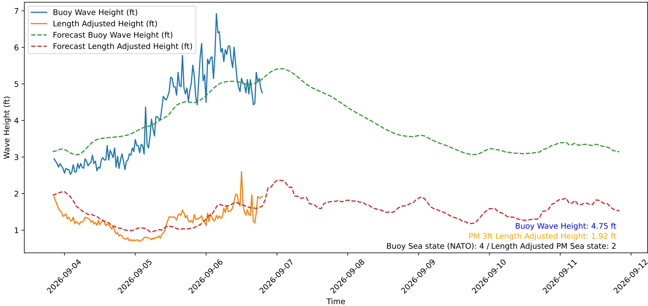
Wave Heights over Time for Red Beach at 2026-09-06 20:00:48
