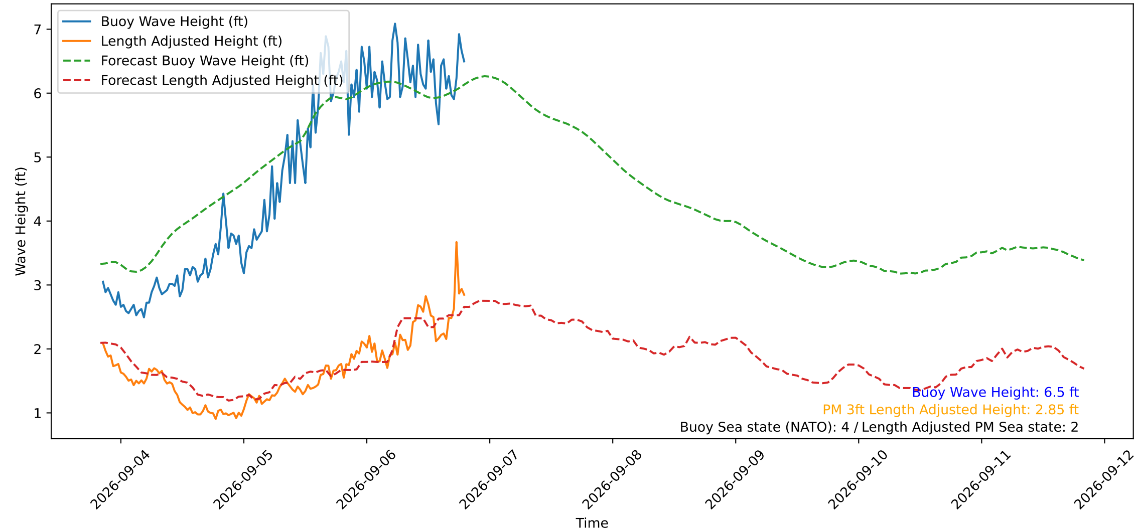
Wave Heights over Time for Green Beach at 2026-09-06 20:01:11
