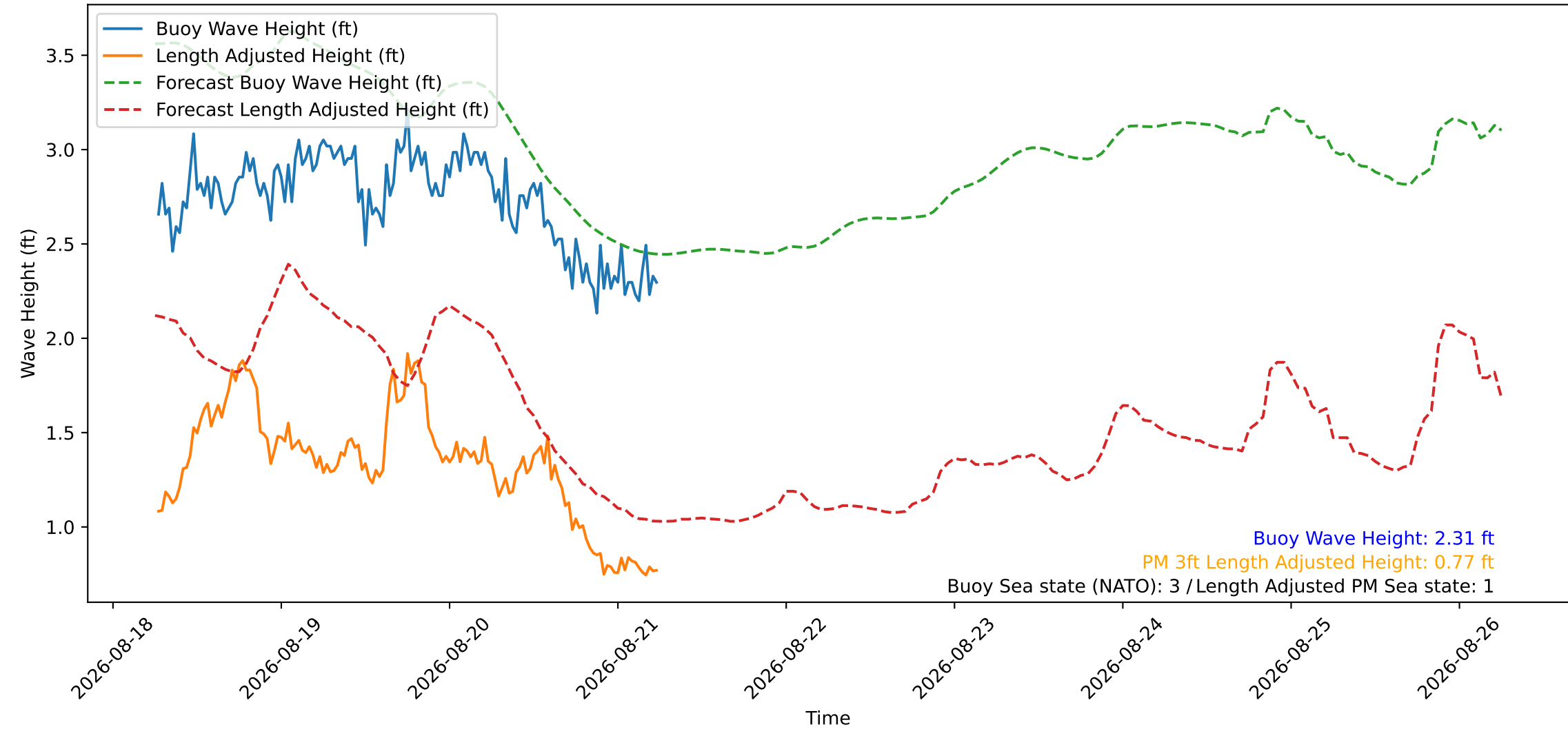
Wave Heights over Time for Red Beach at 2026-08-21 06:10:46
