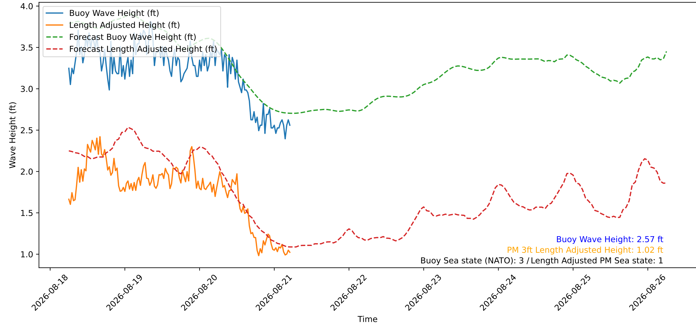
Wave Heights over Time for Oceanside Harbor at 2026-08-21 06:10:26
