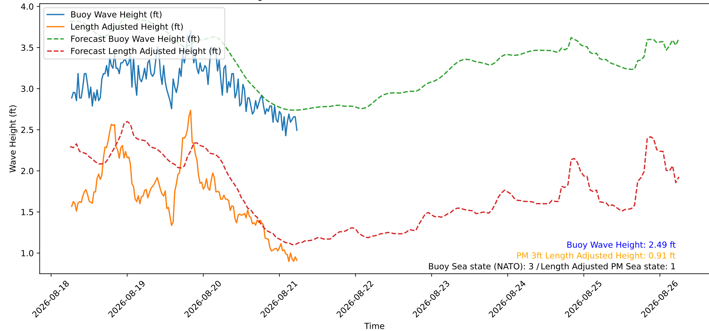
Wave Heights over Time for Green Beach at 2026-08-21 06:11:08
