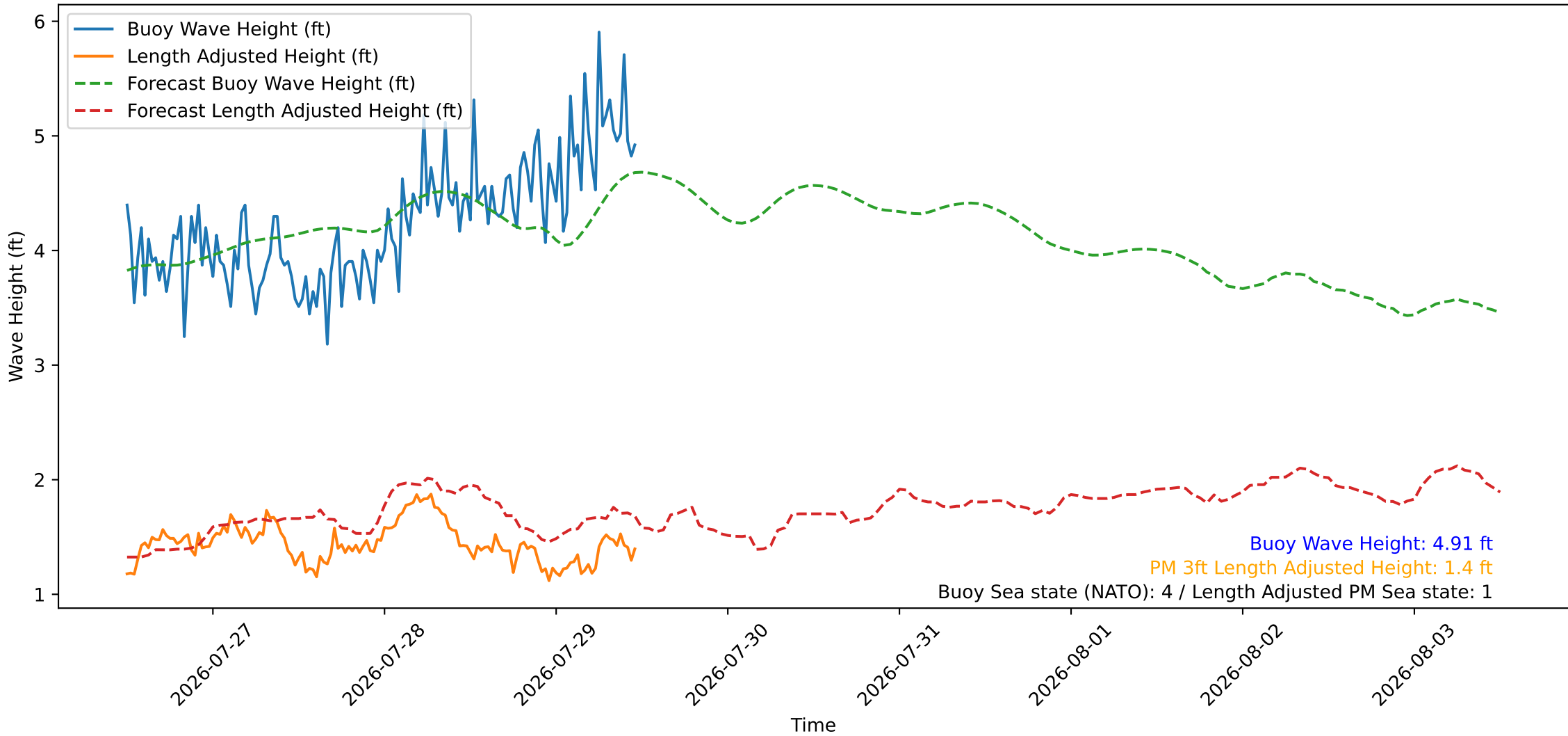
Wave Heights over Time for Oceanside Harbor at 2026-07-29 12:00:26
