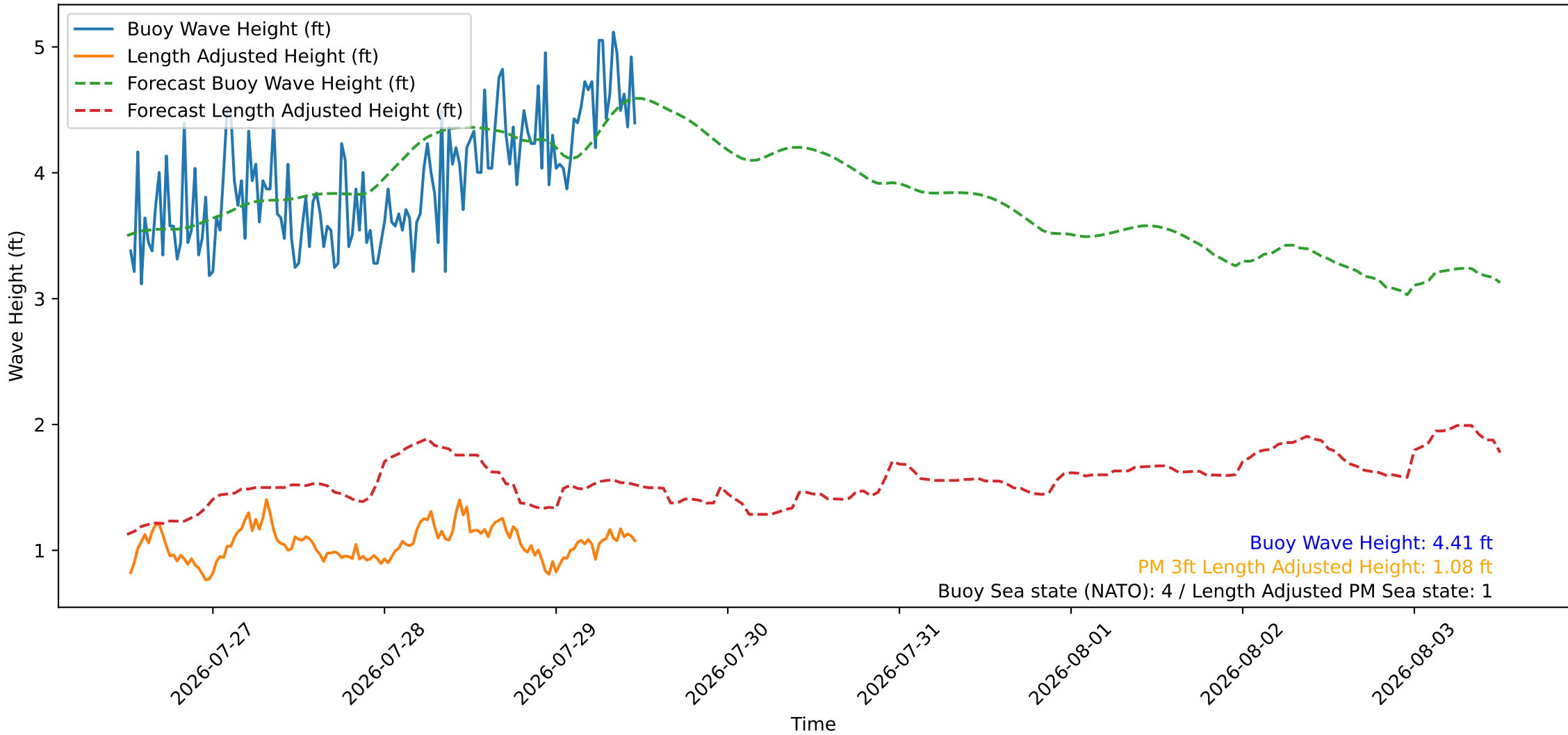
Wave Heights over Time for Red Beach at 2026-07-29 12:00:46
