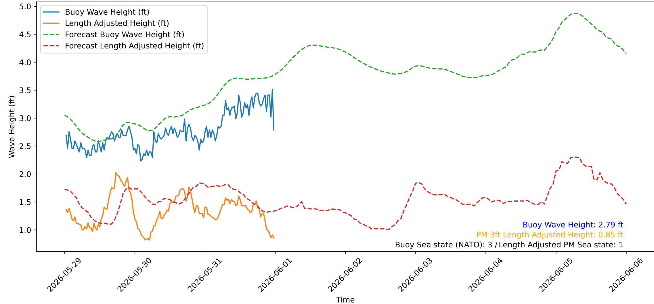
Wave Heights over Time for Red Beach at 2026-06-01 00:10:45
