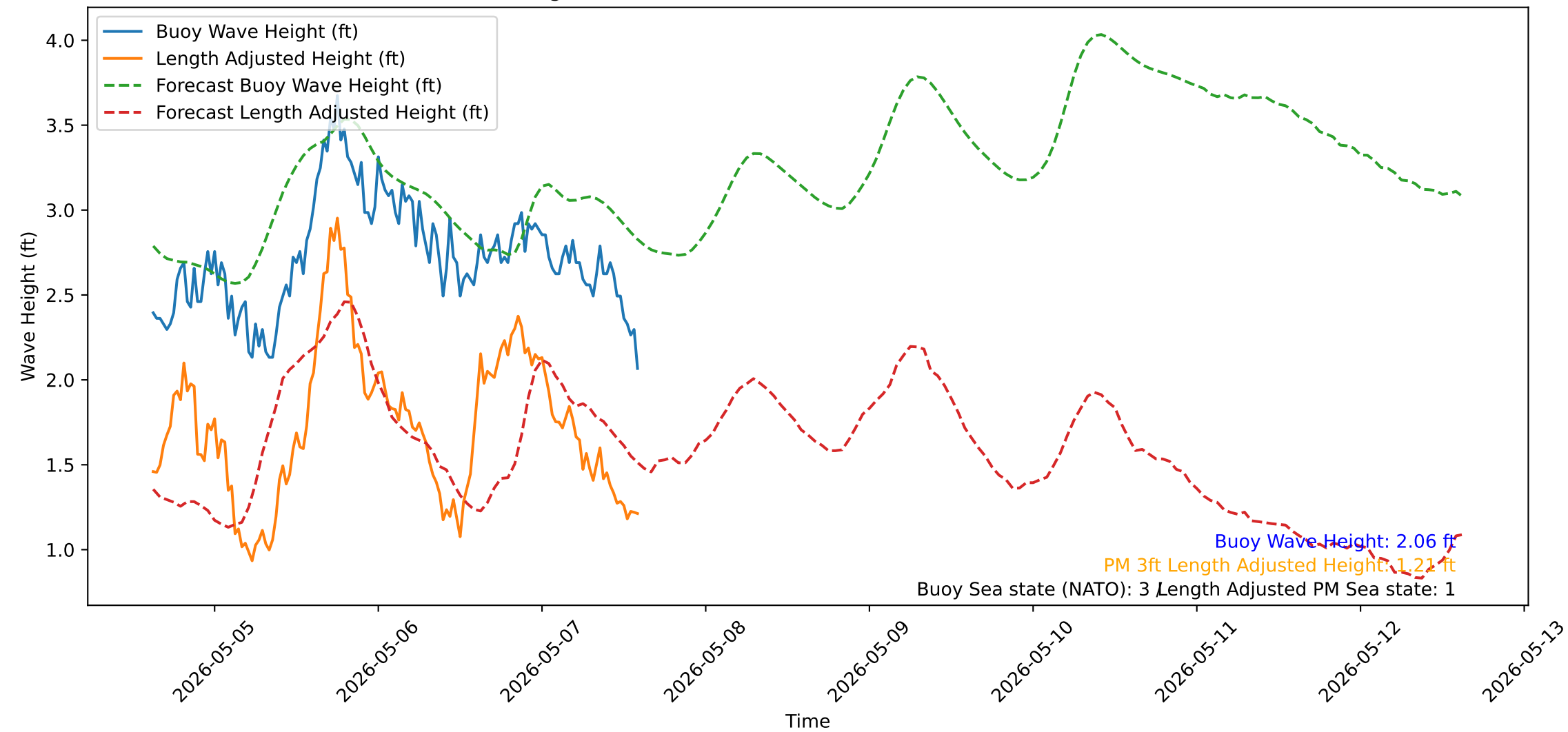
Wave Heights over Time for Green Beach at 2026-05-07 14:51:14
