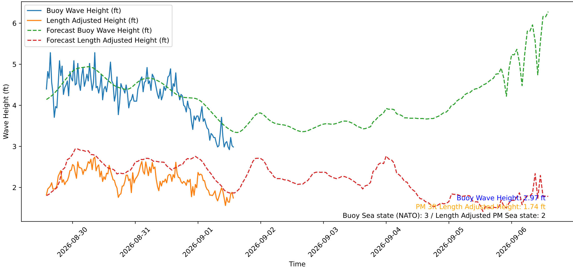
Wave Heights over Time for Oceanside Harbor at 2026-09-01 14:10:30
