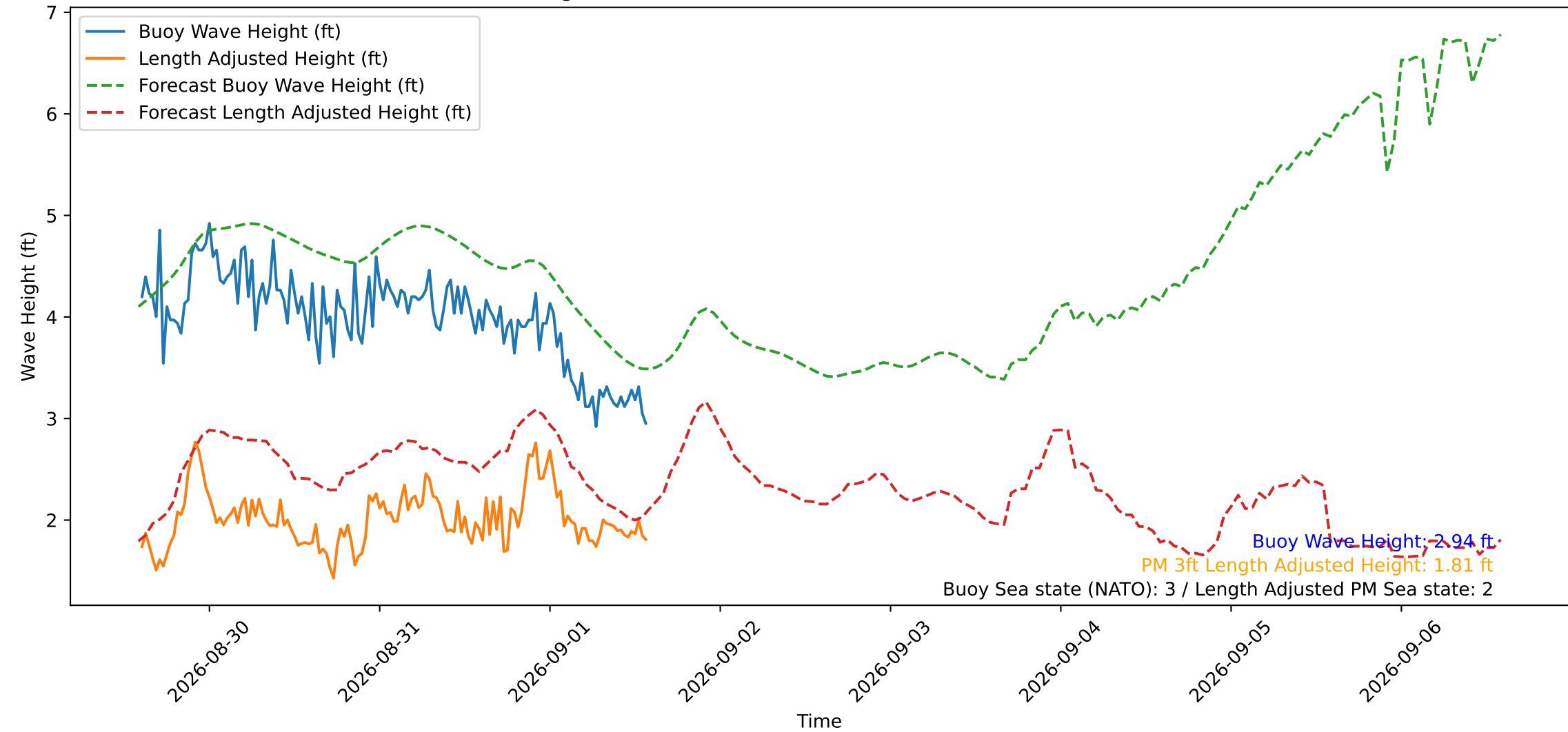
Wave Heights over Time for Green Beach at 2026-09-01 14:11:13
