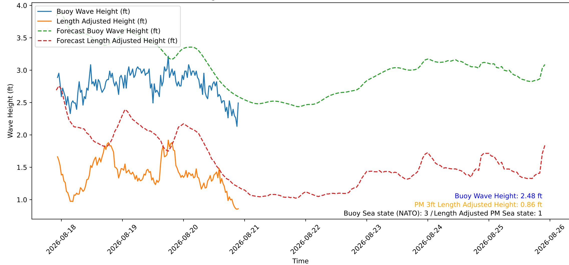
Wave Heights over Time for Red Beach at 2026-08-20 22:10:46
