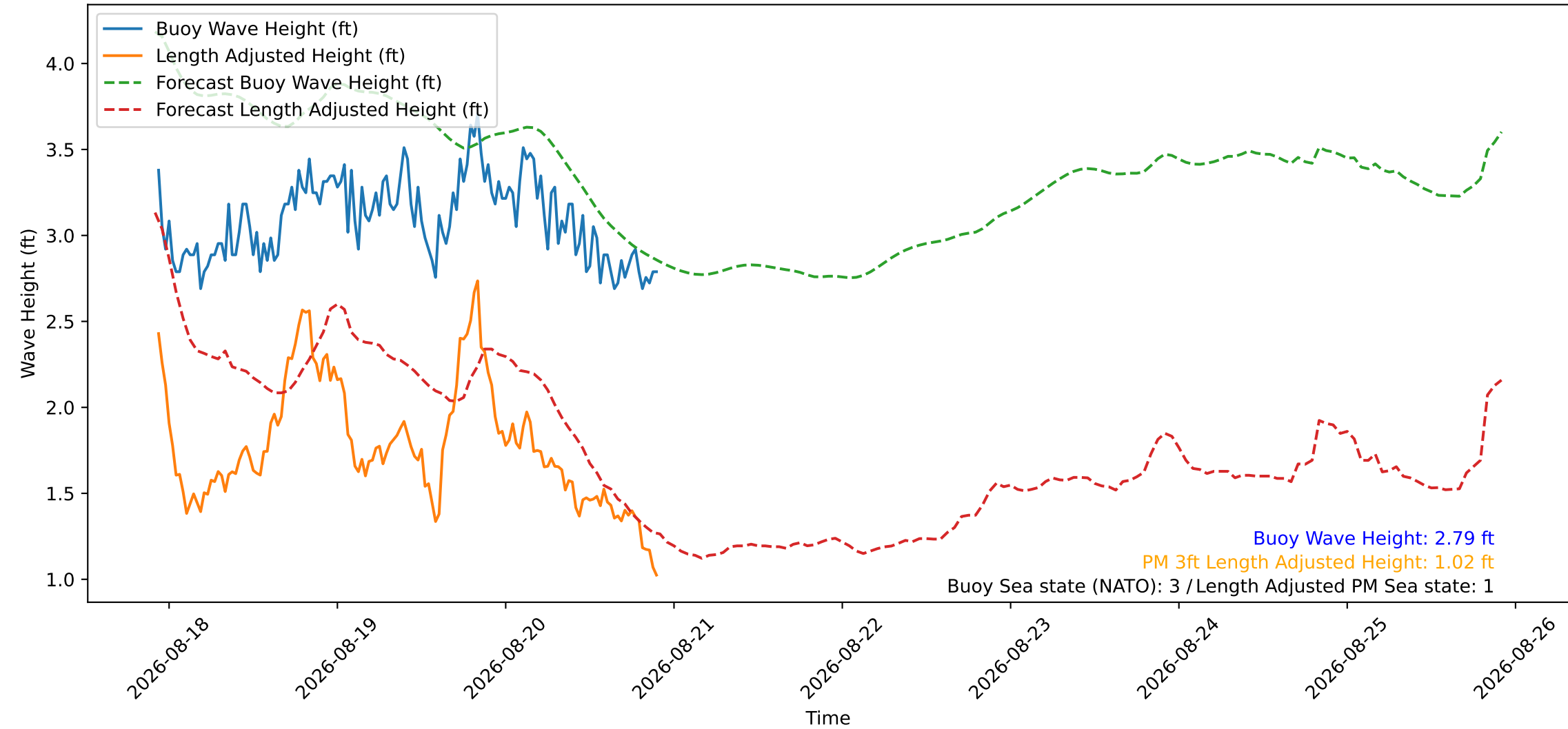
Wave Heights over Time for Green Beach at 2026-08-20 22:11:08
