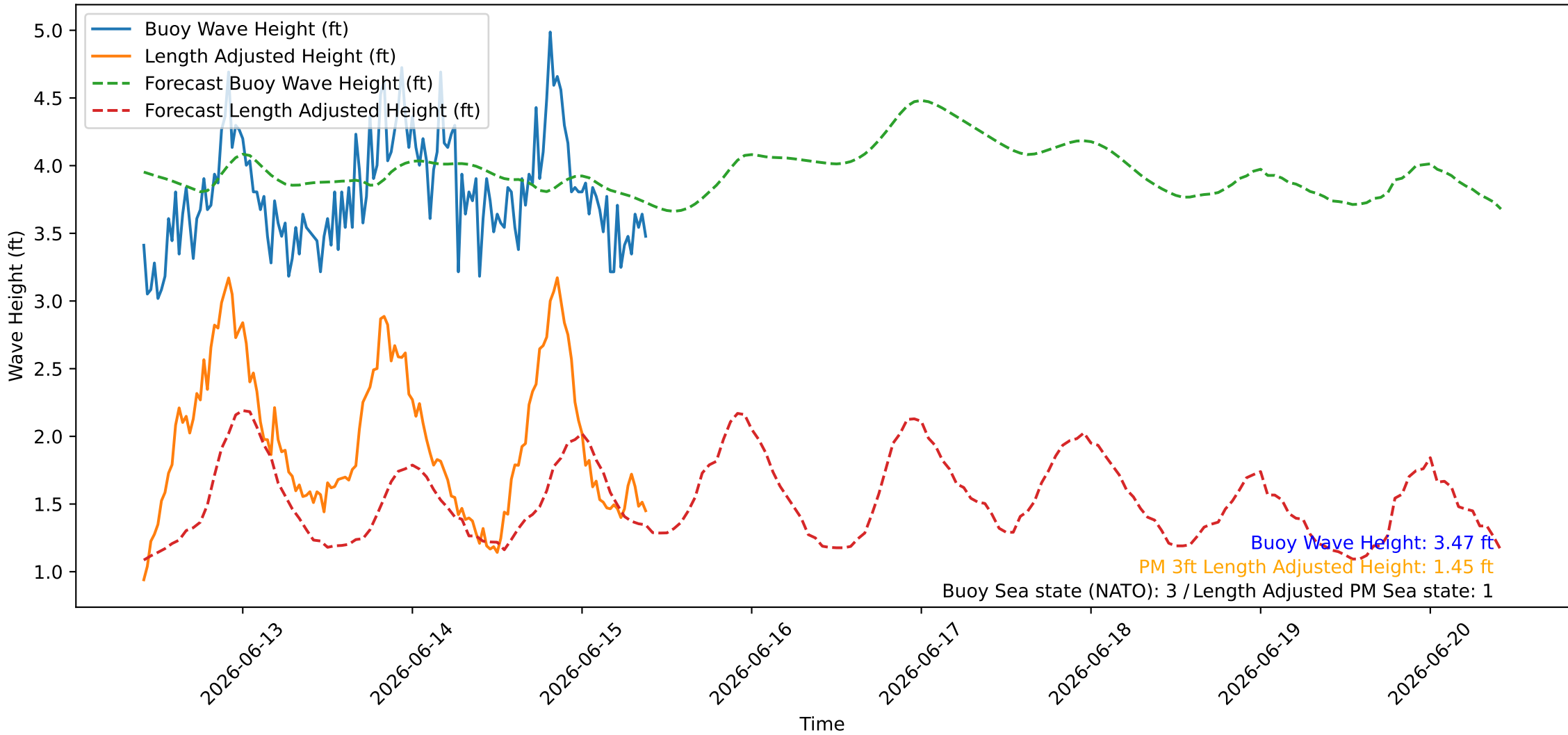
Wave Heights over Time for Oceanside Harbor at 2026-06-15 09:50:26
