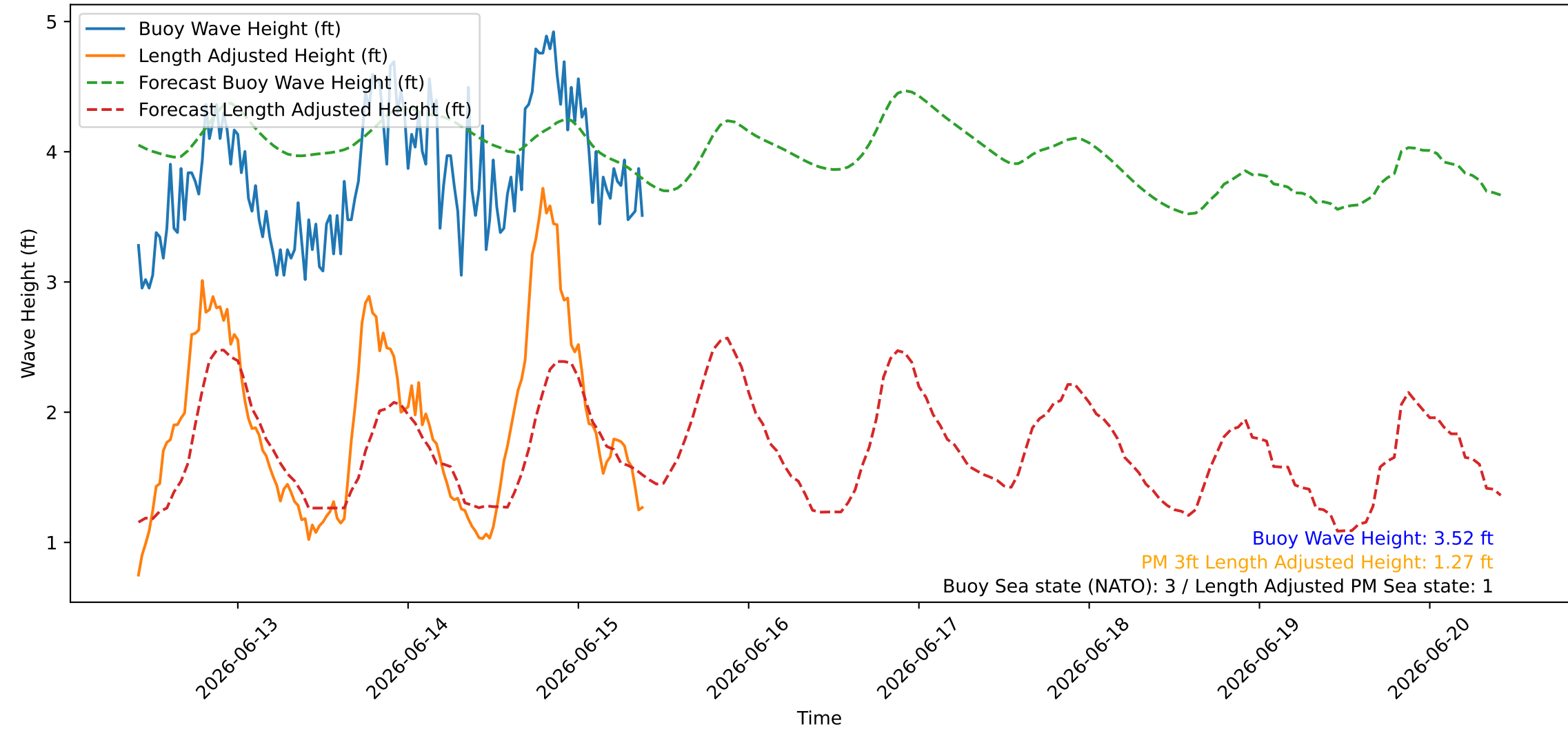
Wave Heights over Time for Green Beach at 2026-06-15 09:51:09
