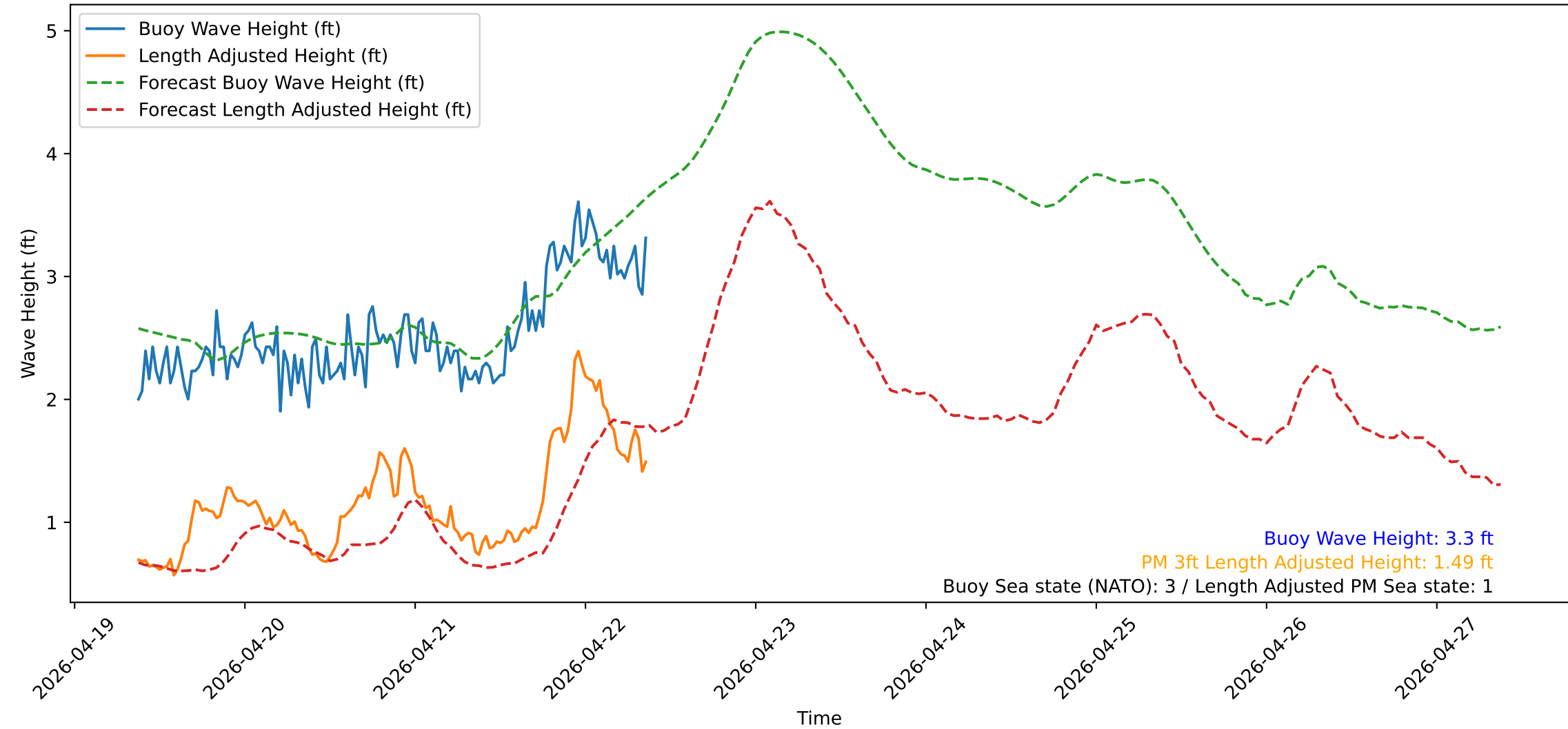
Wave Heights over Time for Oceanside Harbor at 2026-04-22 09:10:31
