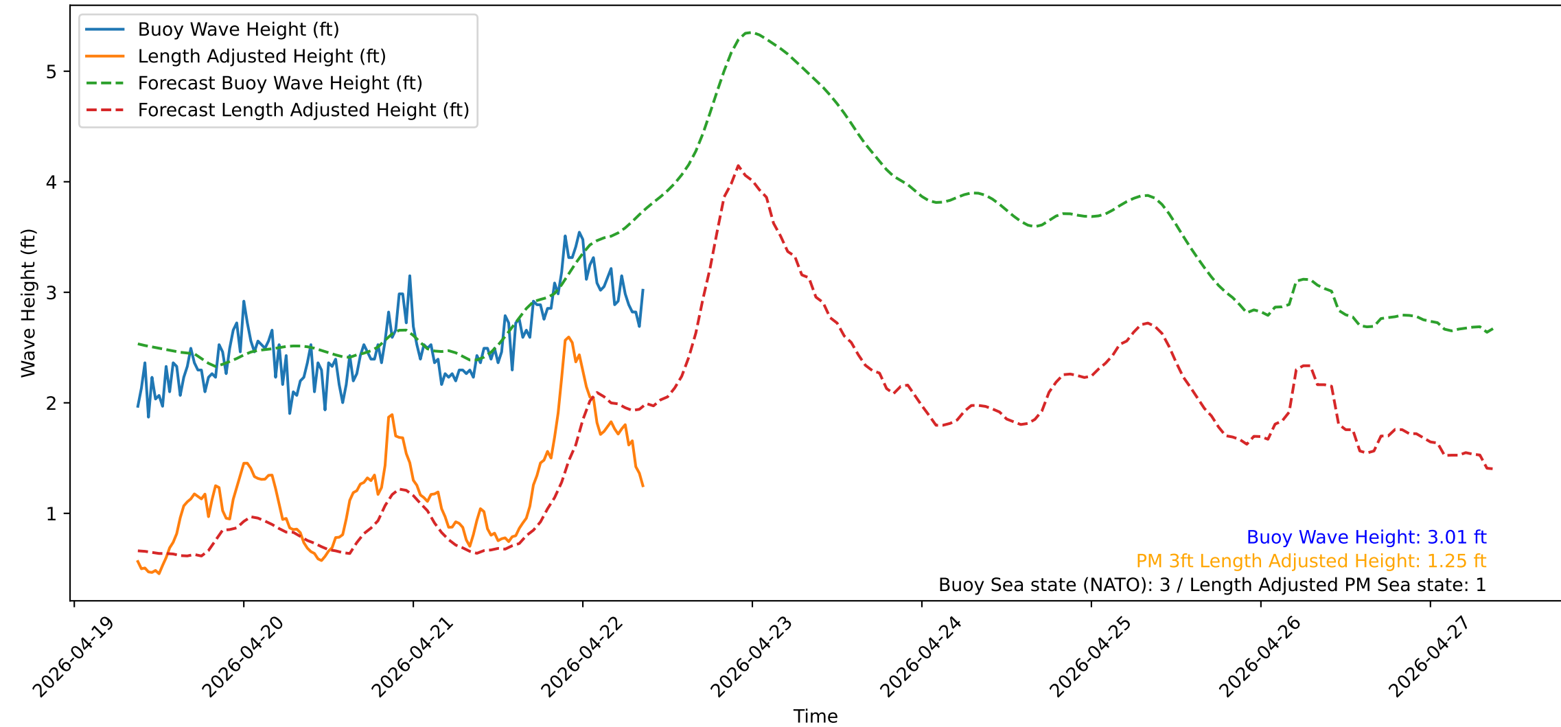
Wave Heights over Time for Green Beach at 2026-04-22 09:11:12
