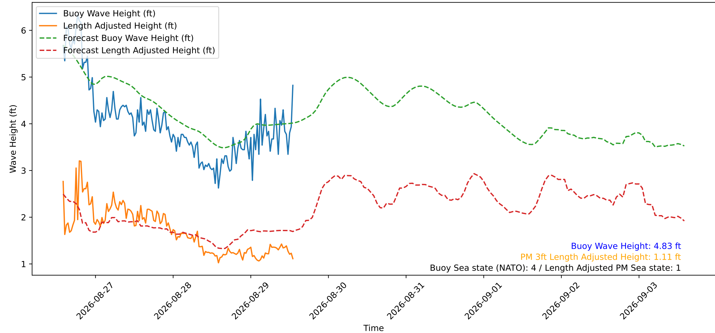
Wave Heights over Time for Green Beach at 2026-08-29 13:41:12
