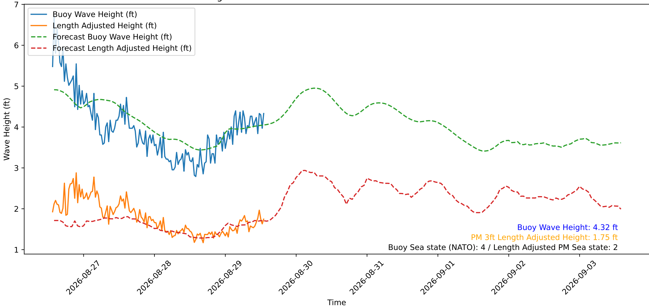
Wave Heights over Time for Oceanside Harbor at 2026-08-29 13:40:30
