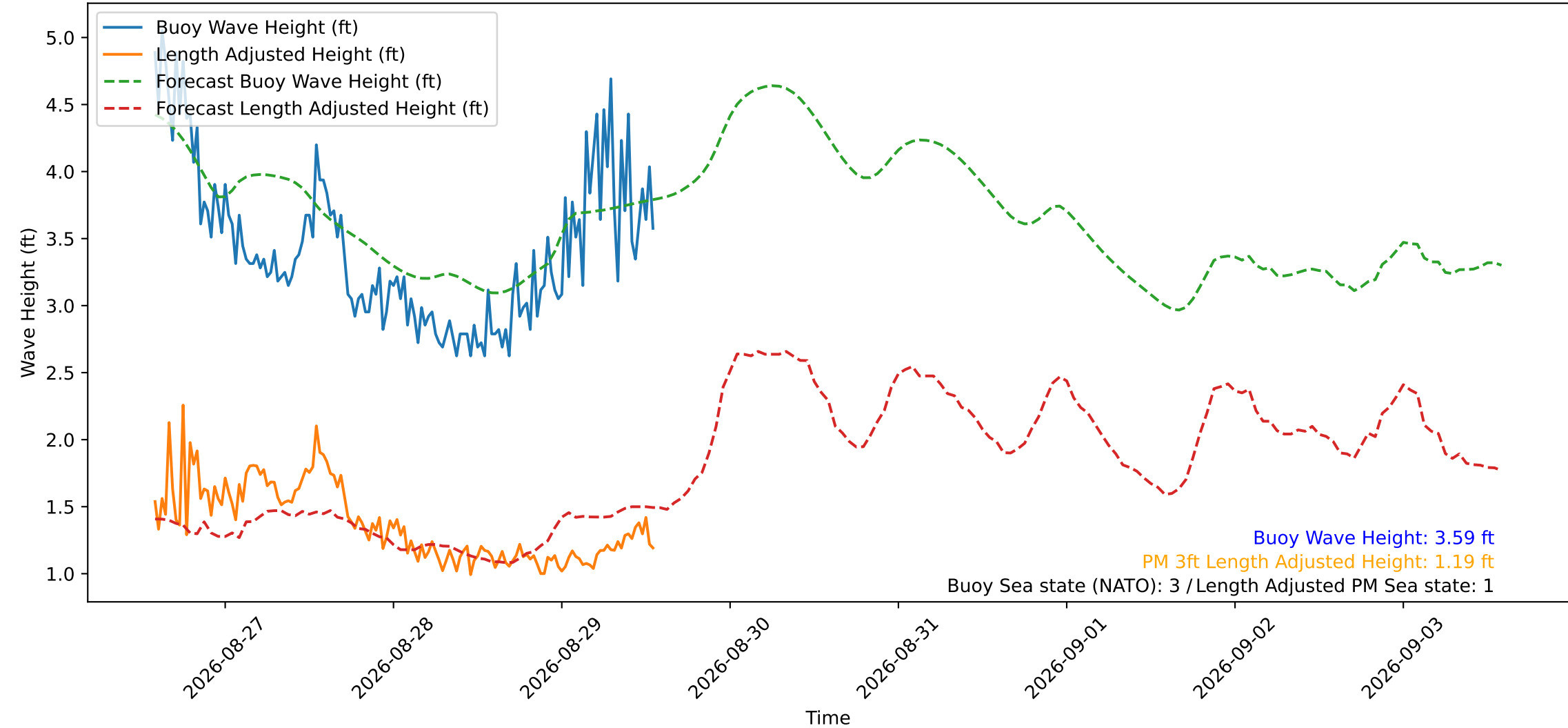
Wave Heights over Time for Red Beach at 2026-08-29 13:40:50
