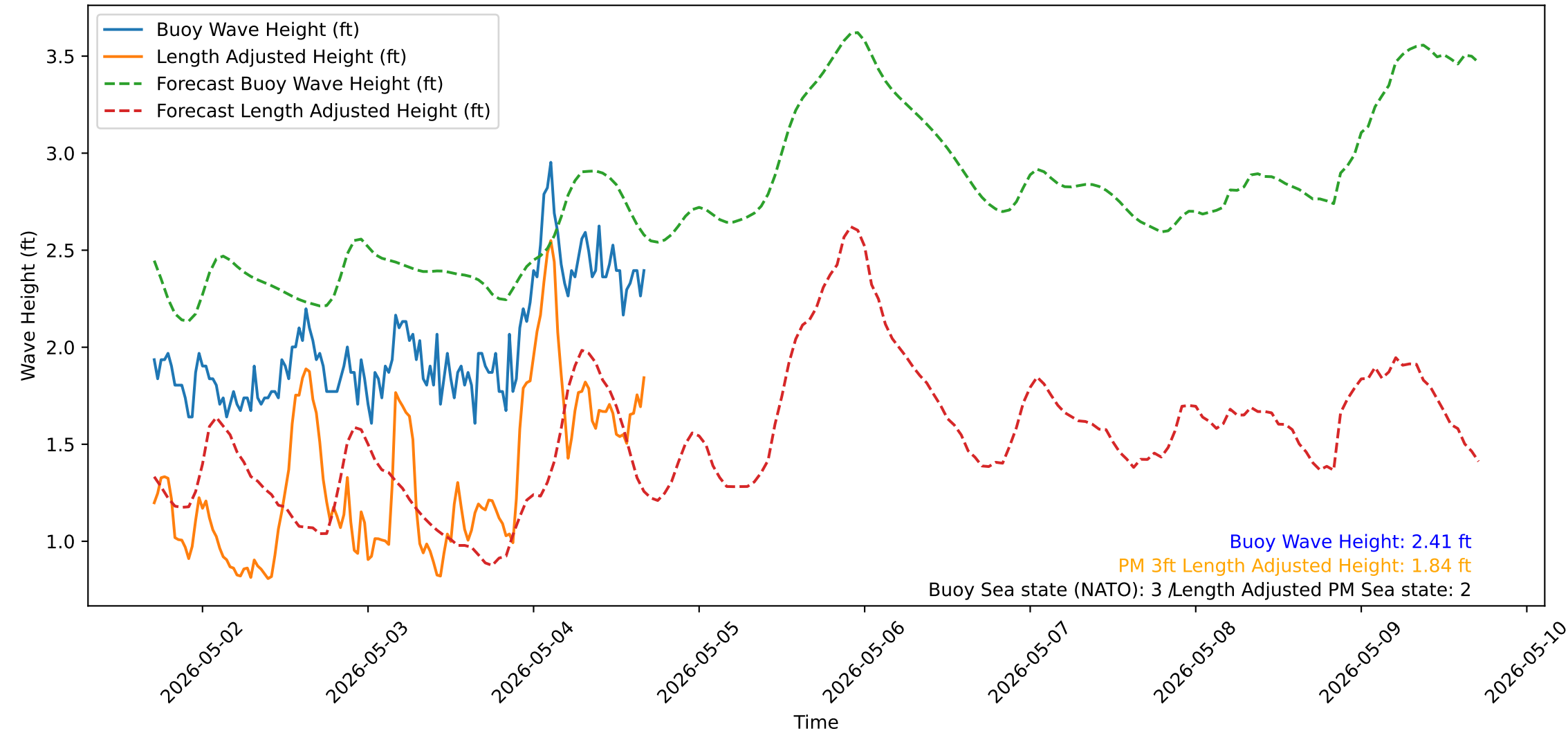
Wave Heights over Time for Red Beach at 2026-05-04 16:50:52
