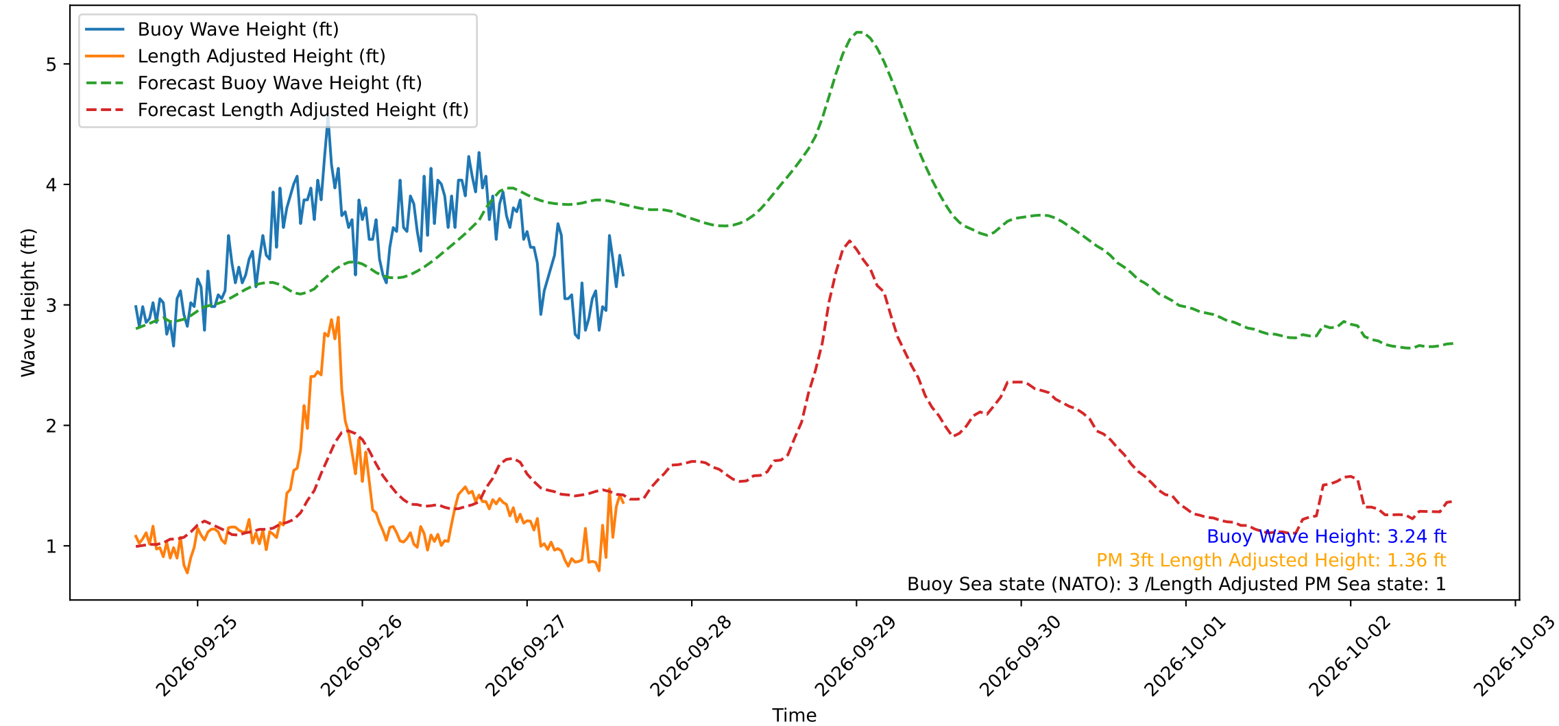
Wave Heights over Time for Green Beach at 2026-09-27 14:41:11
