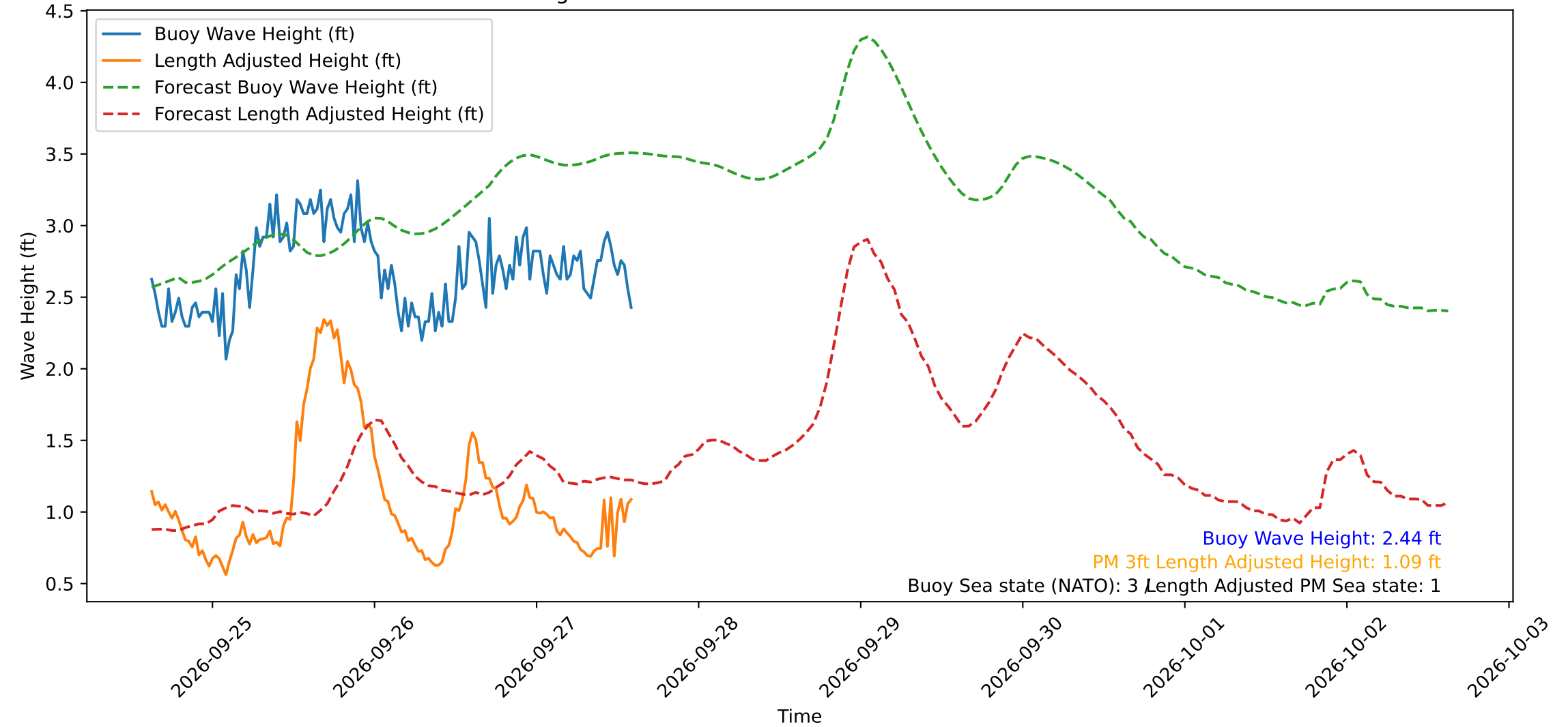
Wave Heights over Time for Red Beach at 2026-09-27 14:40:49
