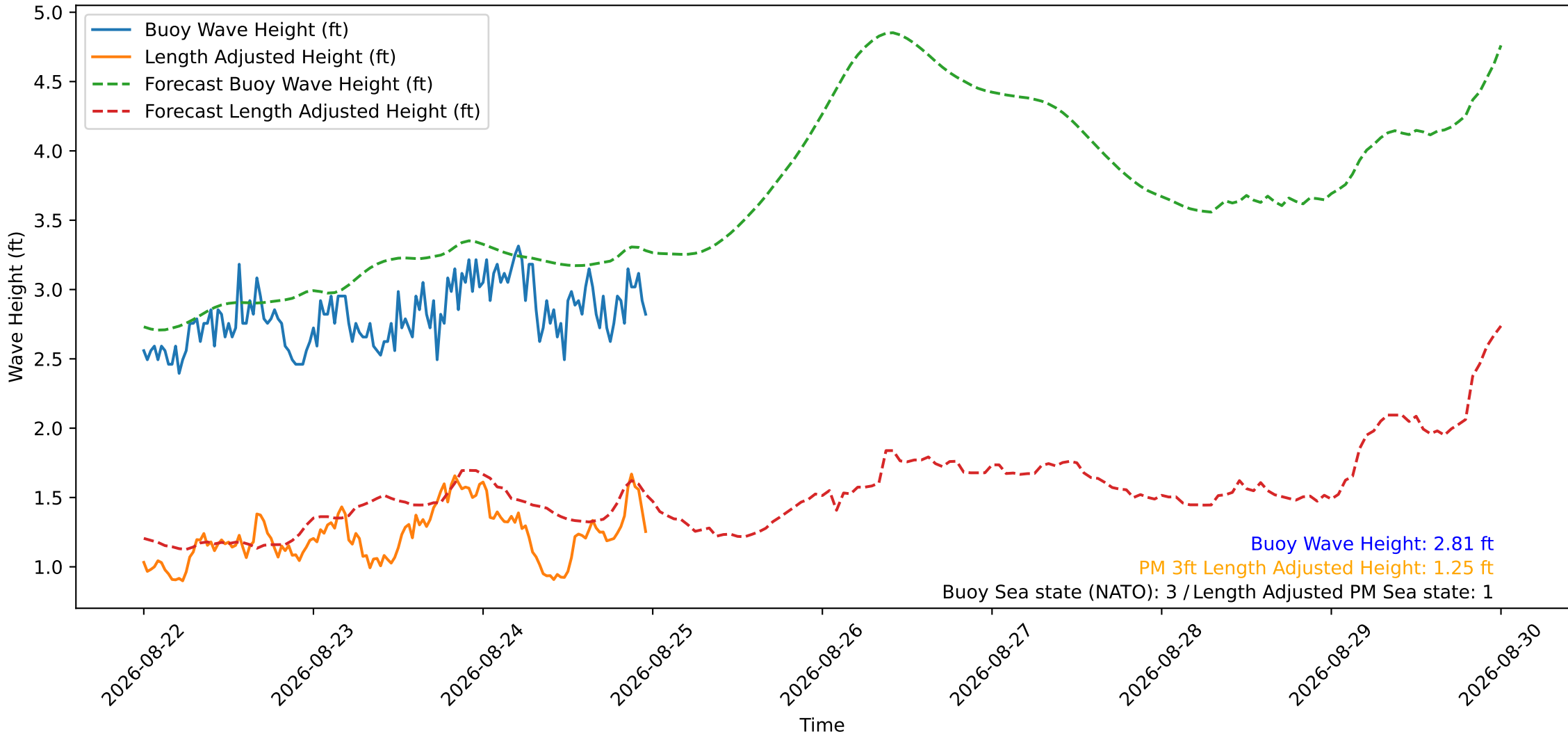
Wave Heights over Time for Green Beach at 2026-08-24 23:51:14
