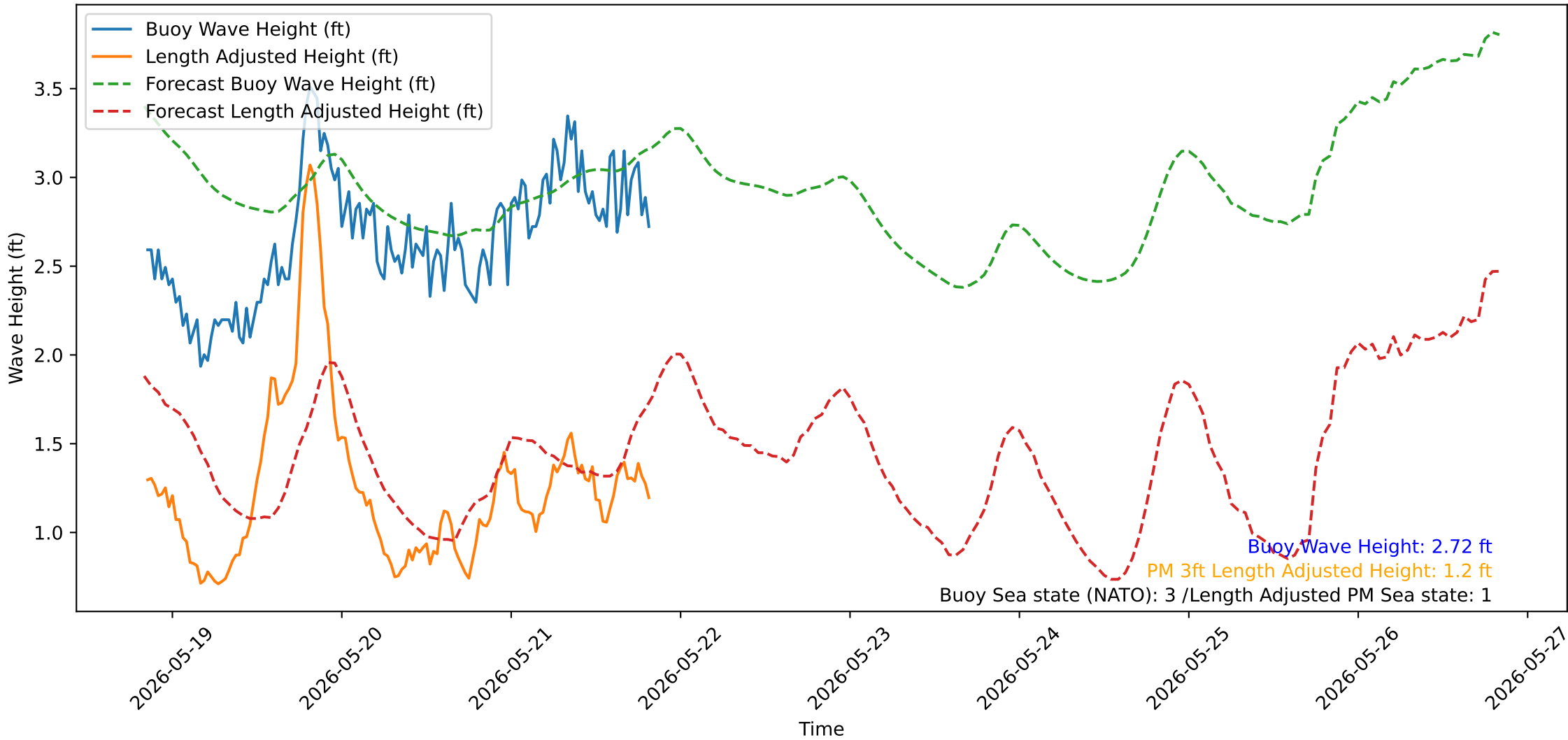
Wave Heights over Time for Red Beach at 2026-05-21 20:20:51
