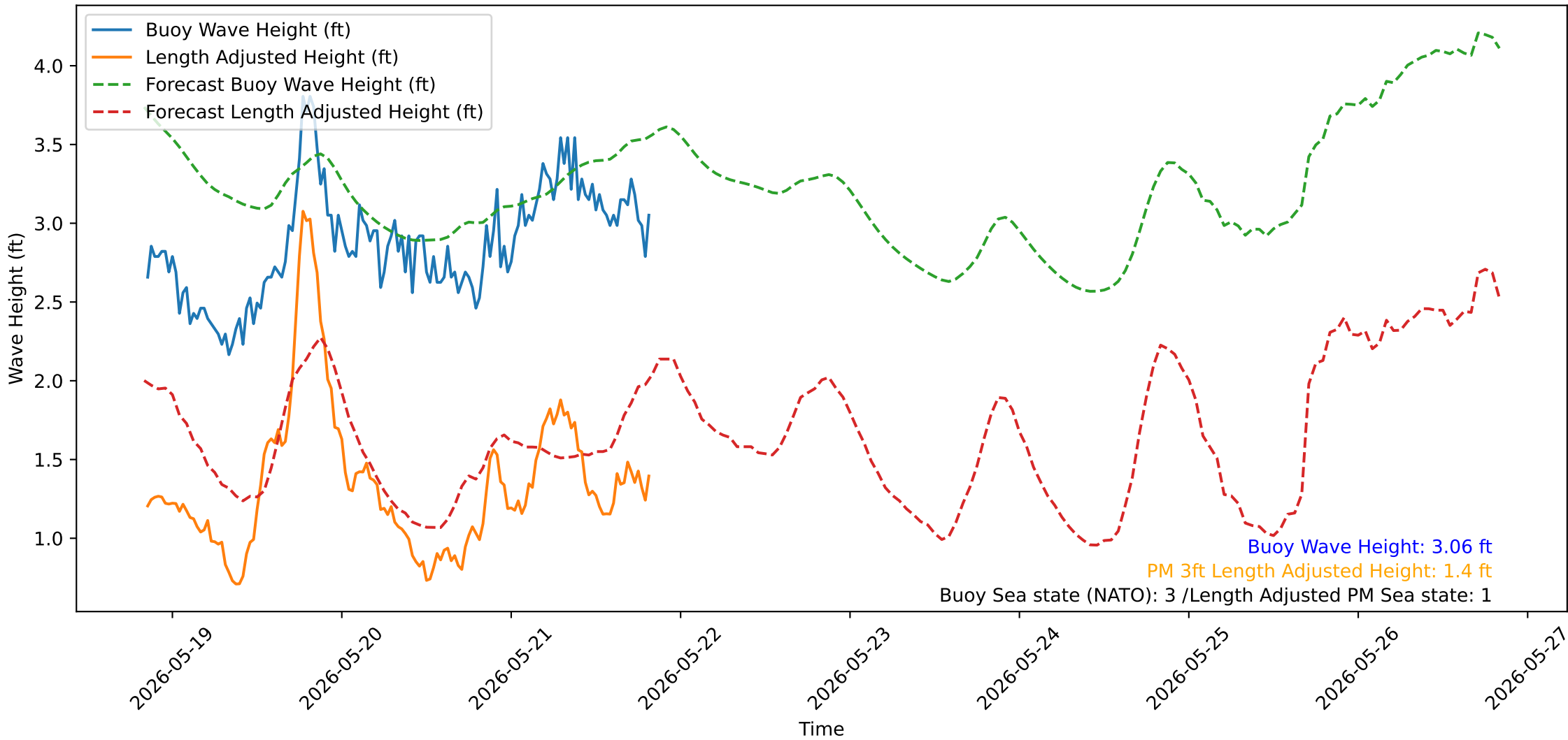
Wave Heights over Time for Green Beach at 2026-05-21 20:21:14
