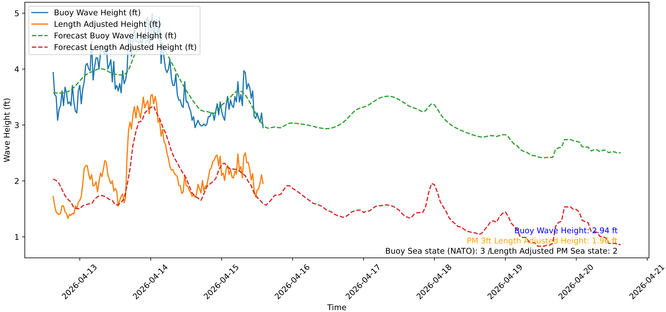
Wave Heights over Time for Green Beach at 2026-04-15 15:01:14
