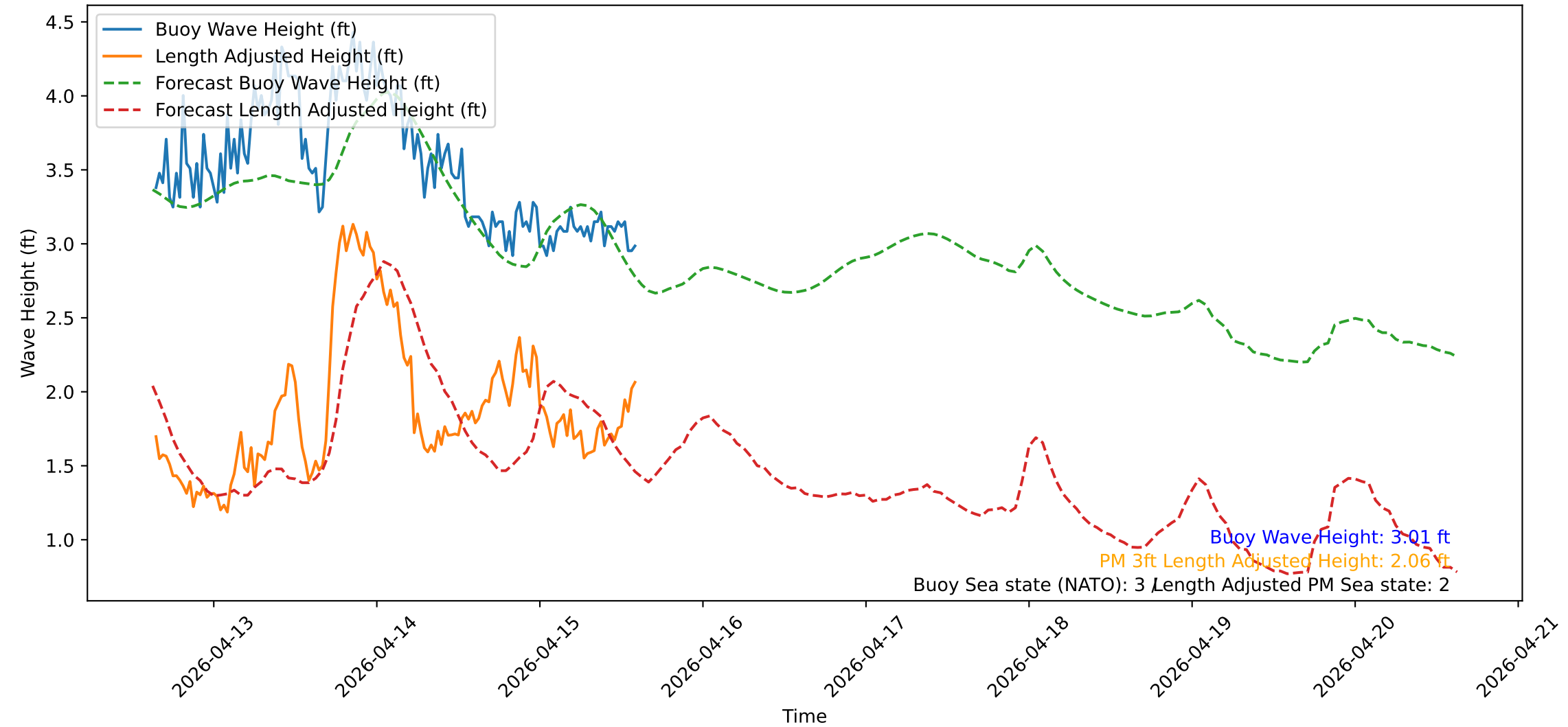
Wave Heights over Time for Red Beach at 2026-04-15 15:00:51
