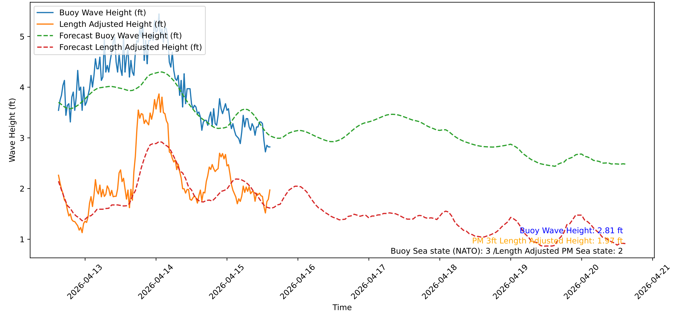
Wave Heights over Time for Oceanside Harbor at 2026-04-15 15:00:32
