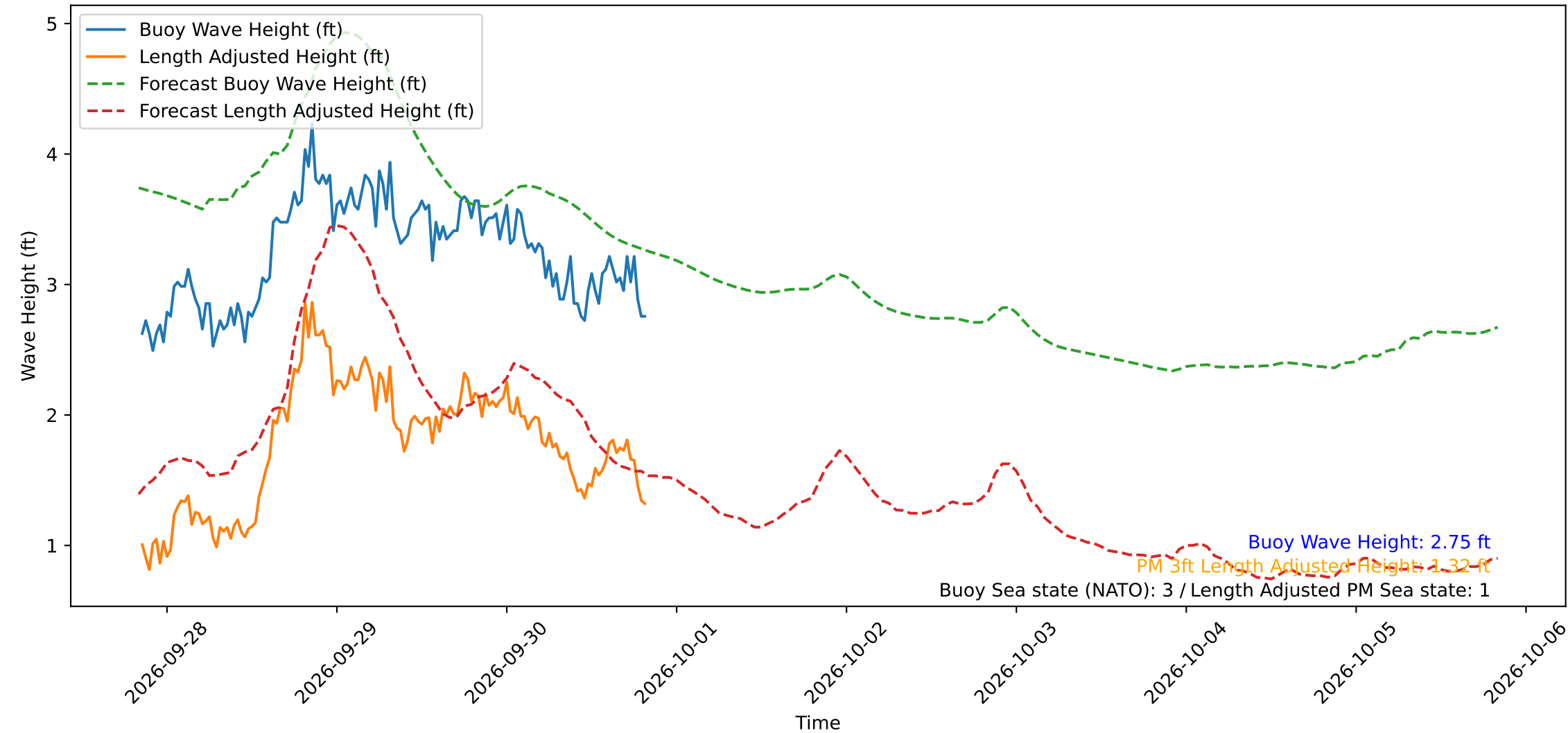
Wave Heights over Time for Oceanside Harbor at 2026-09-30 20:20:30
