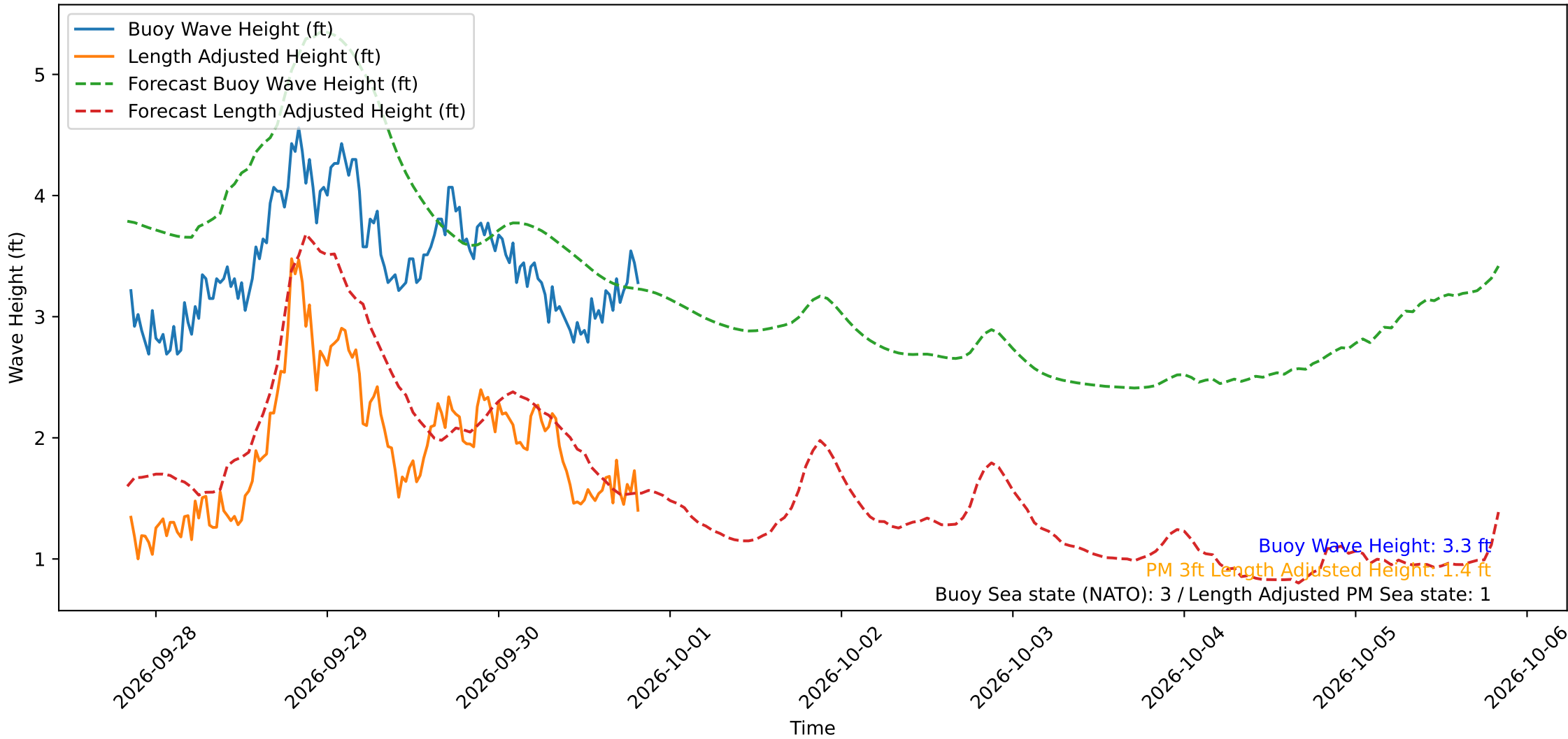
Wave Heights over Time for Green Beach at 2026-09-30 20:21:15
