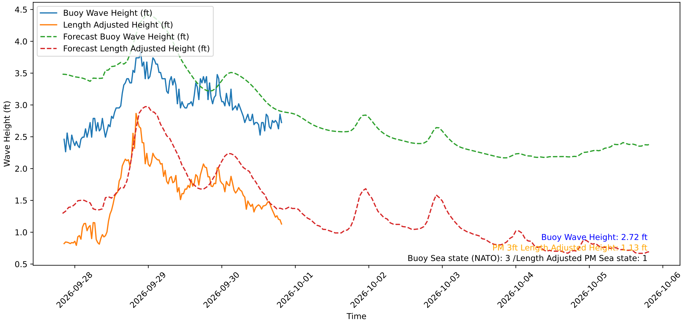
Wave Heights over Time for Red Beach at 2026-09-30 20:20:51
