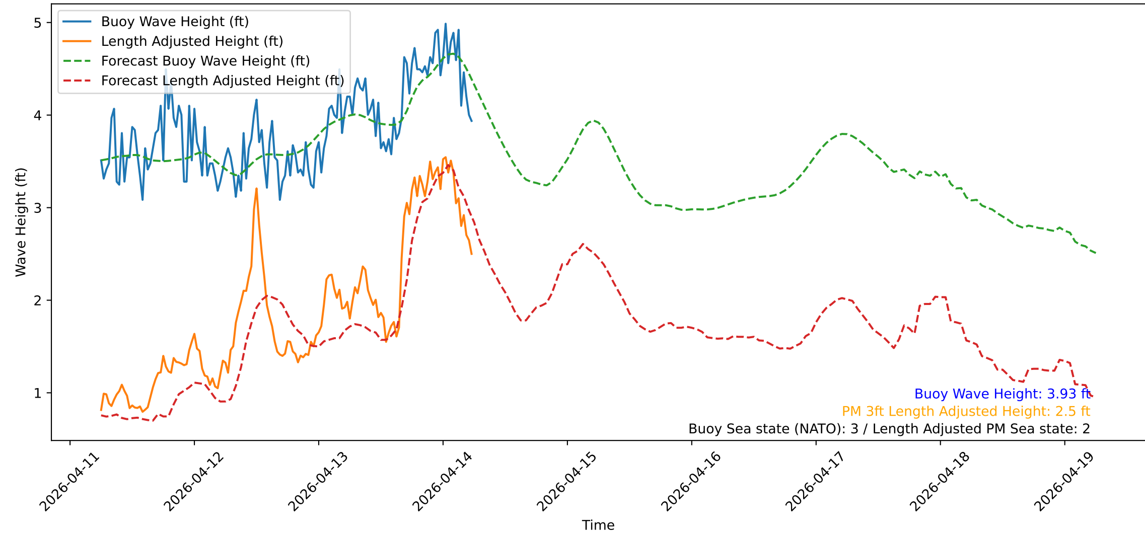
Wave Heights over Time for Green Beach at 2026-04-14 06:11:13
