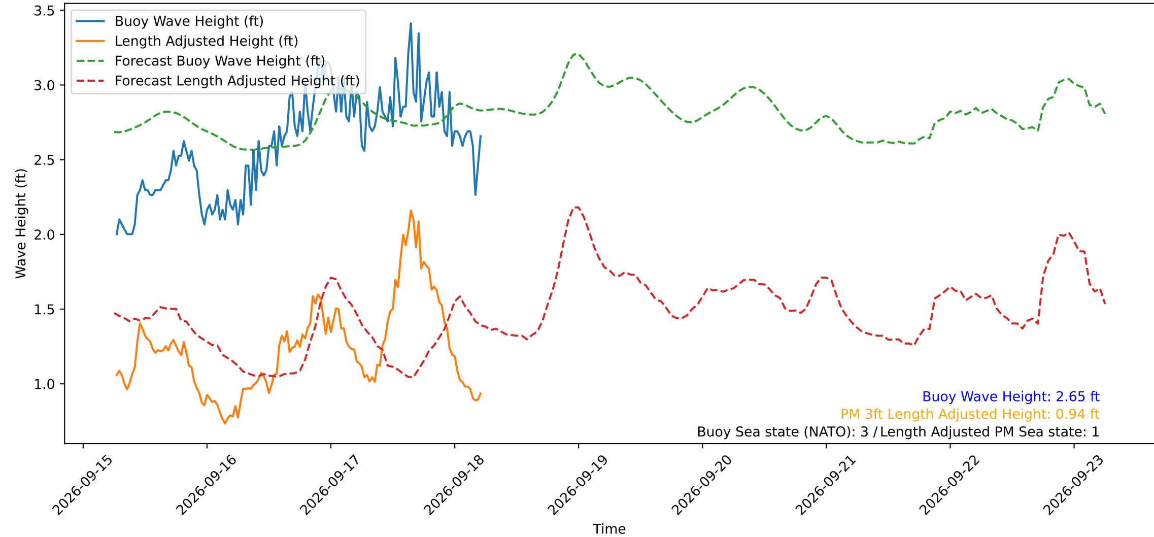
Wave Heights over Time for Red Beach at 2026-09-18 06:00:49
