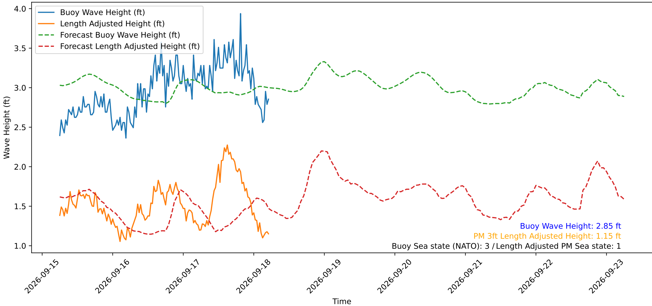
Wave Heights over Time for Oceanside Harbor at 2026-09-18 06:00:30
