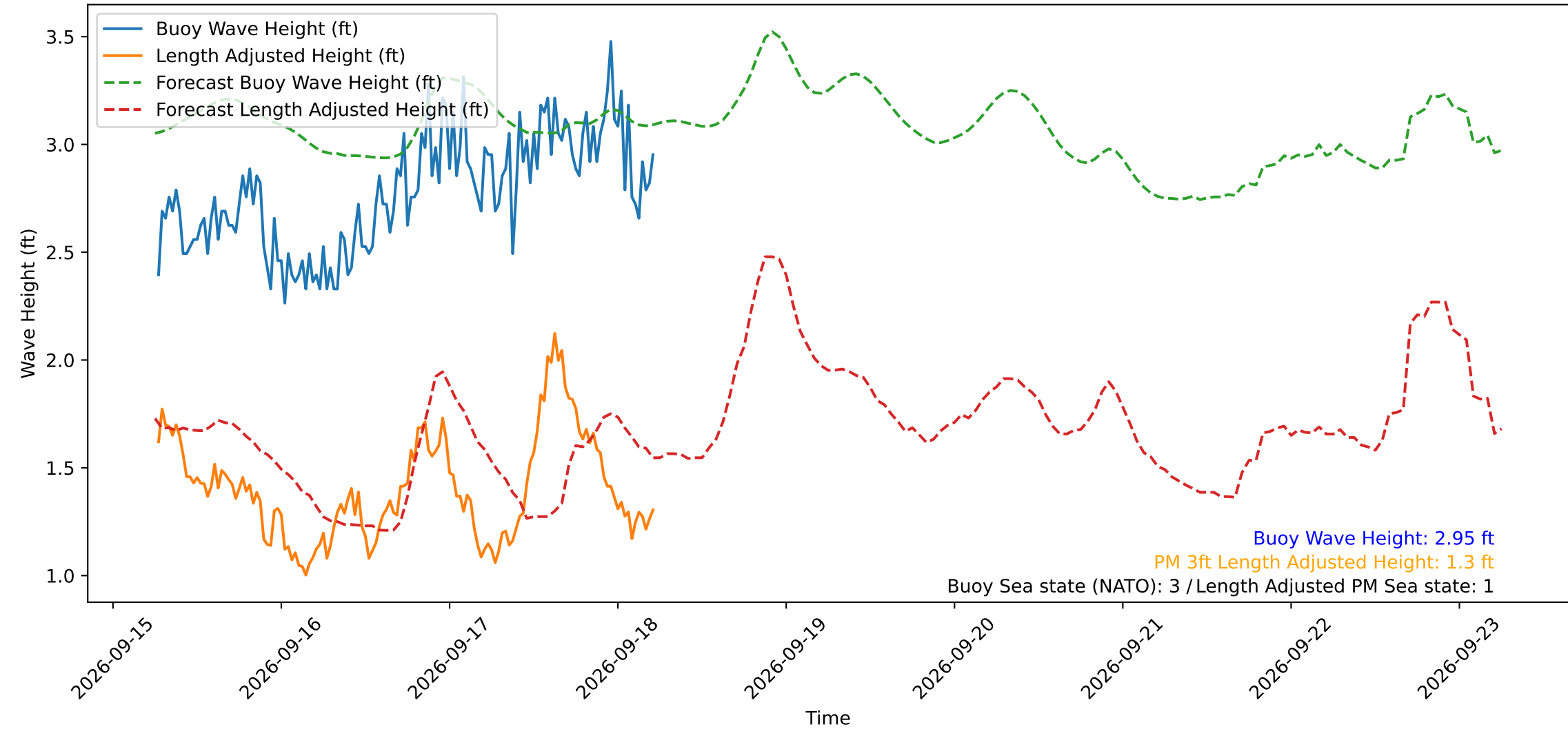
Wave Heights over Time for Green Beach at 2026-09-18 06:01:11
