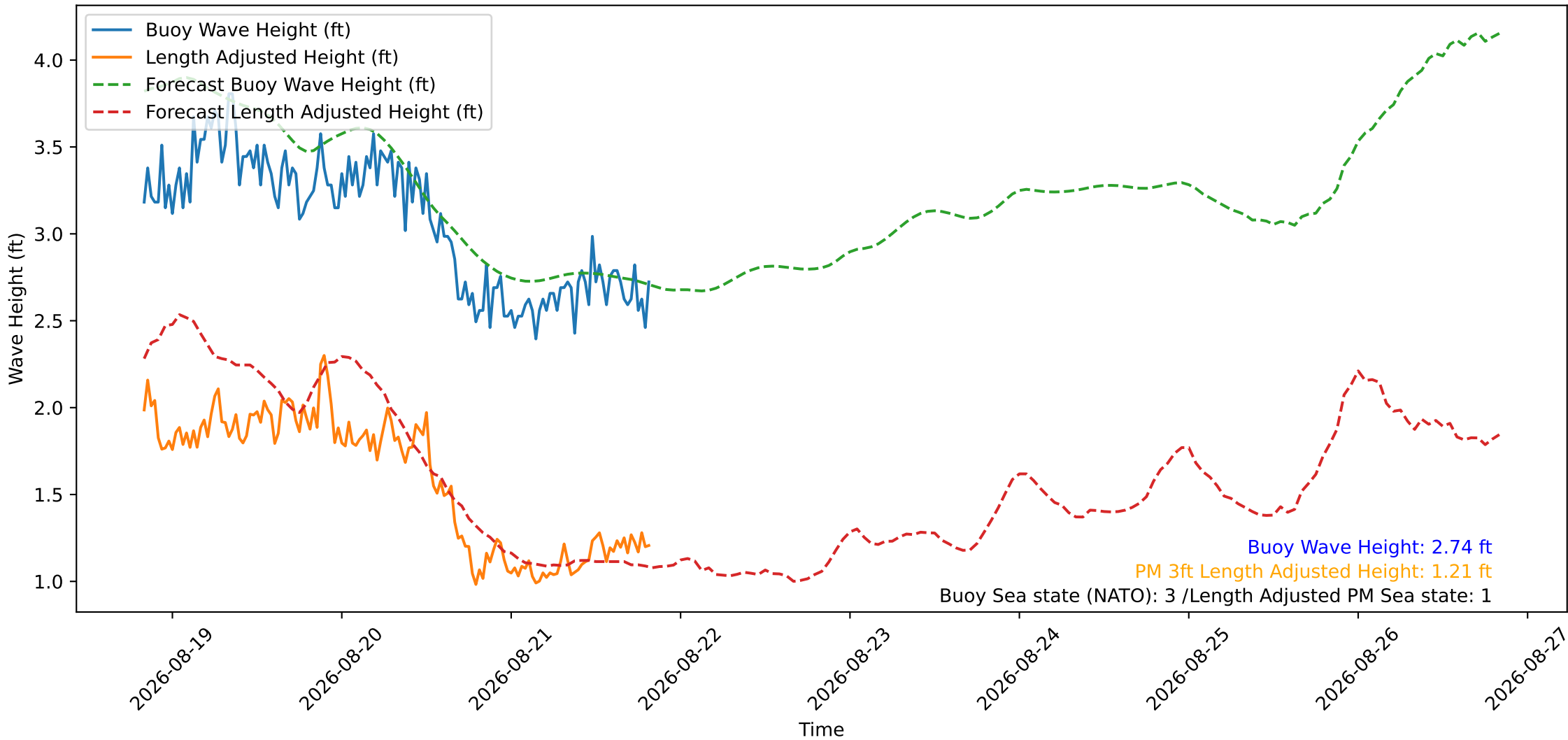
Wave Heights over Time for Oceanside Harbor at 2026-08-21 20:10:26
