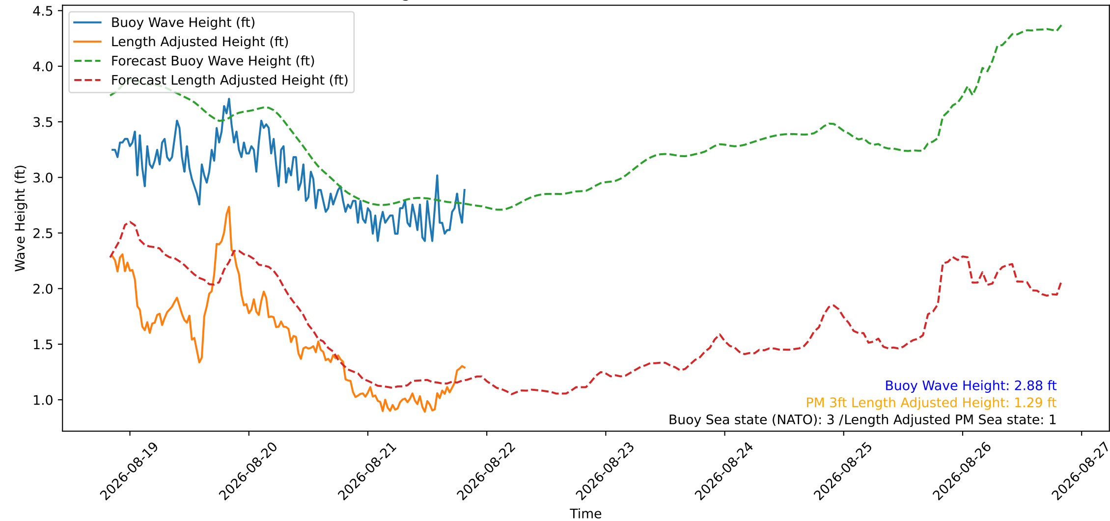
Wave Heights over Time for Green Beach at 2026-08-21 20:11:08
