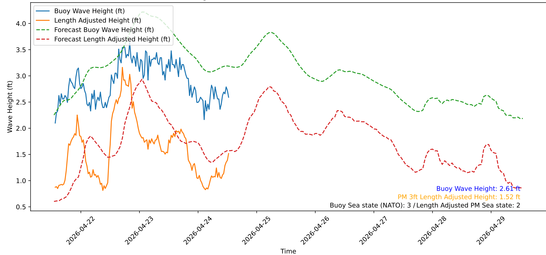
Wave Heights over Time for Red Beach at 2026-04-24 13:10:50
