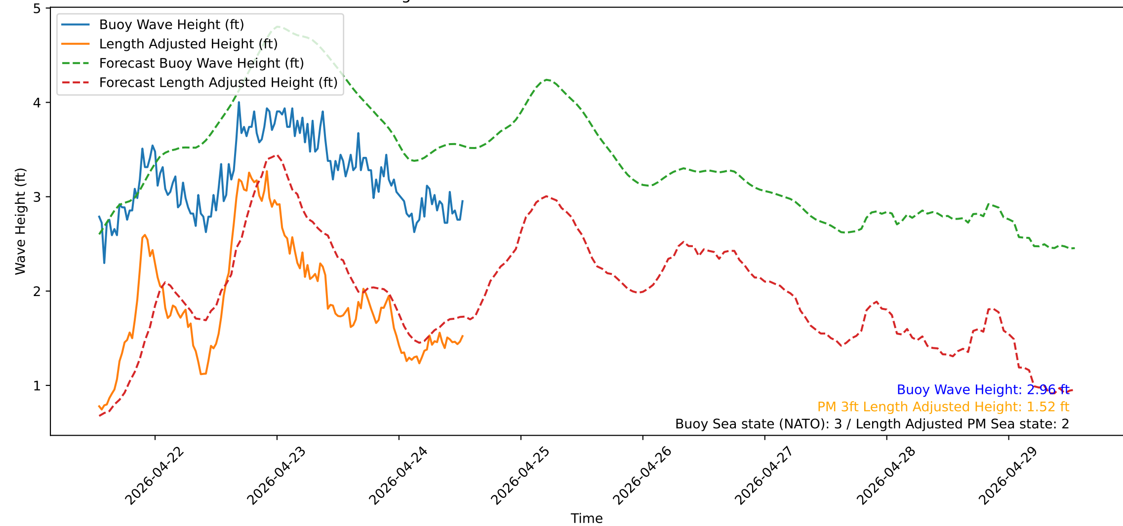
Wave Heights over Time for Green Beach at 2026-04-24 13:11:12
