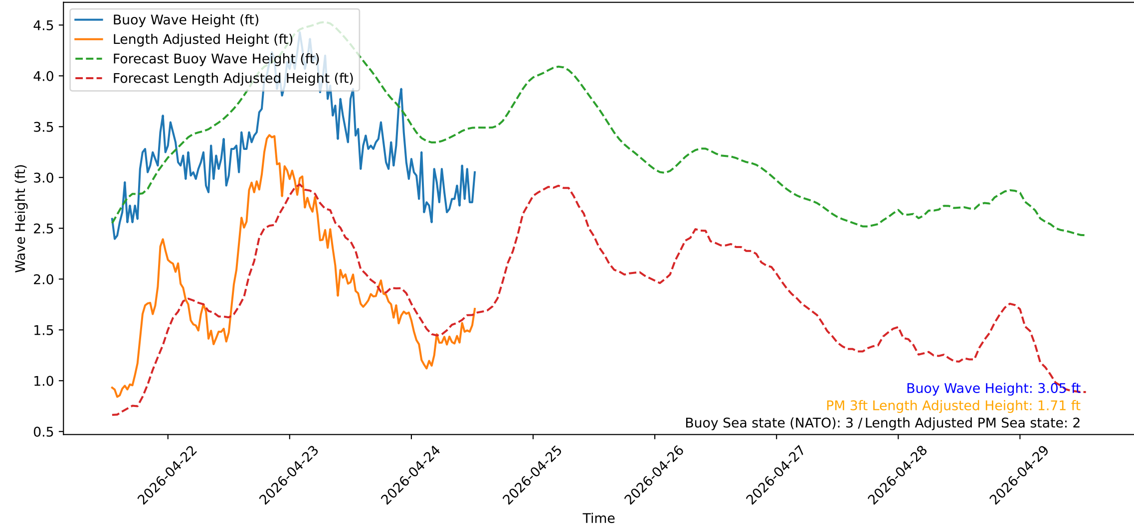
Wave Heights over Time for Oceanside Harbor at 2026-04-24 13:10:31
