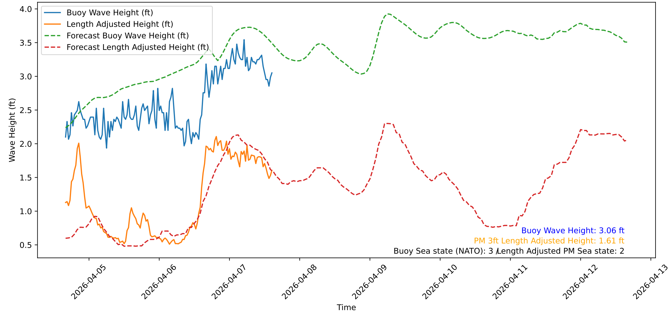
Wave Heights over Time for Red Beach at 2026-04-07 15:30:48
