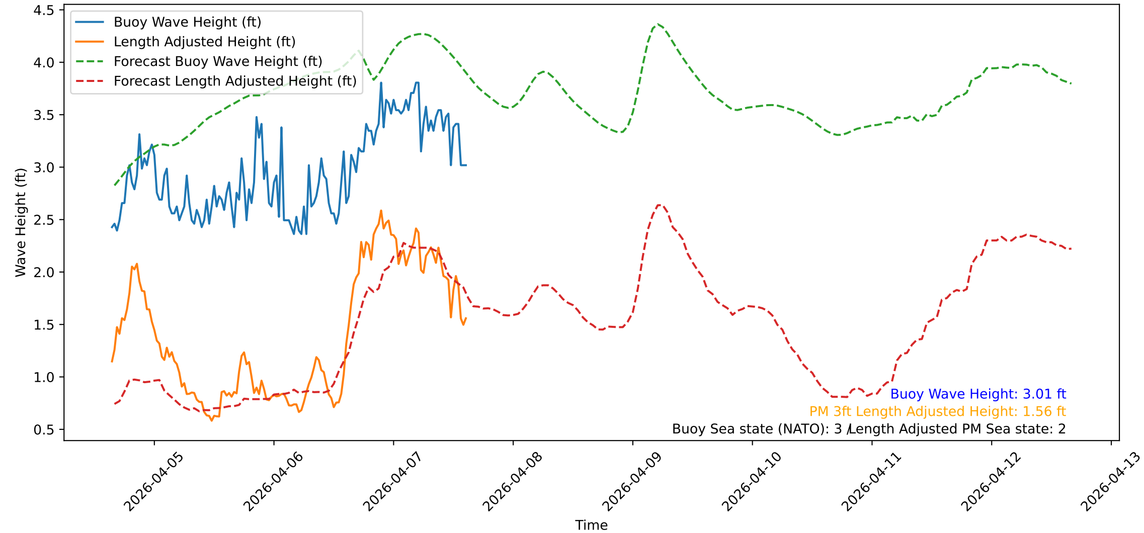
Wave Heights over Time for Green Beach at 2026-04-07 15:31:11
